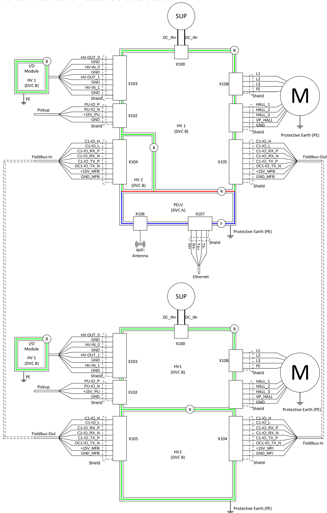
Figure 4-2 Connection diagrams
