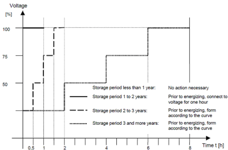
Figure 6-1 Capacitor reforming
