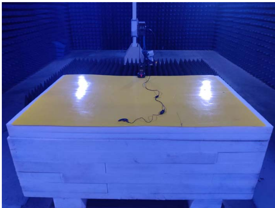
Photo of Radiated Emission Measurement (Above 1G) Test mode 1
