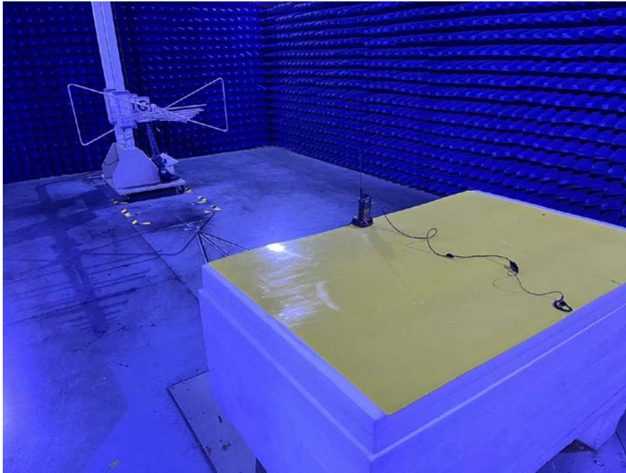
Photo of Radiated Emission Measurement (Below 1G) Test mode 1
