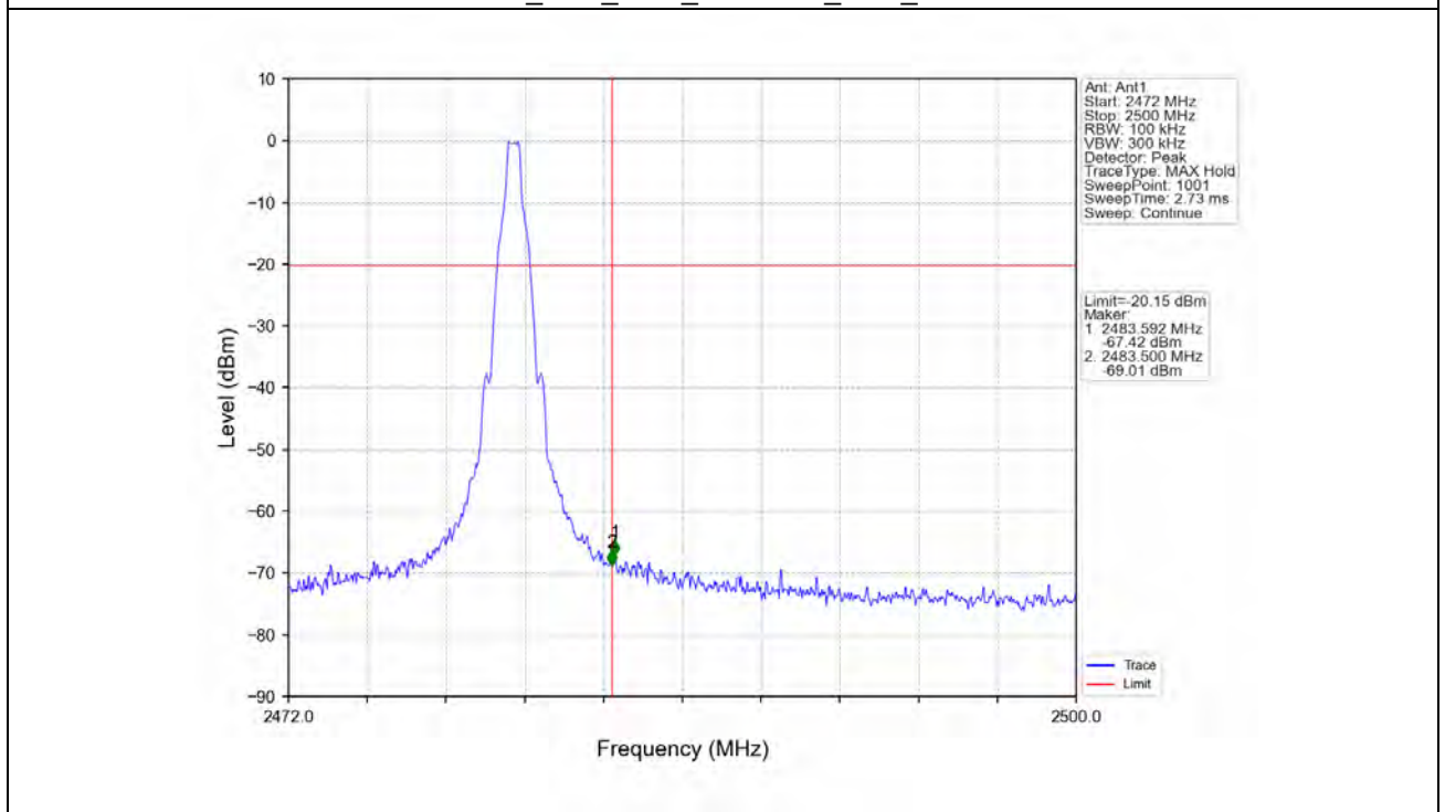
GFSK_DH5_HCH_2480MHz_Ant1_NTNV
