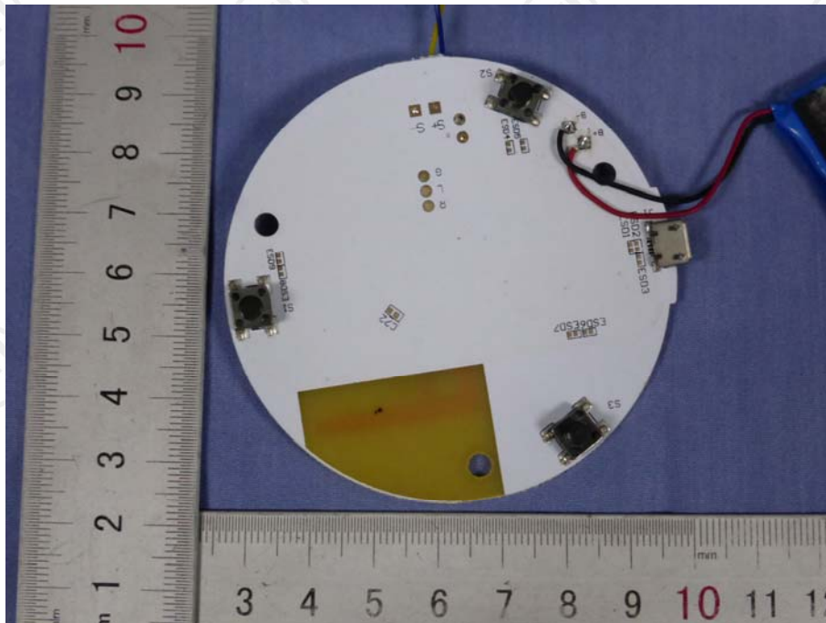
Fig.3- PCB View
