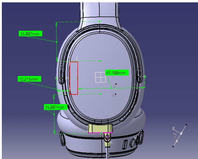
Antenna location
