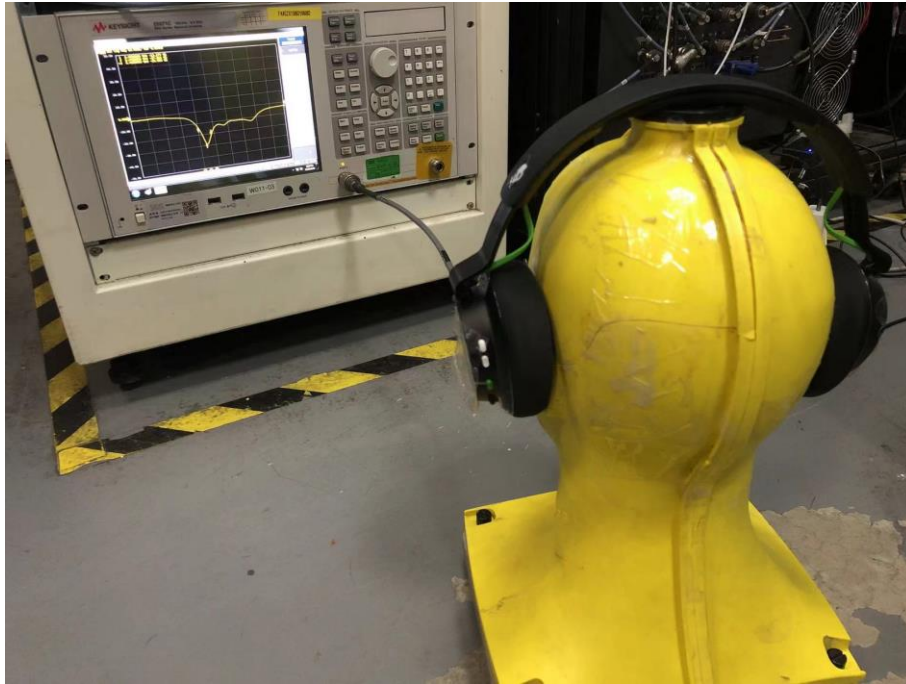
BH-#1 Impedance Setup
