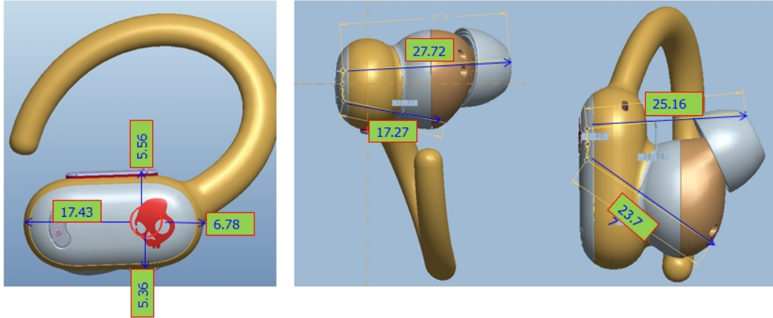
Antenna location
