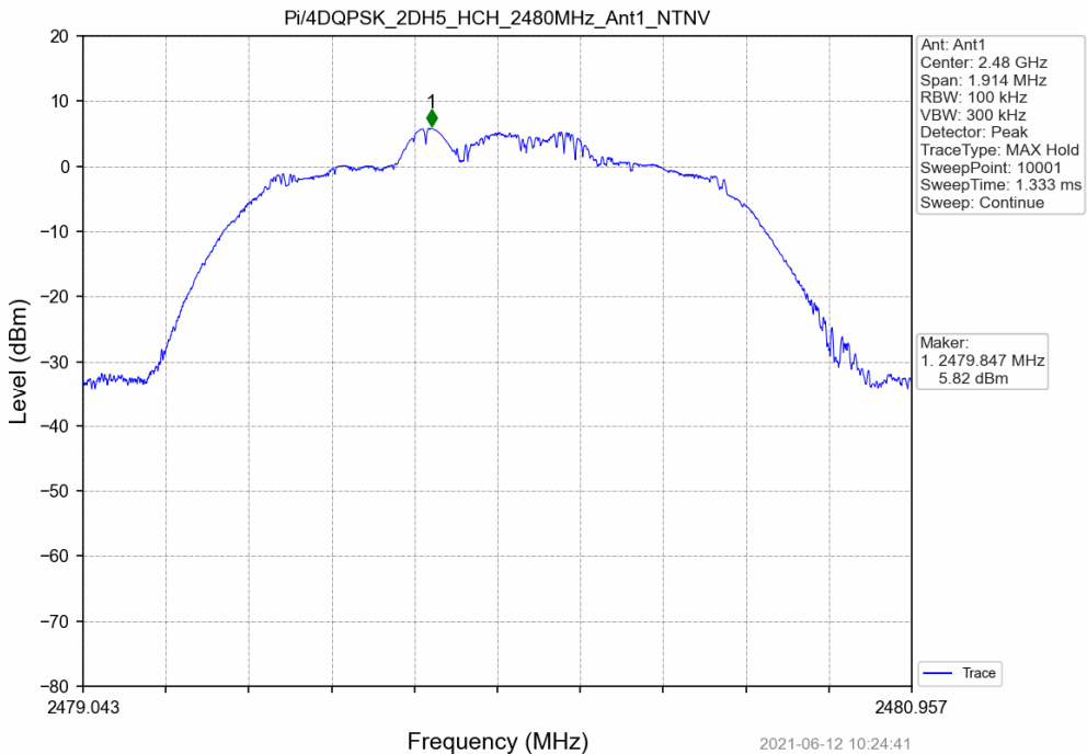
Pi/4DQPSK_2DH5_HCH_2480MHz_Ant1_NTNV
