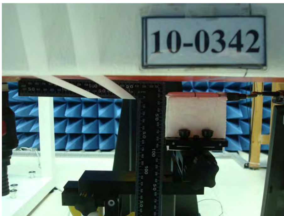
Figure 4. Horizontal Down, EUT to Phantom 15mm space with USB Cable _ LCD Open 90 degree
