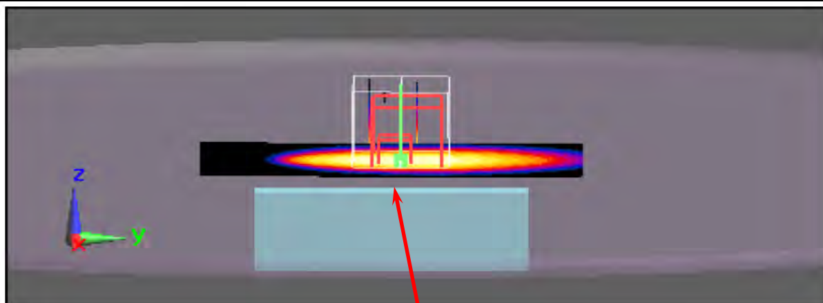
Figure 6. Vertical Back, EUT to Phantom 5mm space with USB Cable _ LCD Open 90 degree
