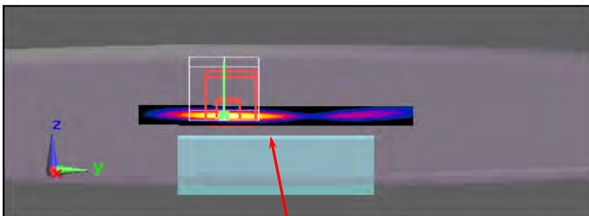
Figure 5. Vertical Front, EUT to Phantom 5mm space _ LCD Open90 degree
