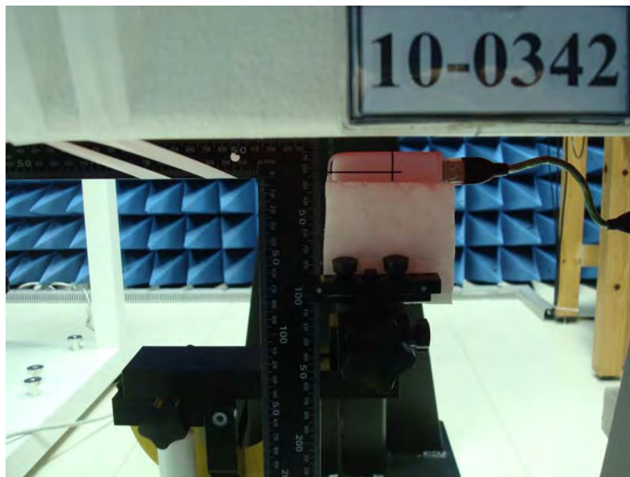
Figure 7. Vertical Back, EUT to Phantom 10mm space with USB Cable _ LCD Open90 degree
