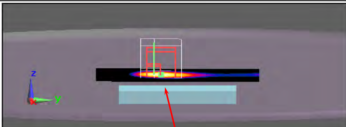
Figure 2. Horizontal Down, EUT to Phantom 5mm space with USB Cable _ LCD Open90 degree
