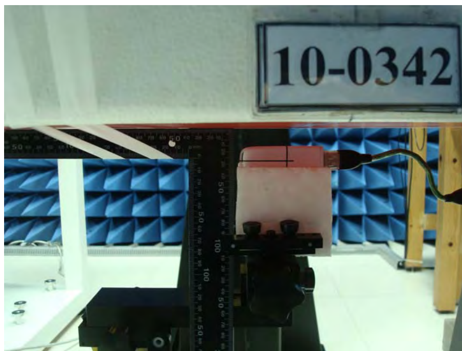
Figure 8. Vertical Back, EUT to Phantom 15mm space with USB Cable _ LCD Open90 degree
