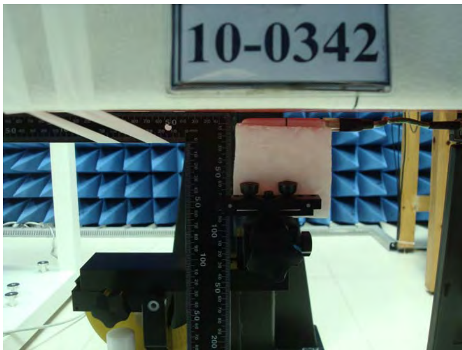
Figure 2. Horizontal Down, EUT to Phantom 5mm space with USB Cable _ LCD Open90 degree
