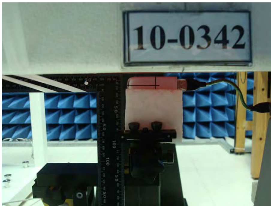
Figure 6. Vertical Back, EUT to Phantom 5mm space with USB Cable _ LCD Open 90 degree
