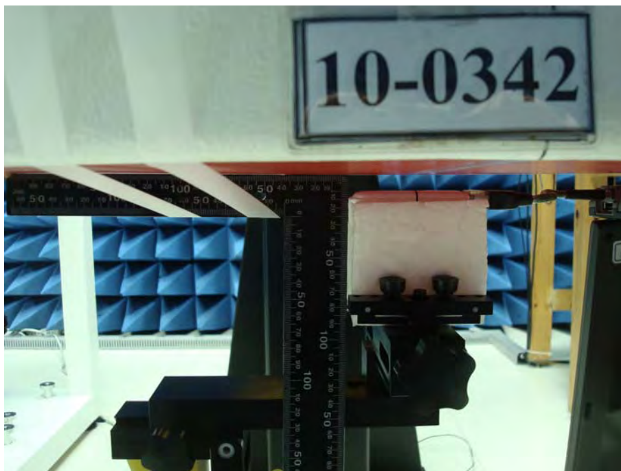
Figure 3. Horizontal Down, EUT to Phantom 10mm space with USB Cable _ LCD Open 90 degree
