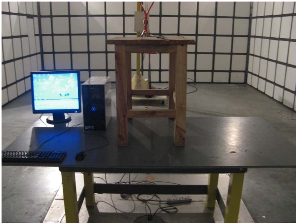
EIRP TEST SETUP BELOW 1GHZ
