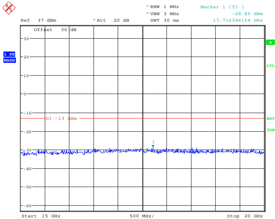
(Plot 4.7.2 A5: Channel 9400: 1880.0MHz @ Traffic WCDMA Band II)
