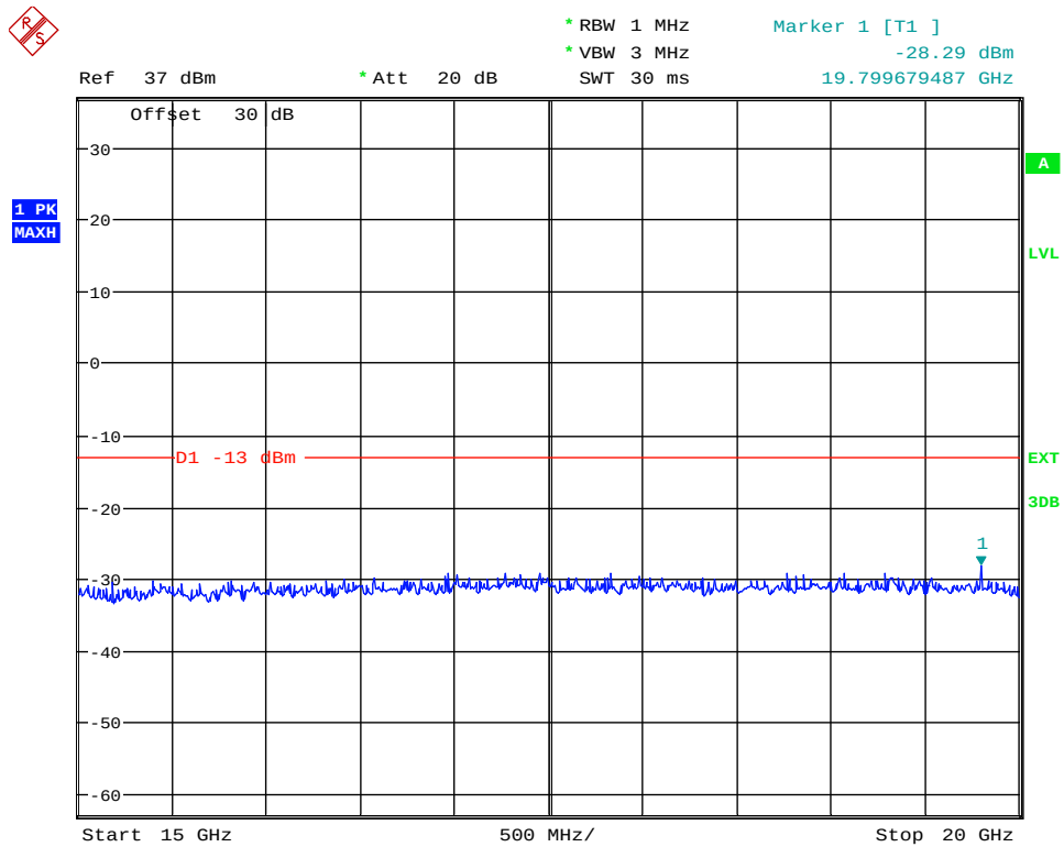
(Plot 4.7.12 A5: Idle @ GPRS1900)
