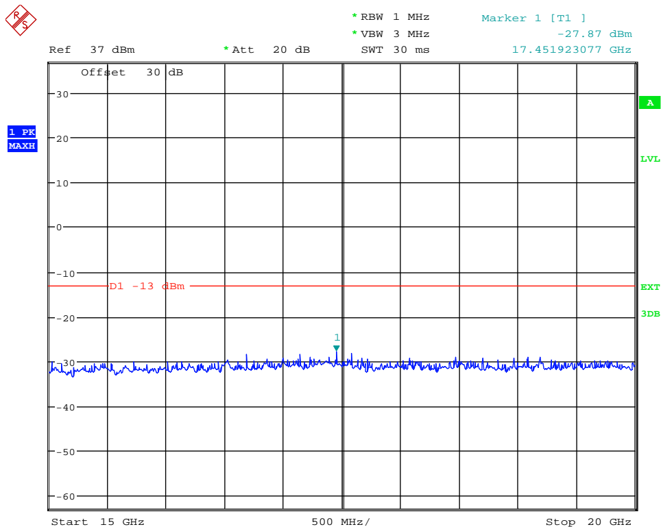
(Plot 4.7.3 A5: Channel 9538: 1907.6MHz @ Traffic WCDMA Band II)
