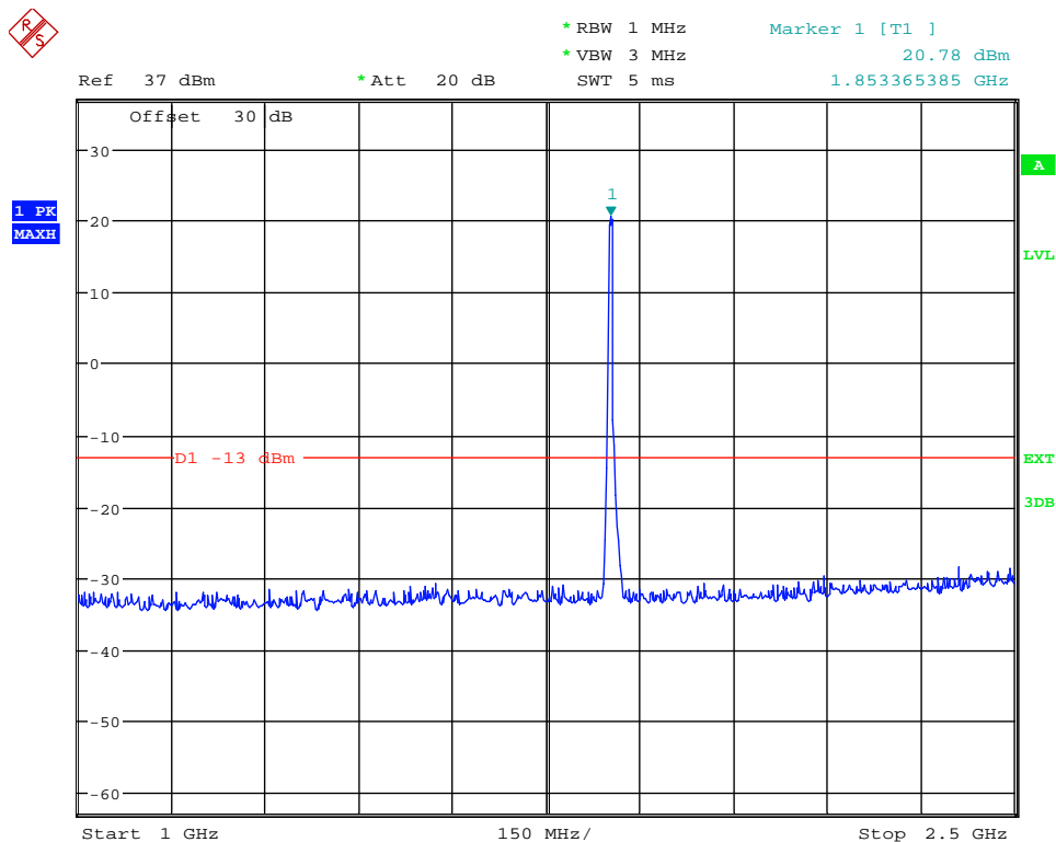
(Plot 4.7.1 A1: Channel 9262: 1852.4MHz @ Traffic WCDMA Band II)
