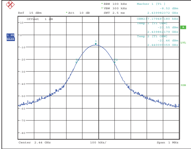
CH19 (99% bandwidth)
