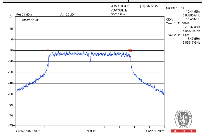
Data Rate 6Mbps
