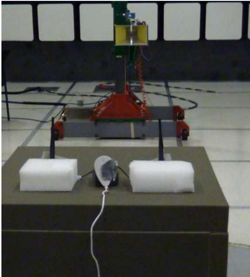
Test Setup – Radiated Emissions
