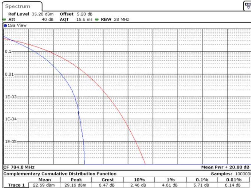
Band12-10MHz-QPSK-23060-50RB#0
