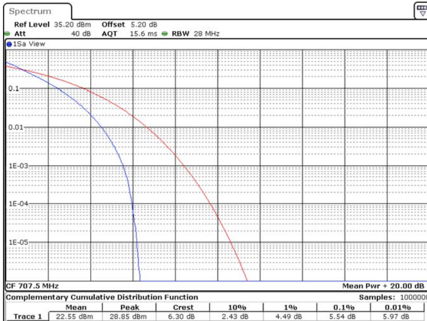
Band12-10MHz-QPSK-23095-50RB#0
