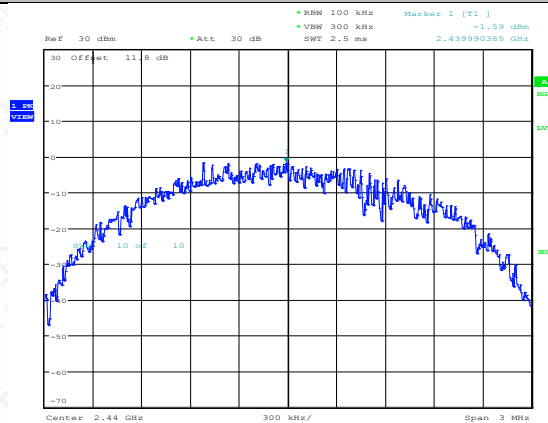
BLE_2M-Ant1-2440-0~Reference-PASS
