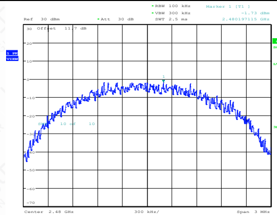
BLE_2M-Ant1-2480-0~Reference-PASS
