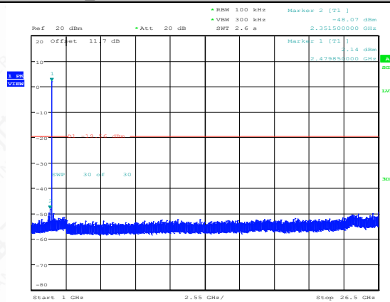
BLE_1M-Ant1-2480-1000~26500-PASS
