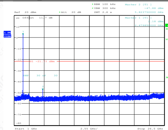
BLE_2M-Ant1-2480-1000~26500-PASS
