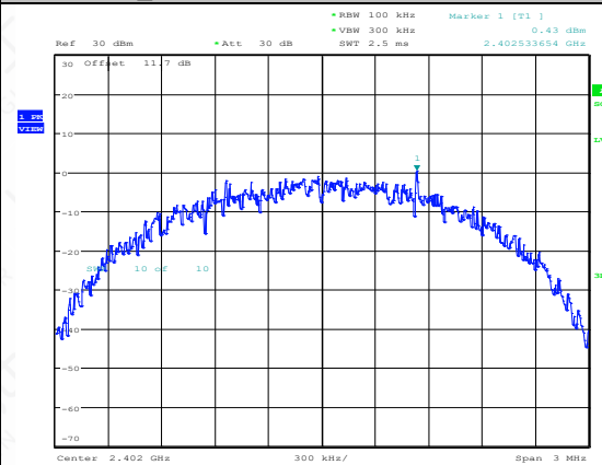
BLE_2M-Ant1-2402-0~Reference-PASS
