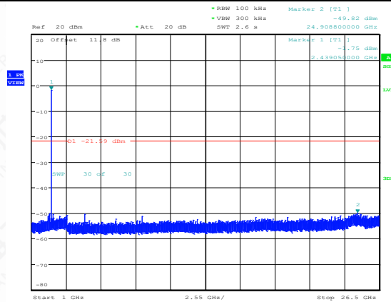
BLE_2M-Ant1-2440-1000~26500-PASS
