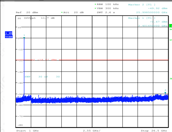
BLE_2M-Ant1-2402-1000~26500-PASS
