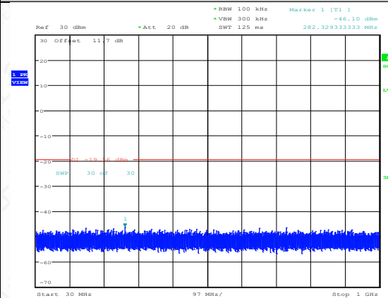
BLE_1M-Ant1-2480-30~1000-PASS
