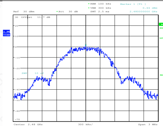
BLE_1M-Ant1-2480-0~Reference-PASS
