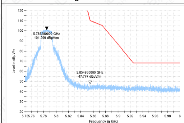
Bandedge-11AC-CH157-PK
