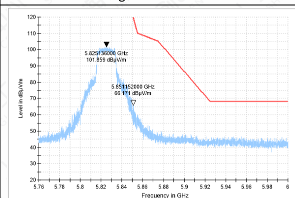
Bandedge-11AC-CH165-PK
