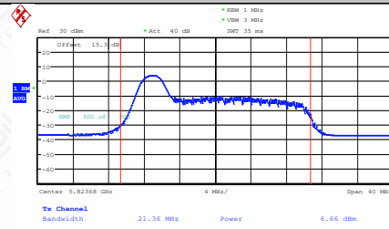
11AX20MIMO-Ant1-5825-26Tone-RU0-PASS
