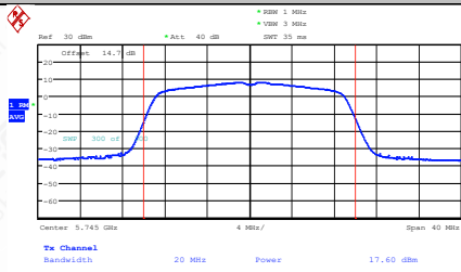
11AC20MIMO-Ant1-5745-PASS
