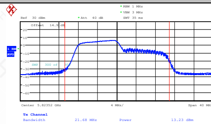
11AX20MIMO-Ant1-5825-106Tone-RU53-PASS
