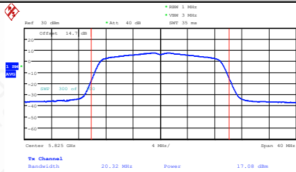
11AC20MIMO-Ant1-5825-PASS
