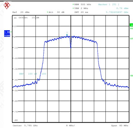
11AC40MIMO-Ant2-5795-PASS
