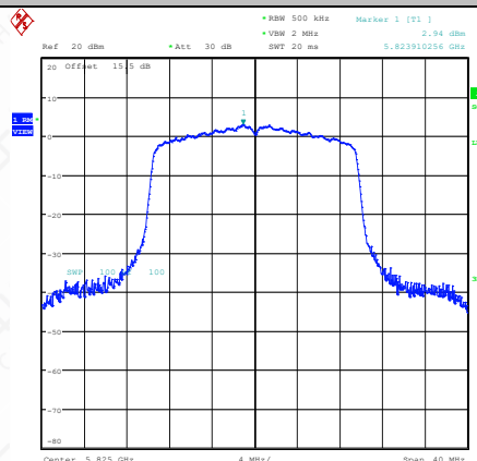
11AX20MIMO-Ant2-5825-PASS
