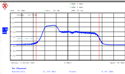
11AX20MIMO-Ant2-5825-52Tone-RU37-PASS
