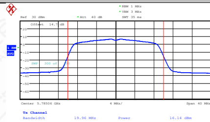
11AC20MIMO-Ant2-5785-PASS
