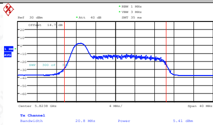
11AX20MIMO-Ant2-5825-26Tone-RU0-PASS
