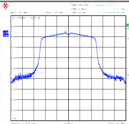
11AX20MIMO-Ant1-5825-PASS
