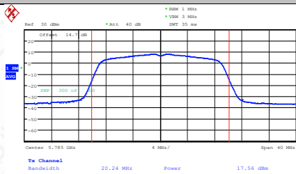
11AC20MIMO-Ant1-5785-PASS
