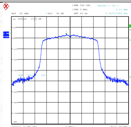
11AX20MIMO-Ant2-5785-PASS
