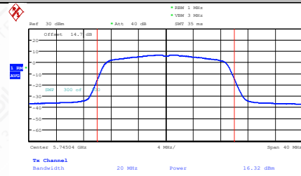
11AC20MIMO-Ant2-5745-PASS
