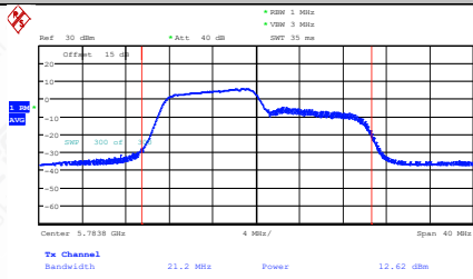
11AX20MIMO-Ant2-5785-106Tone-RU53-PASS
