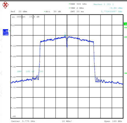
11AC80MIMO-Ant1-5775-PASS
