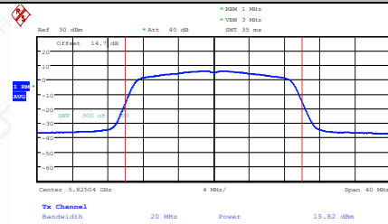
11AC20MIMO-Ant2-5825-PASS
