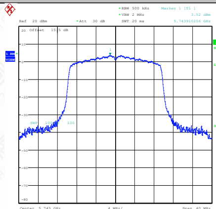
11AX20MIMO-Ant2-5745-PASS
