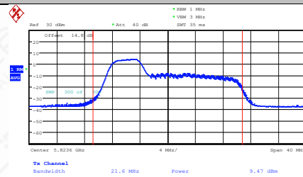
11AX20MIMO-Ant1-5825-52Tone-RU37-PASS
