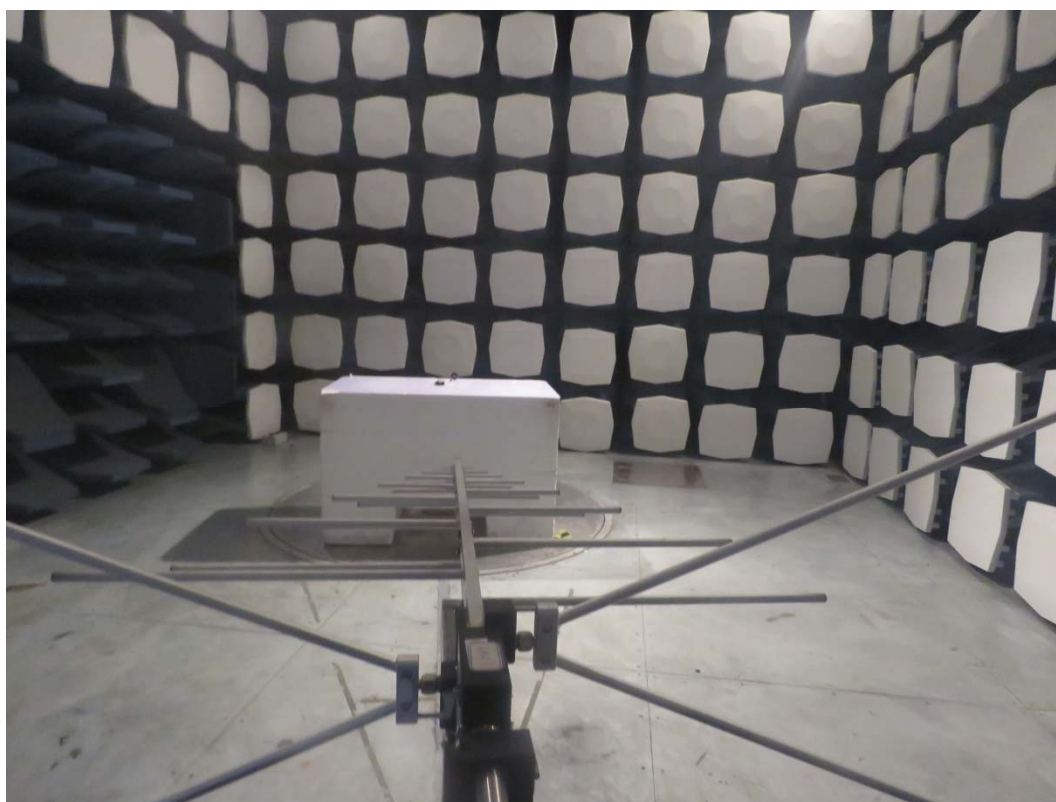
30MHz-1GHz
