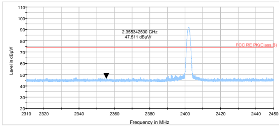
BLE Channel 0 Peak
