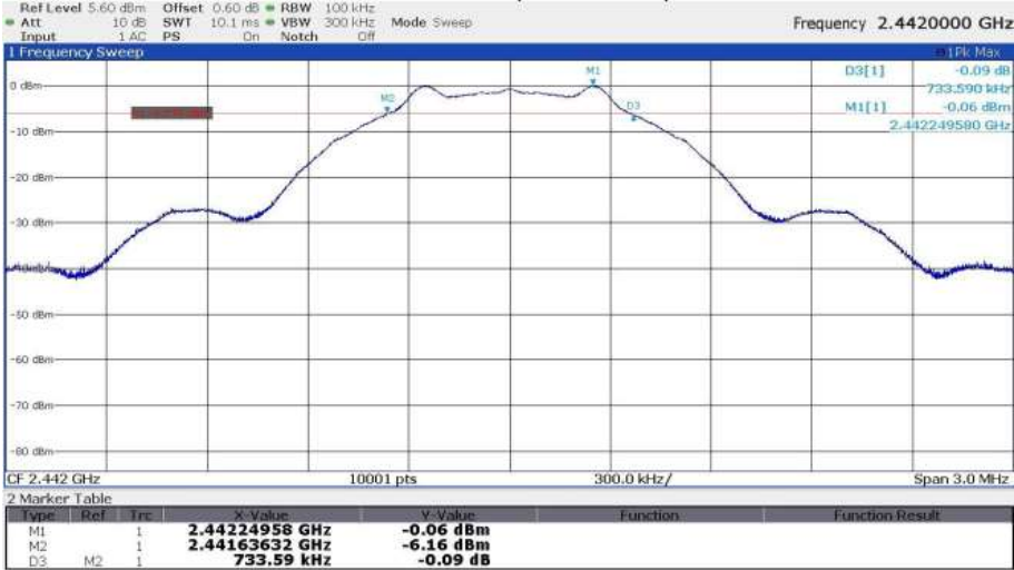
Channel 18 (2442 MHz)
