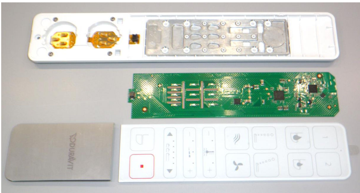
fig. 5 – all parts front side
