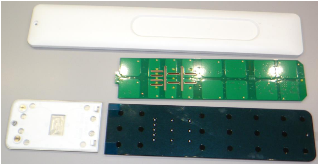
fig. 4 – all parts back side
