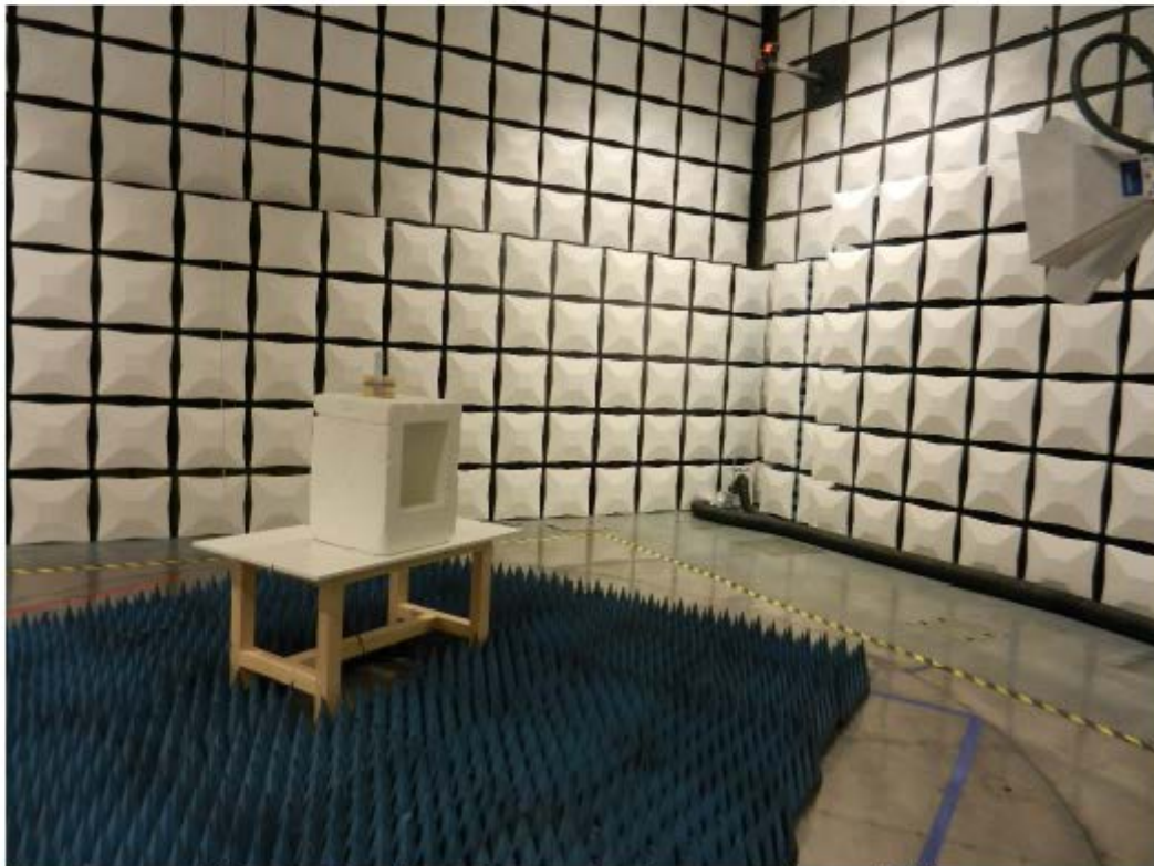
Figure 83 – Test Setup for frequencies >1 GHz
