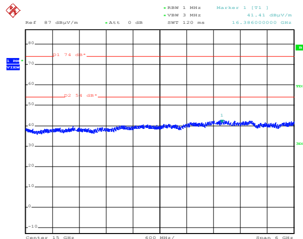
Spurious emissions from 12 to 18 GHz, RMS
