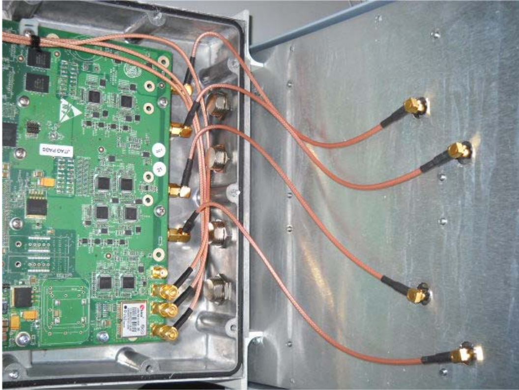
Photograph No.2 Pico base station with internal antennas internal view
