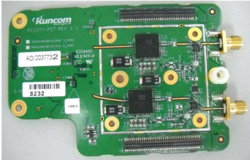
Photograph No.14 RF module top view
