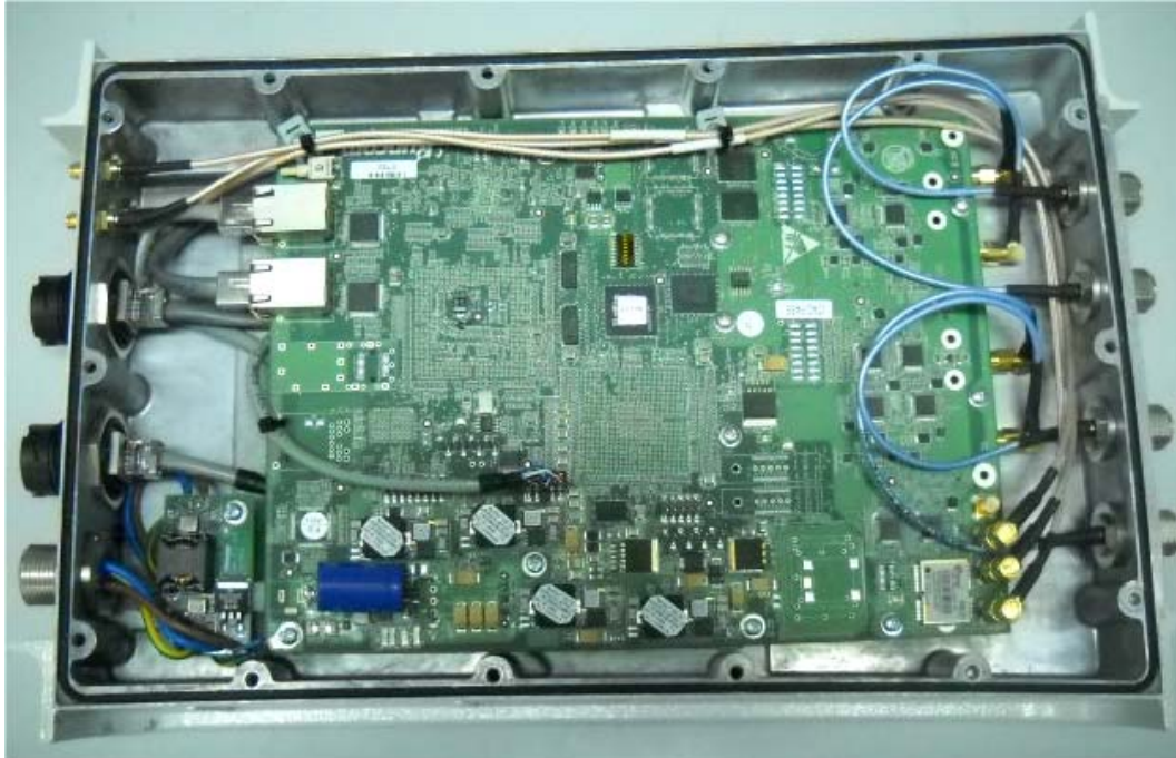
Photograph No.6 Pico base station with external antennas view
