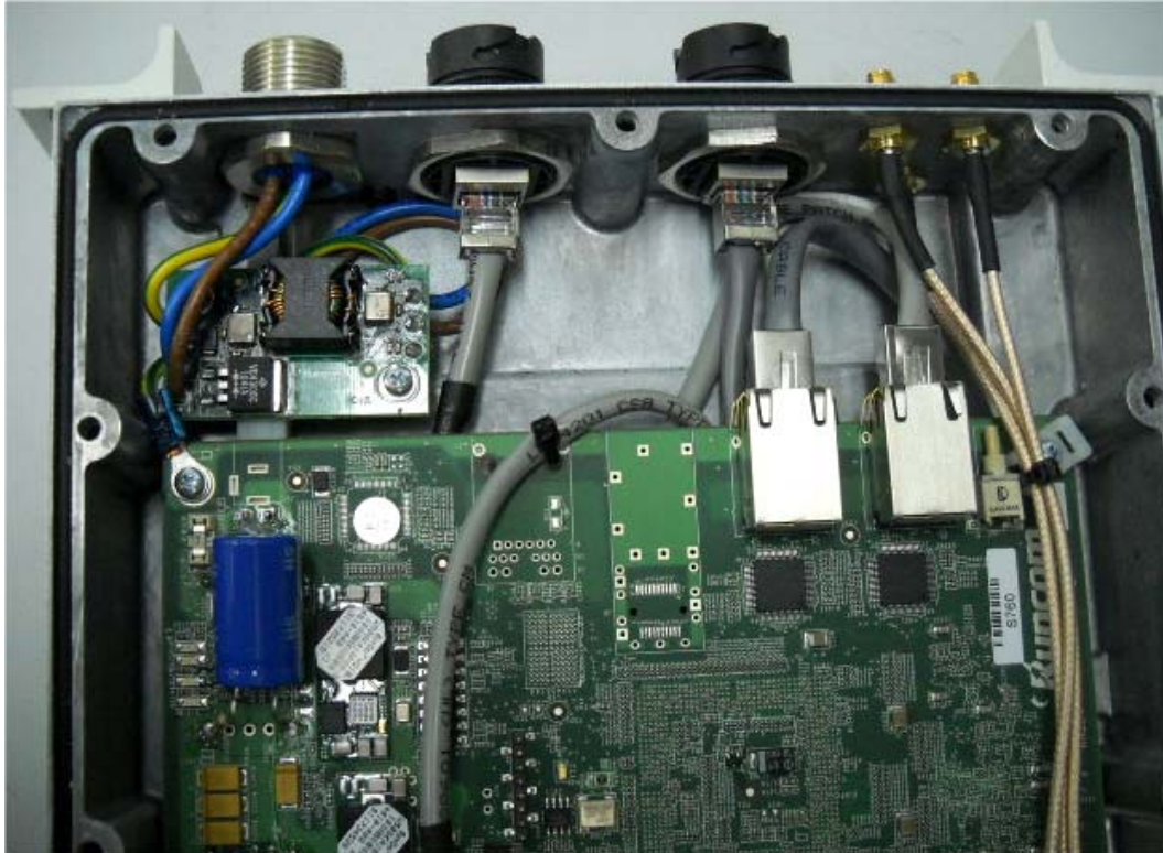
Photograph No.8 Pico base station internal close view
