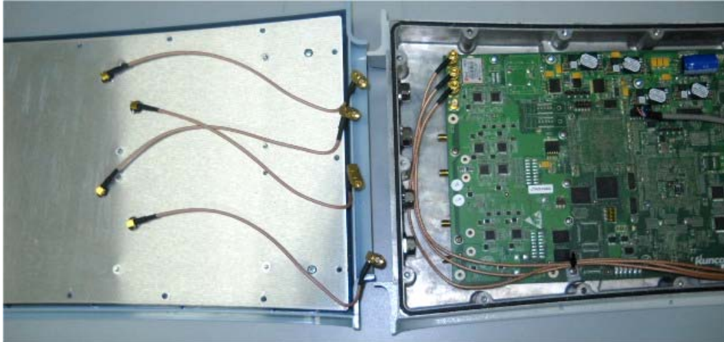
Photograph No.3 Pico base station with internal antennas internal view
