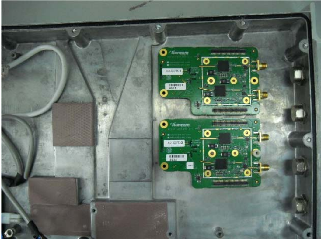
Photograph No.13 RF modules
