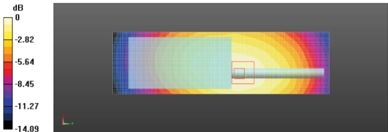
Figure 1: Face held for 4FSK Modulation at 12.5 KHz Channel Separation Front towards Phantom 162.10 MHz
