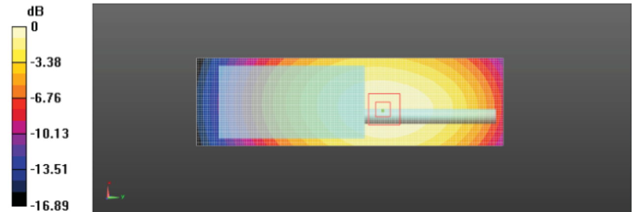
Figure 3: Face held for FM Modulation at 12.5 KHz Channel Separation Front towards Phantom 162.10 MHz
