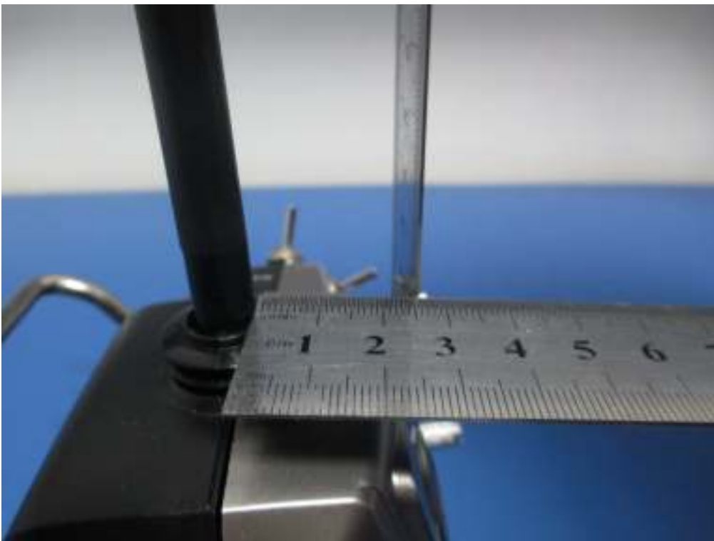
Antenna distance from front control surface about 25mm
