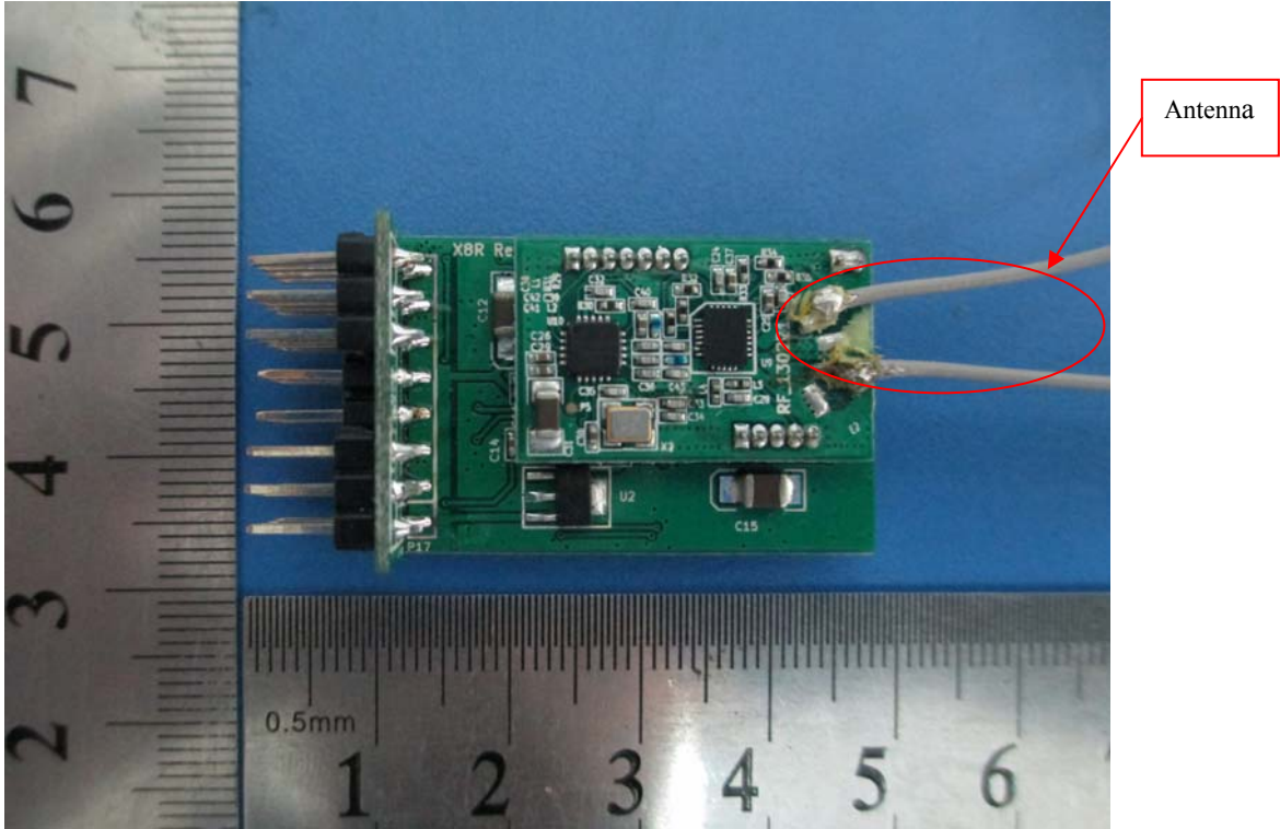
EUT Main PCB Board – Front View
