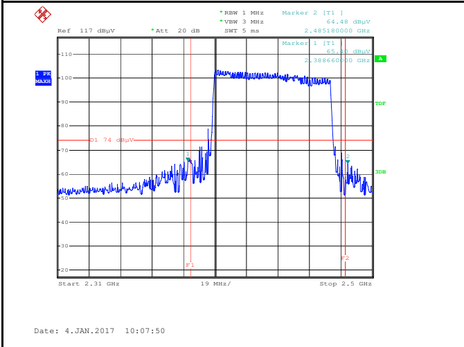
2-FSK -Hopping-PK-V
