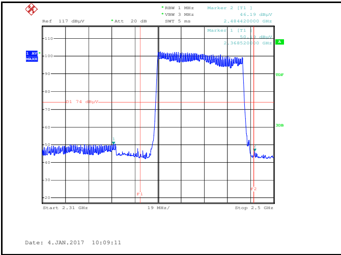
2-FSK -Hopping-Ave-V
