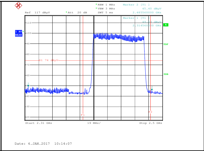
2-FSK -Hopping-Ave-H
