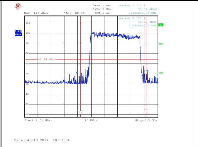
2-FSK -Hopping-PK-H
