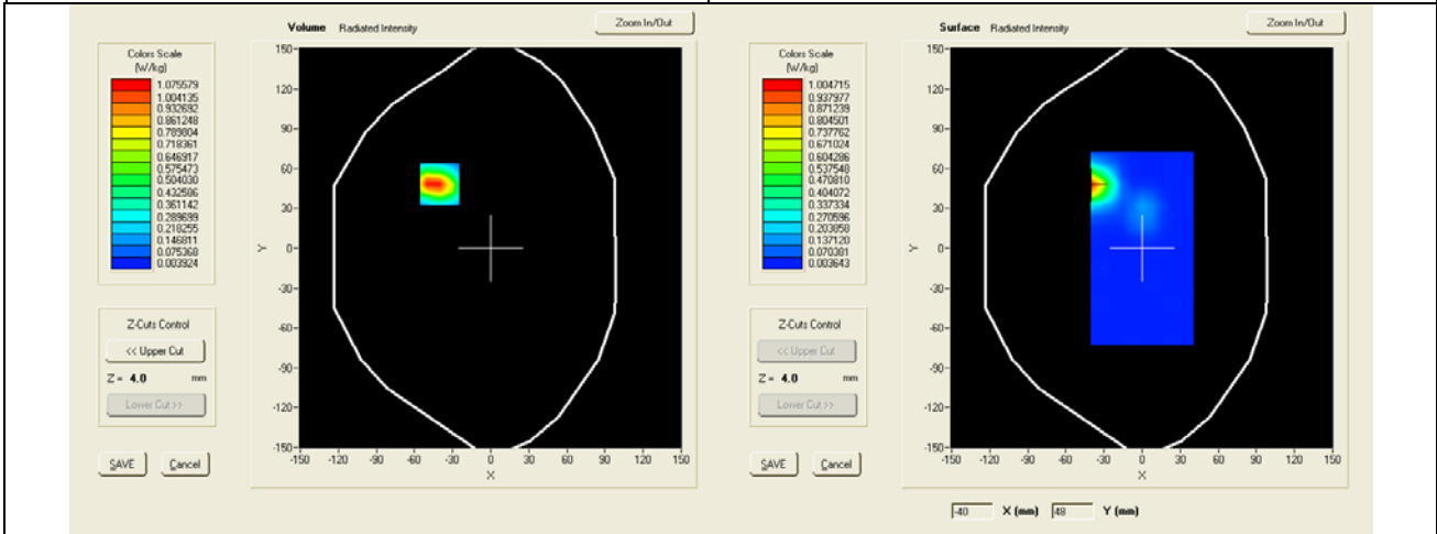
SAR, Z Axis Scan (X = -40, Y = 48)
