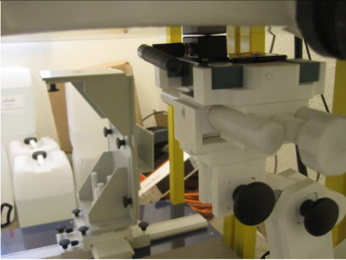
SAR Test setup - 3
