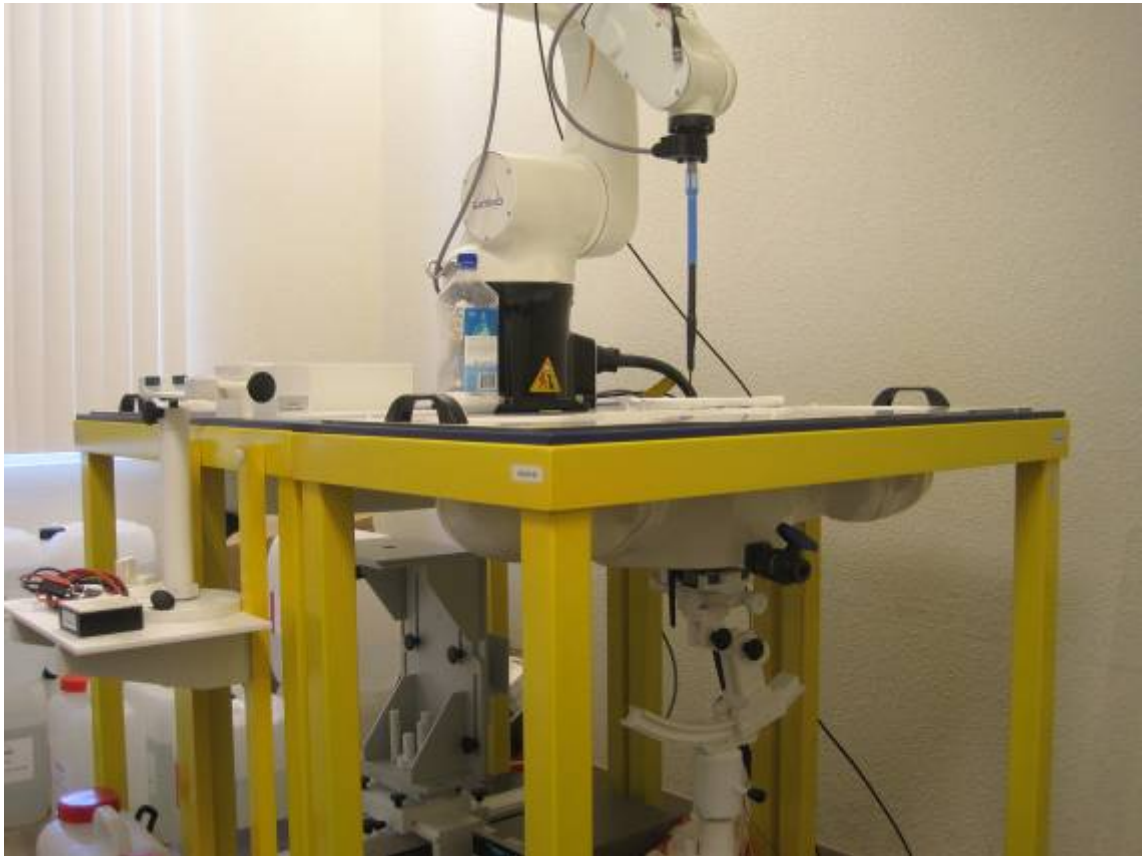
SAR Test setup - 5
