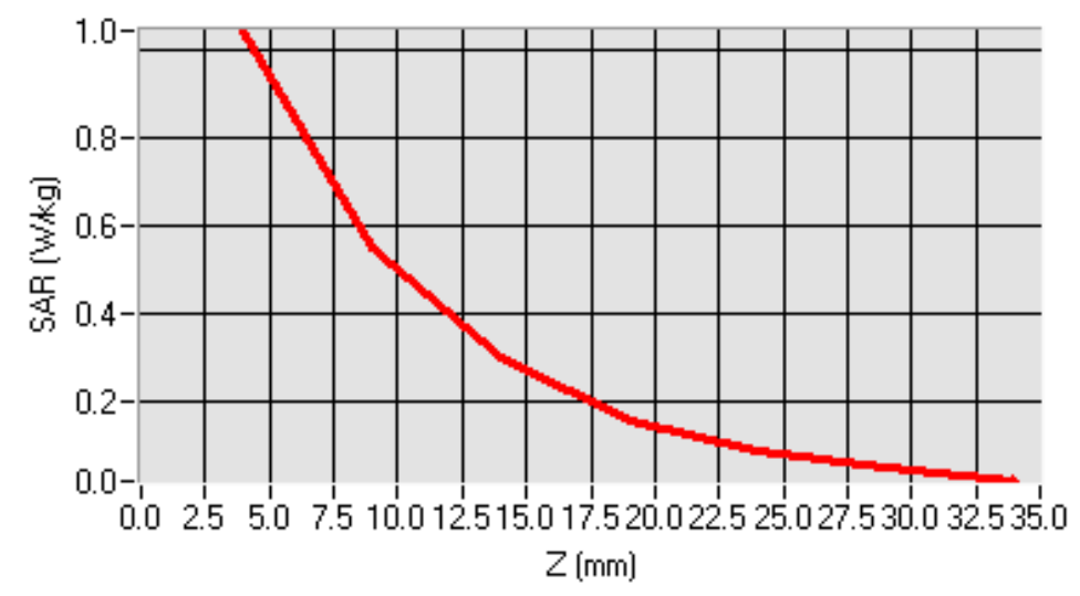
SAR, Z Axis Scan (X = -40, Y = 54)
