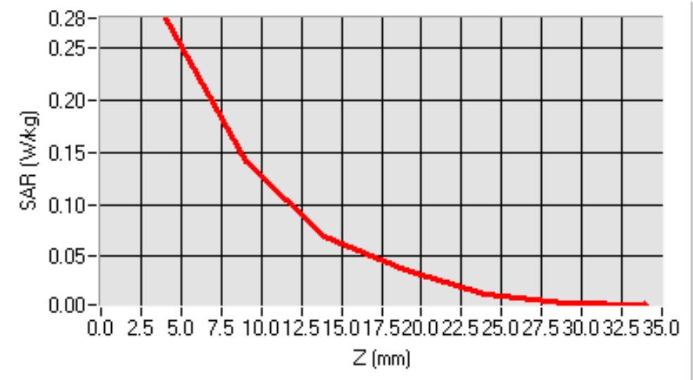
SAR, Z Axis Scan (X = 5, Y = 31)
