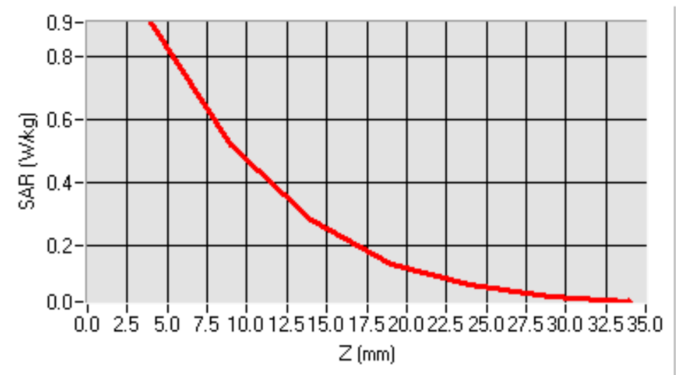
SAR, Z Axis Scan (X = -40, Y = 53)
