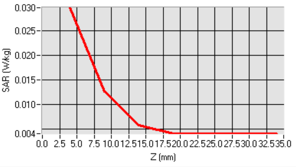
SAR, Z Axis Scan (X = 3, Y = 32)
