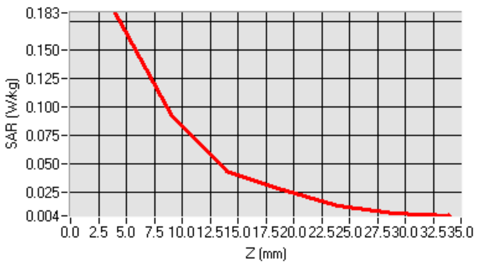
SAR, Z Axis Scan (X = 9, Y = 72)
