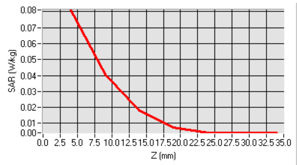
SAR, Z Axis Scan (X = 1, Y = 32)
