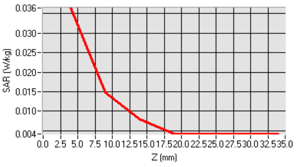
SAR, Z Axis Scan (X = 5, Y = 32)
