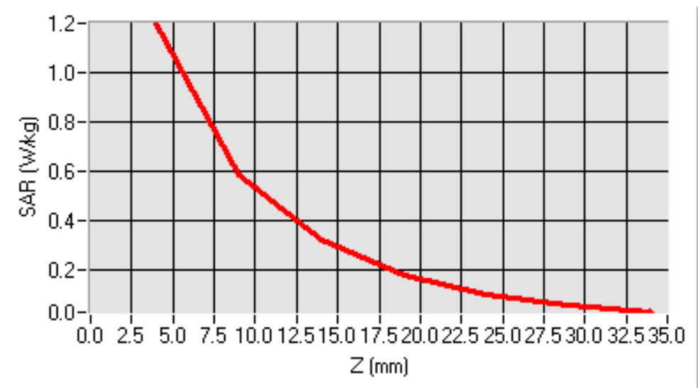
SAR, Z Axis Scan (X = -40, Y = 48)
