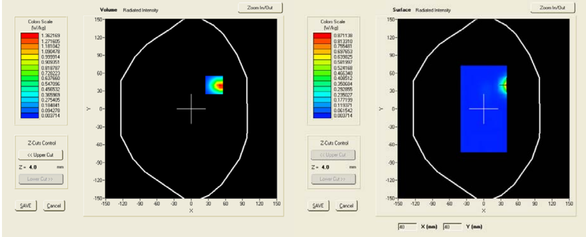
SAR, Z Axis Scan (X = 40, Y = 40)
