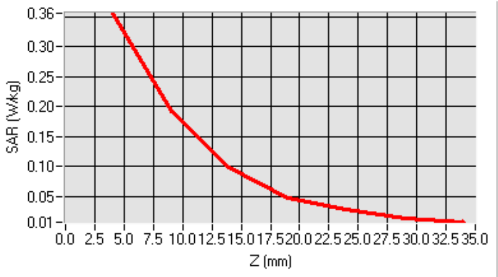
SAR, Z Axis Scan (X = 8, Y = 72)
