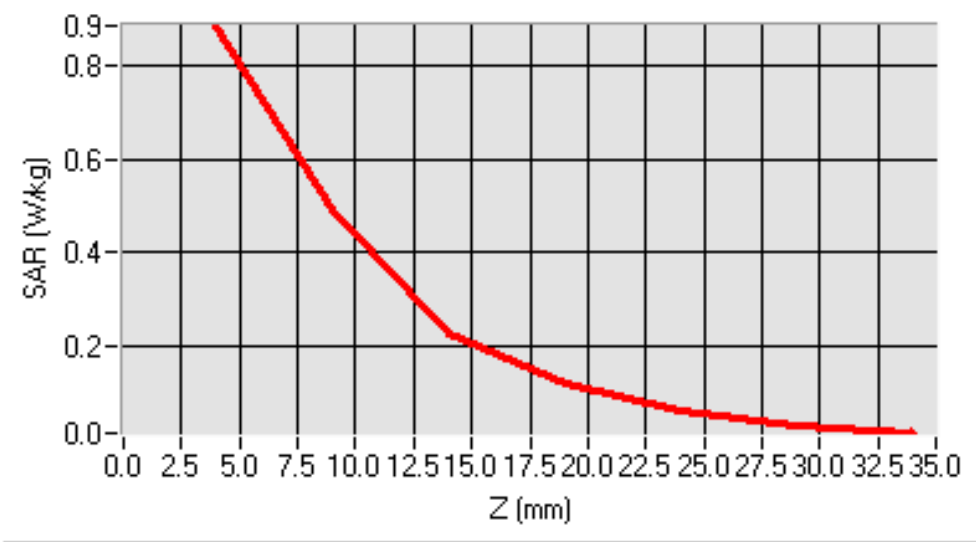
SAR, Z Axis Scan (X = 40, Y = 40)
