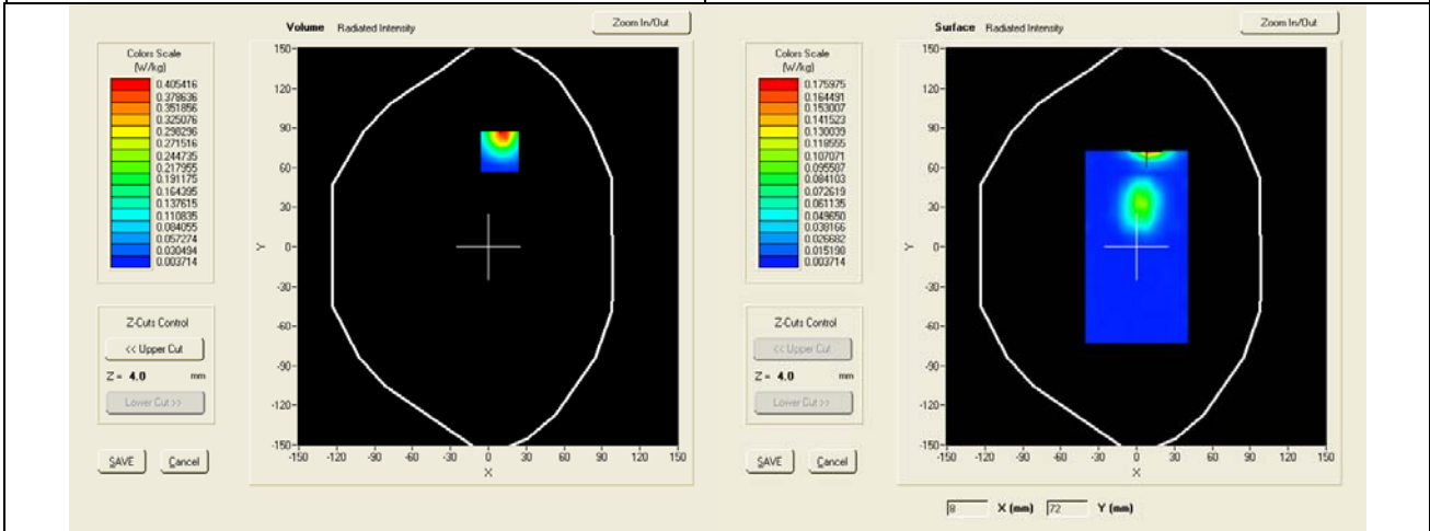
SAR, Z Axis Scan (X = 9, Y = 72)
