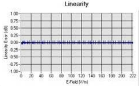
Linearity: \pm 0.92\% ( \pm 0.04\text{dB} )
