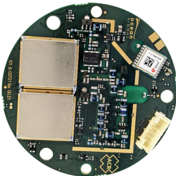
Figure 4: EPIRB3/EPIRB3 Pro PCB – Rear side
