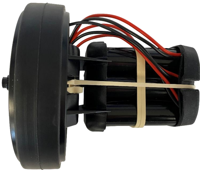
Figure 6: EPIRB3/EPIRB3 Pro – Battery pack in carrier.
