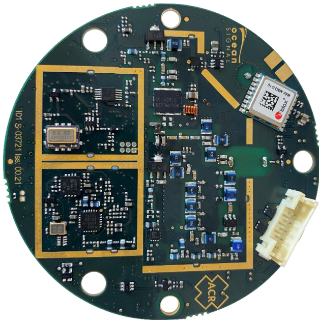
Figure 5: EPIRB3/EPIRB3 Pro PCB – Rear side with screening cans removed.
