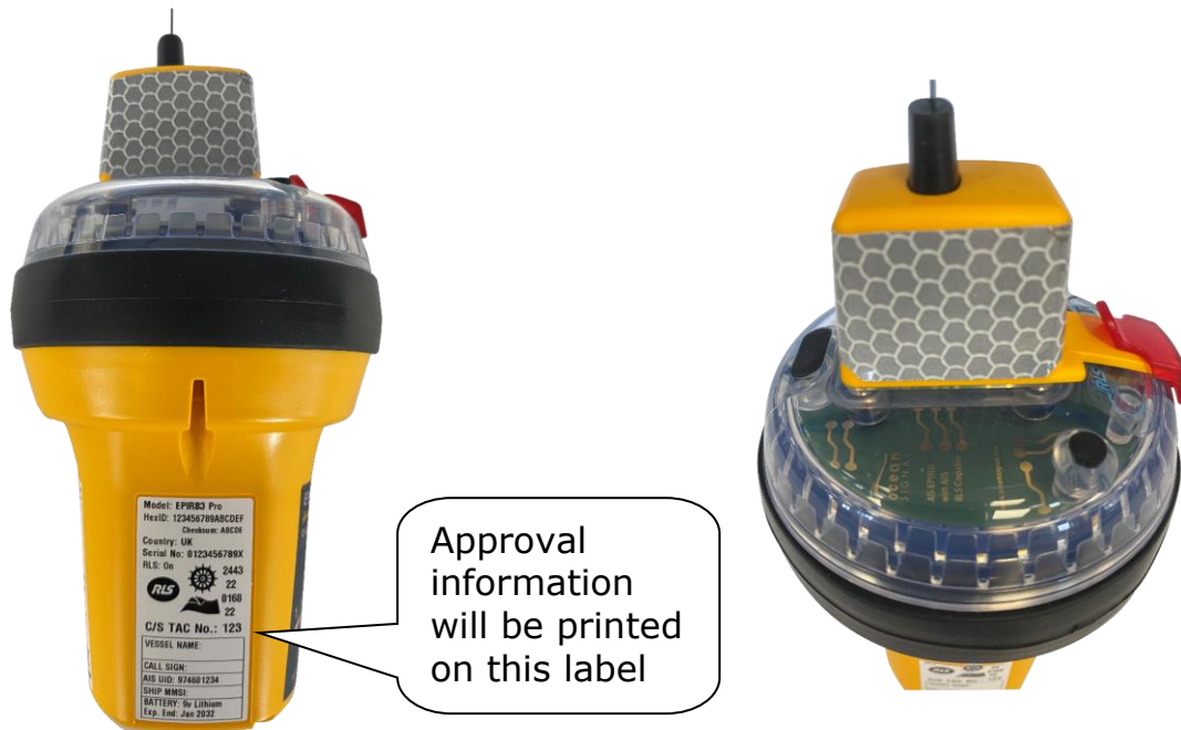
Figure 2: SafeSea EPIRB3 PRO – Right Hand Side View (Antenna Not Shown for Clarity)
