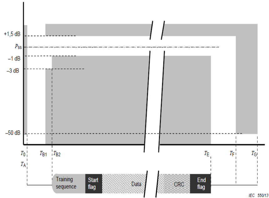
Figure 22 - Power Versus Time Mask
