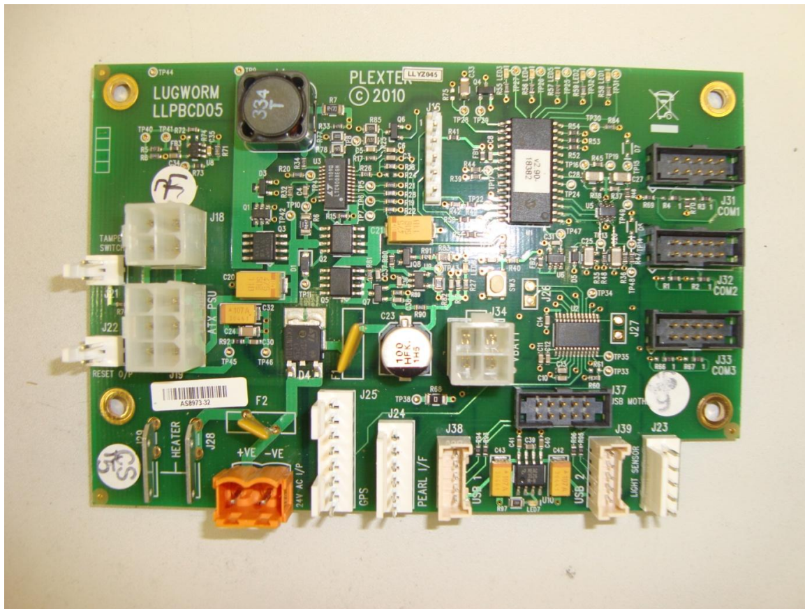
Interface board
