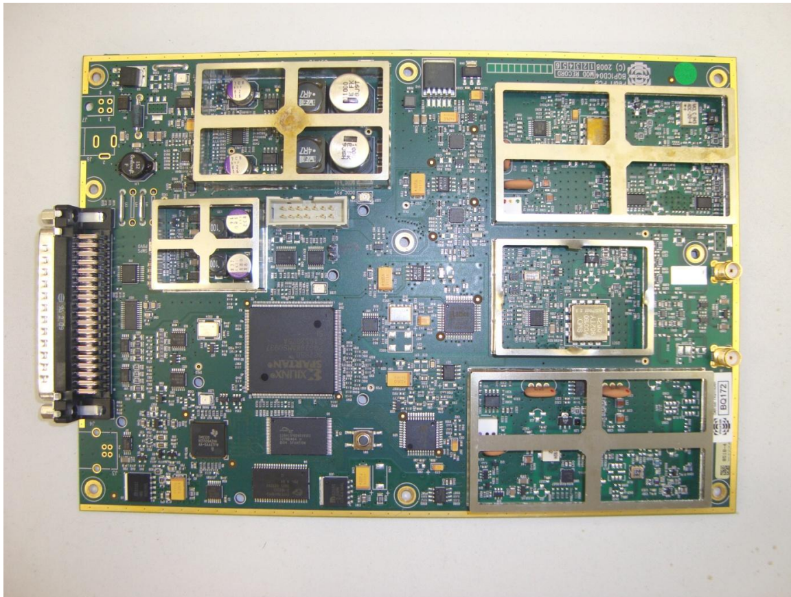
Radio board – shielding removed
