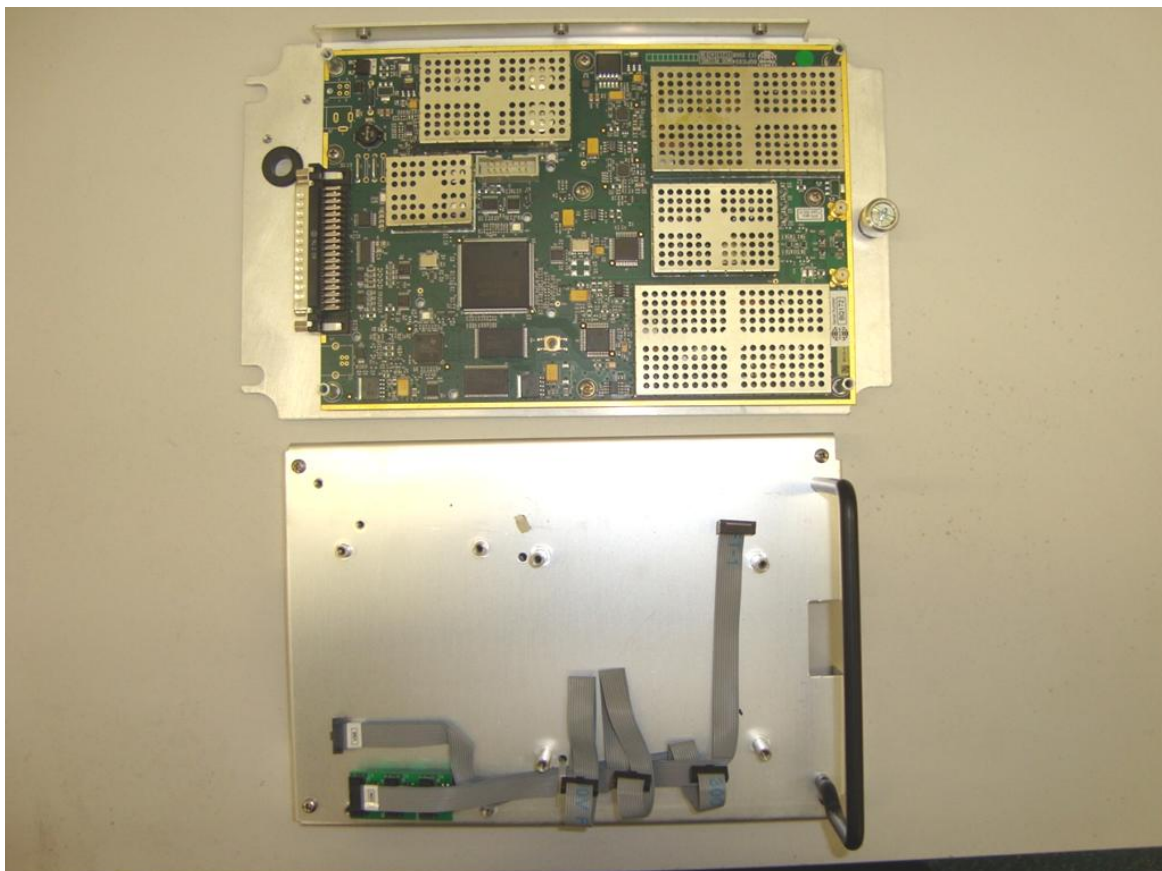
Chassis base with radio board plus cover for radio
