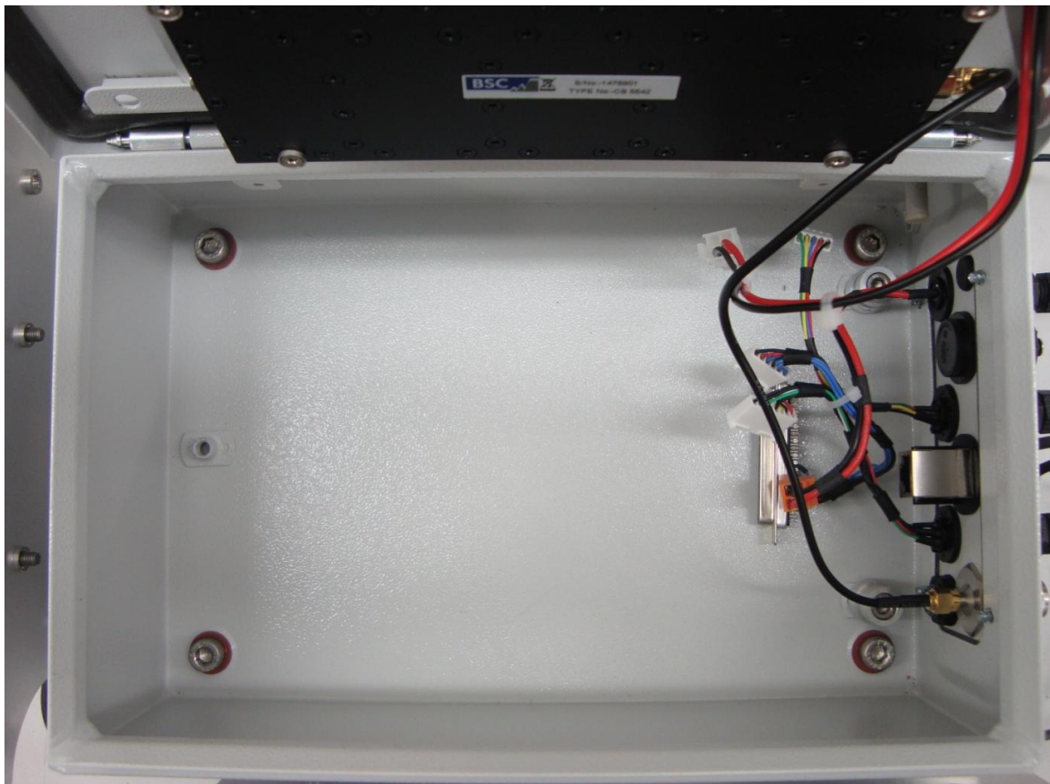
Internal chassis removed from case
