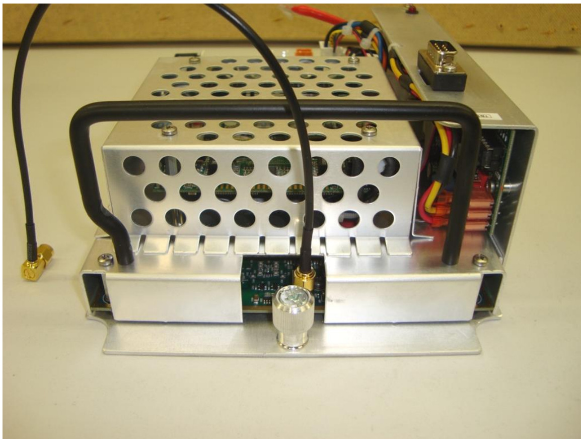
Chassis top – single board computer is under top perforated cover
