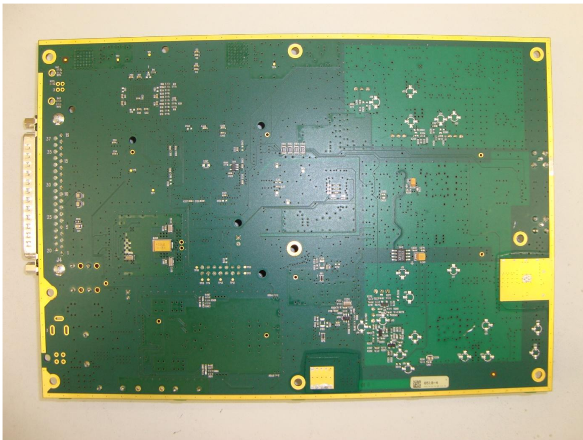
Radio board underside
