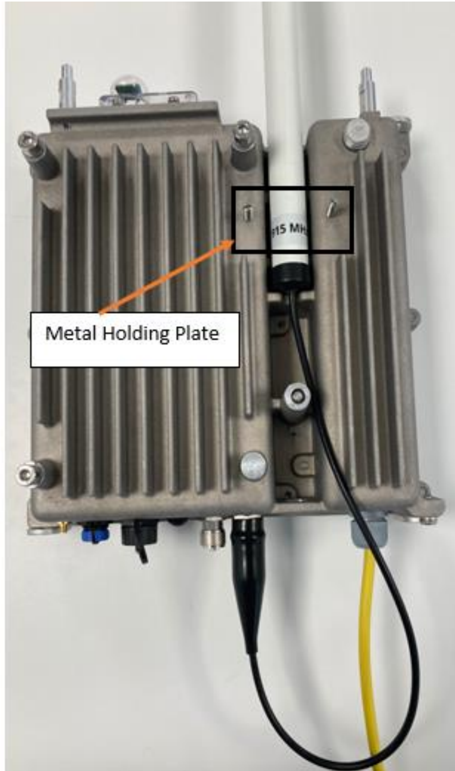
Photo of UNB Antenna fitting – Holding Plate removed.
