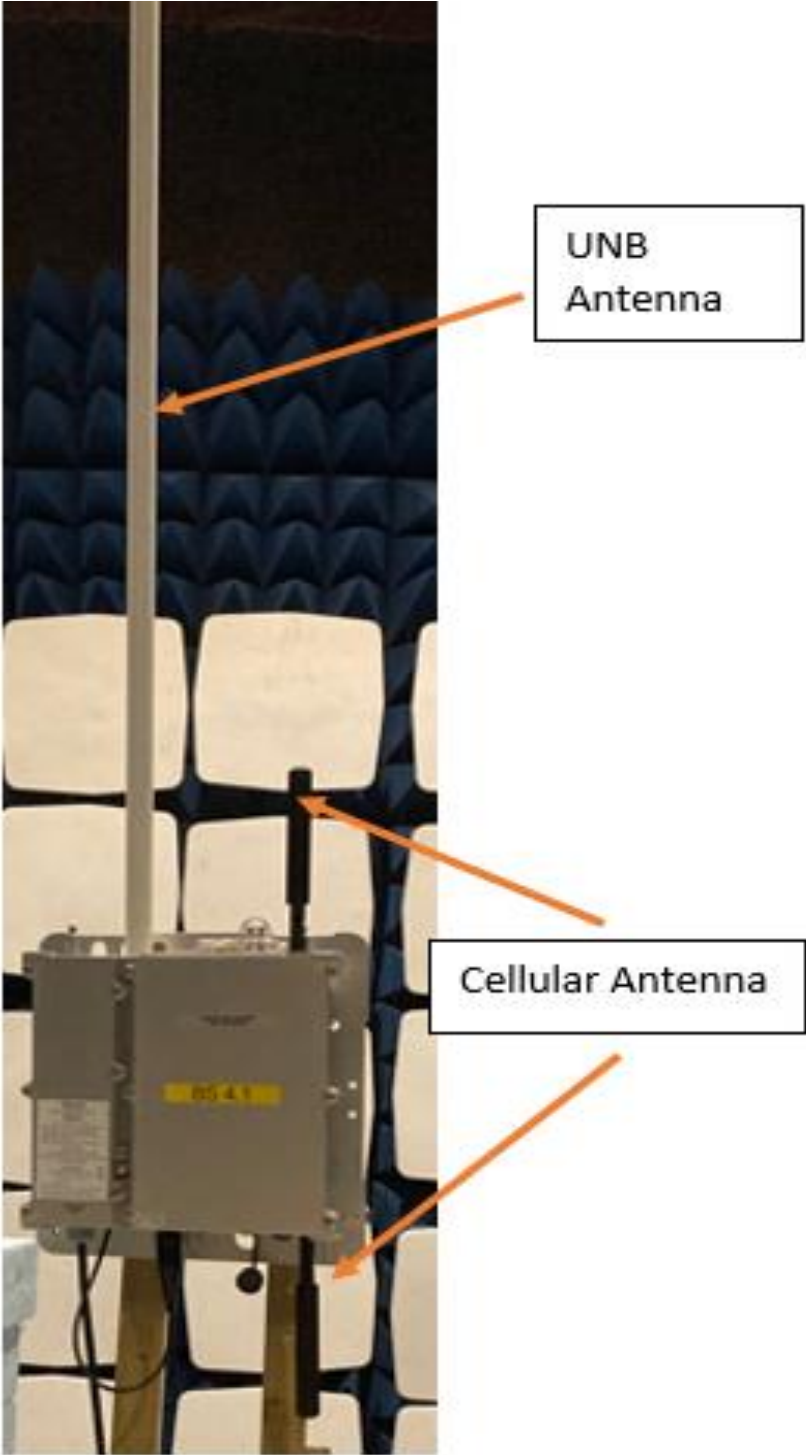
Photo of UNB and Cellular Antenna
