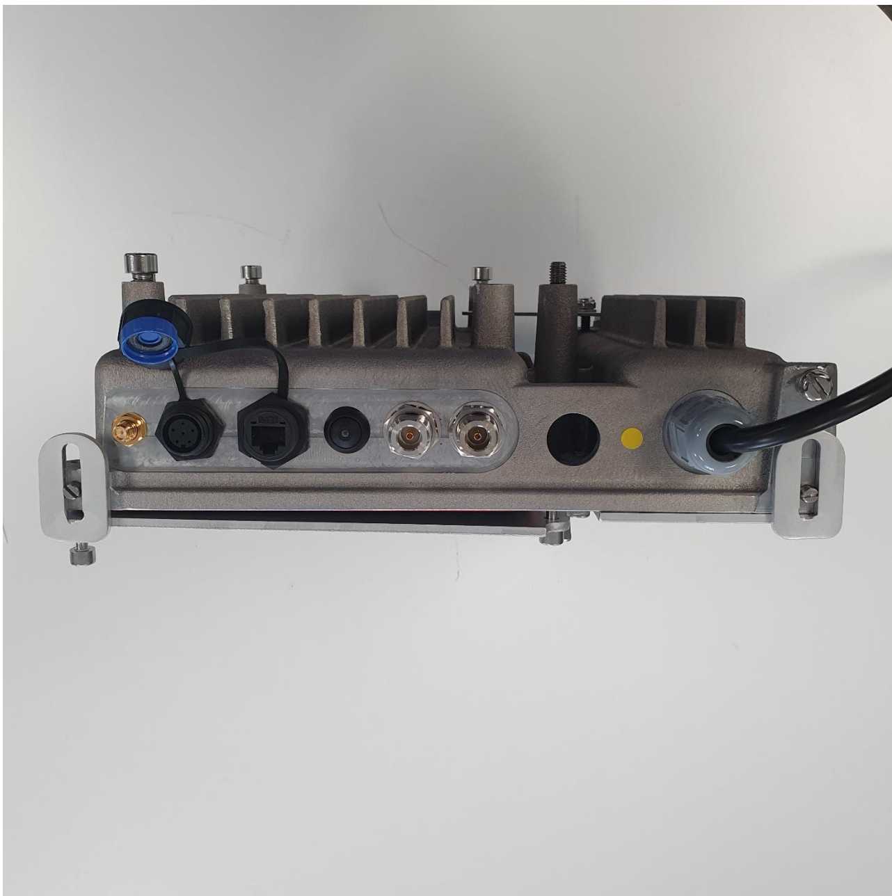
Bottom View (Connector Cover Caps Removed)
