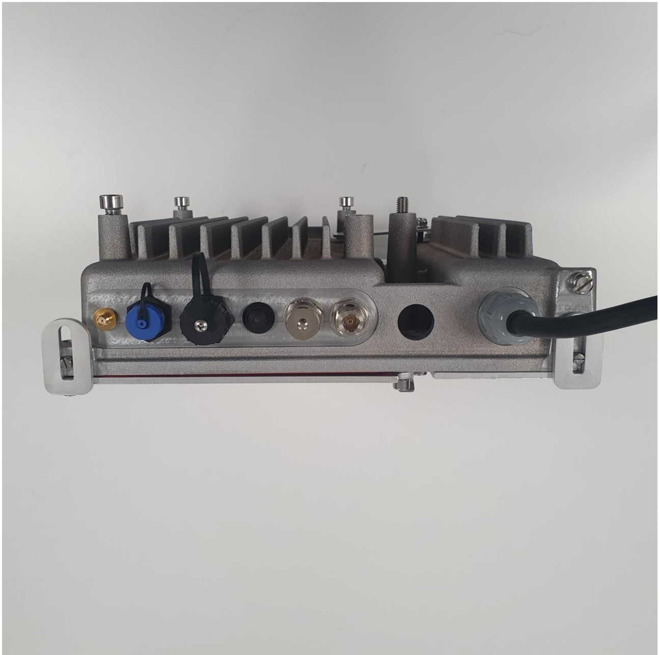
Bottom View (Connector Cover Caps Fitted)
