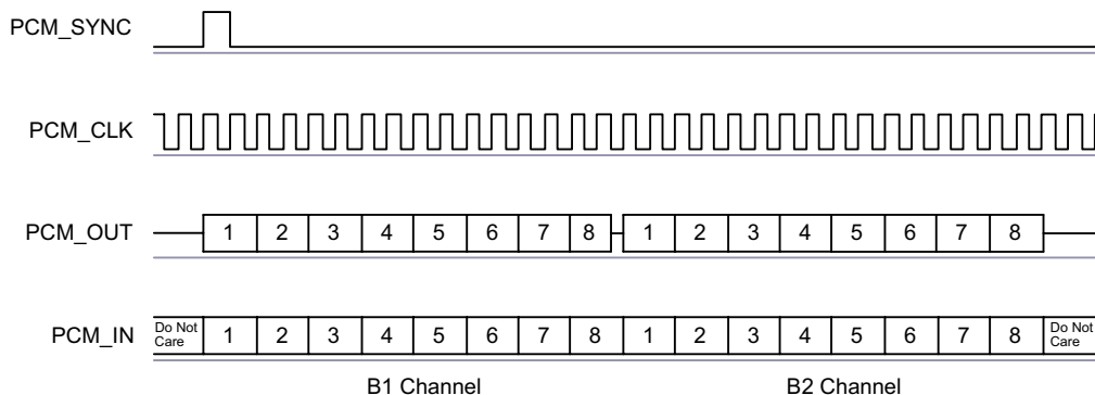
Figure 11.25: GCI Interface
