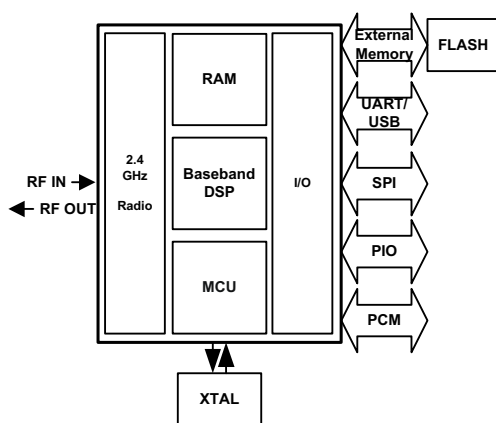
System Architecture
