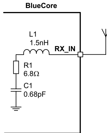
Figure 11.2: Circuit RX_IN
