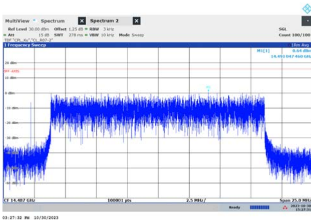
f_{HIGH} (19.8 MHz, 16QAM)
