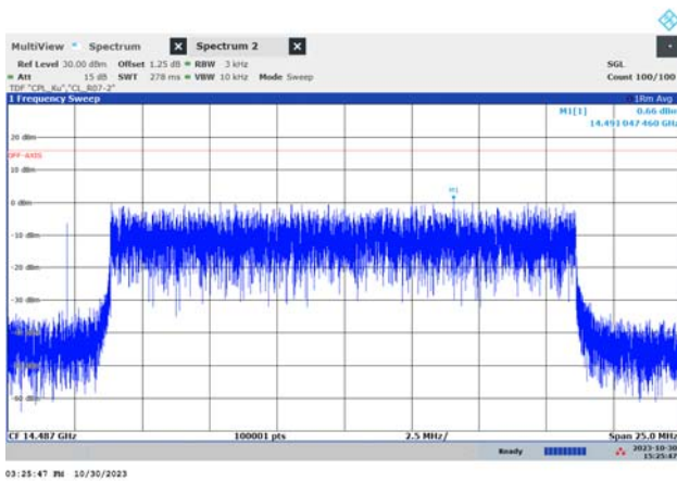
f_{HIGH} (19.8 MHz, 8PSK)
