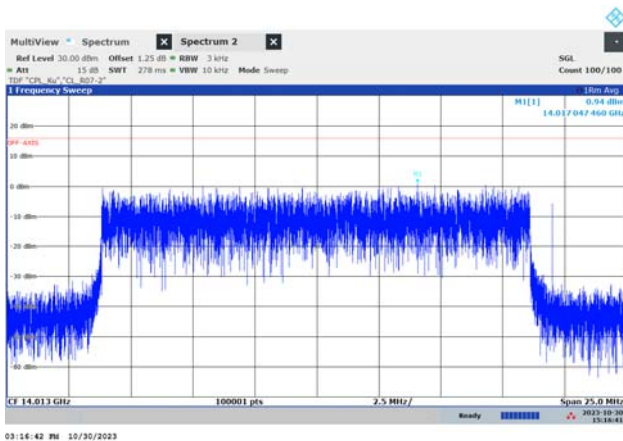
f_{LOW} (19.8 MHz, 16QAM)
