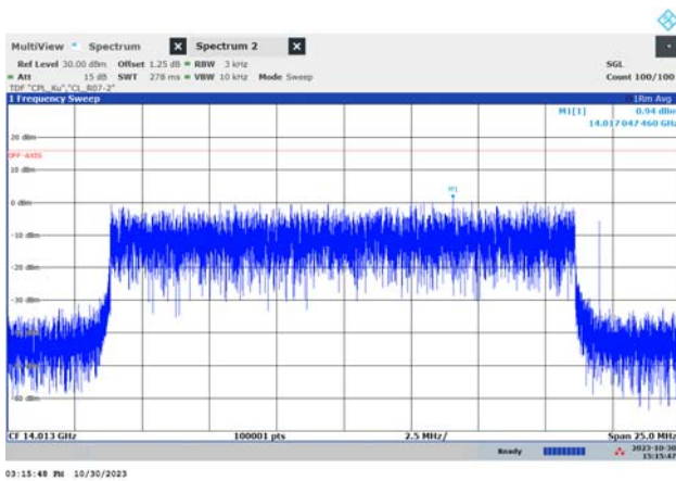
f_{LOW} (19.8 MHz, 8PSK)
