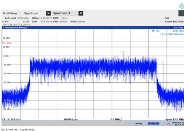
f_{MID} (19.8 MHz, 16QAM)
