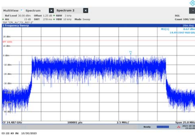
f_{HIGH} (19.8 MHz, QPSK)
