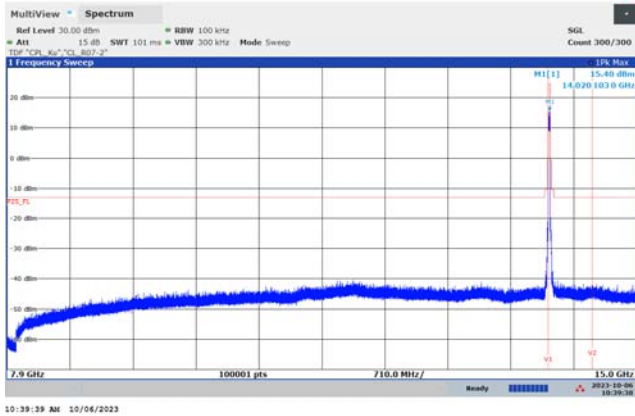
7.9 GHz to 15 GHz
