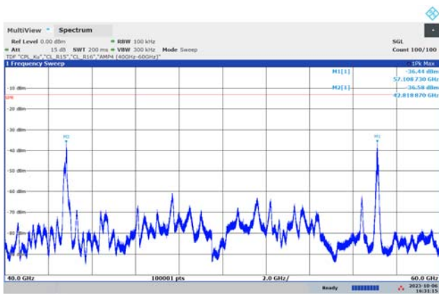
40 GHz to 60 GHz
