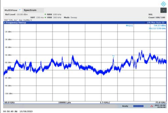
60 GHz to 75 GHz
