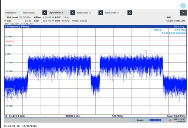
f_{HIGH} (39.6 MHz, 16QAM)
