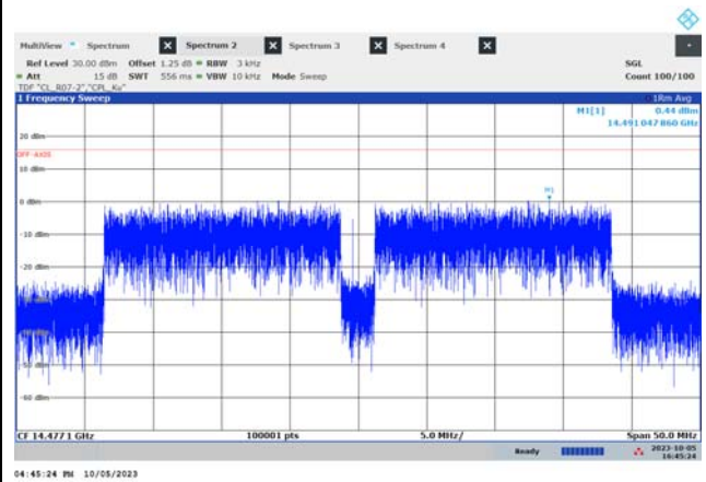
f_{HIGH} (39.6 MHz, 8PSK)
