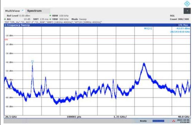
26.5 GHz to 40 GHz
