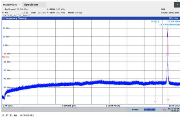
7.9 GHz to 15 GHz
