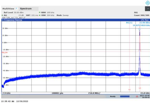
7.9 GHz to 15 GHz
