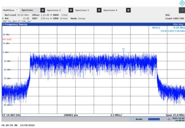
f_{HIGH} (19.8 MHz, QPSK)
