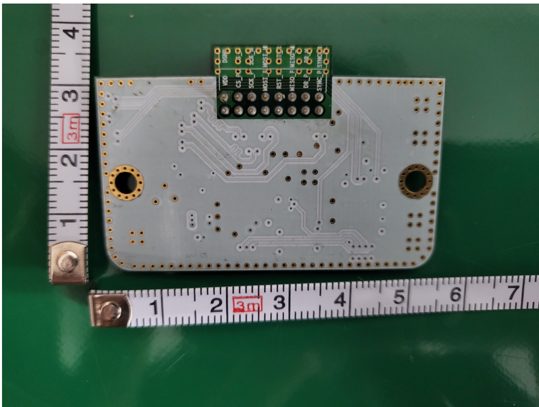
IMU Rear
