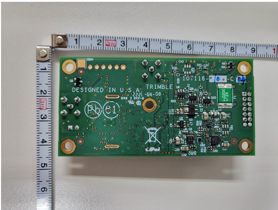
EGR Rear
