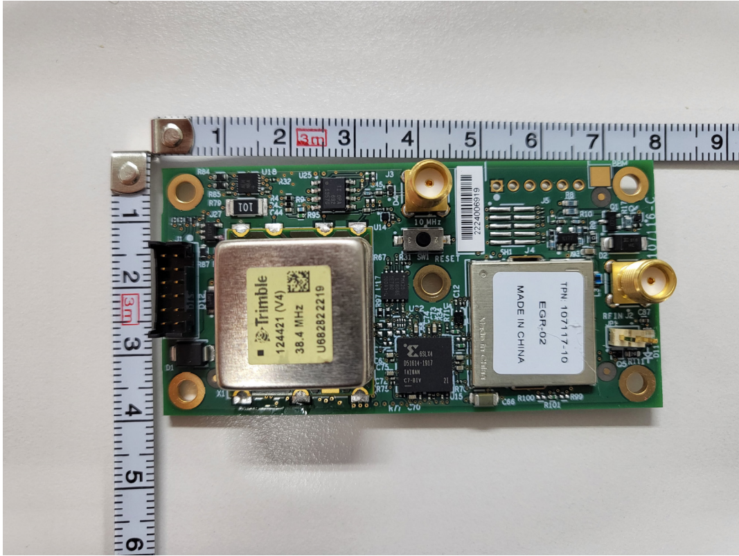
EGR Front
