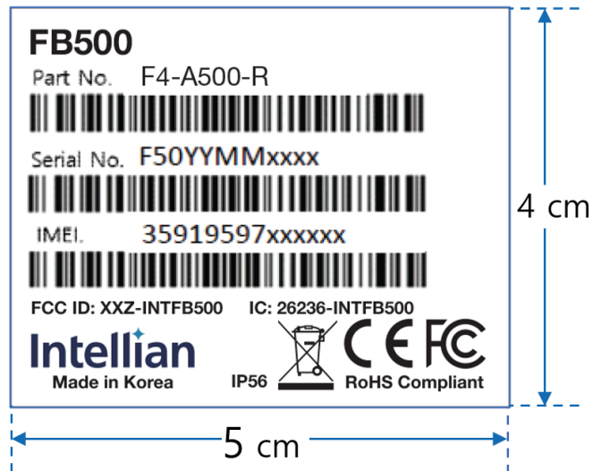
(ADU Rack Type)
