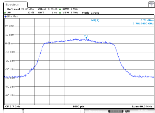
802.11ax20_5700MHz_RU_242/61_Chain 1
