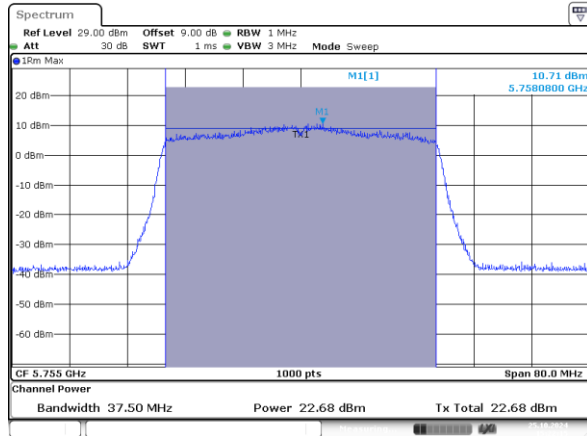
802.11ax40_5755MHz_RU_484/65_Chain 0
