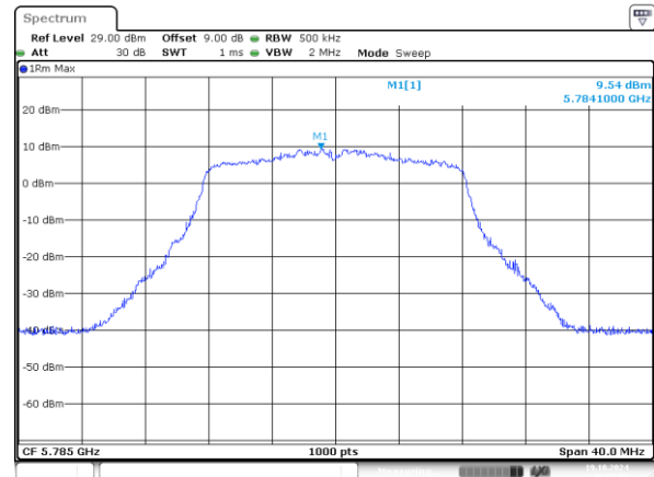
802.11a_5785MHz_Chain 1
