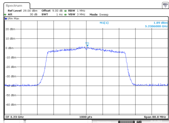
802.11ax40_5230MHz_RU_484/65_Chain 1
