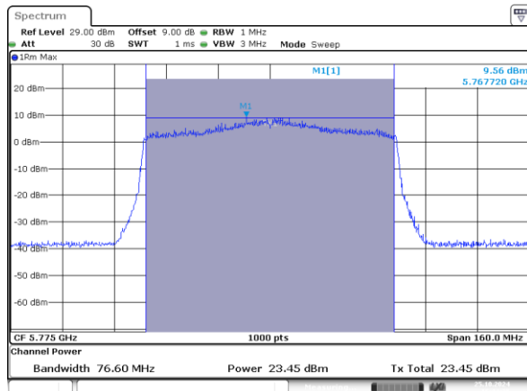
802.11ax80_5775MHz_RU_996/67_Chain 0
