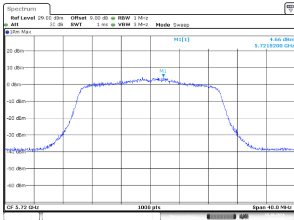
802.11ax20_5720MHz_RU_242/61_Chain 0
