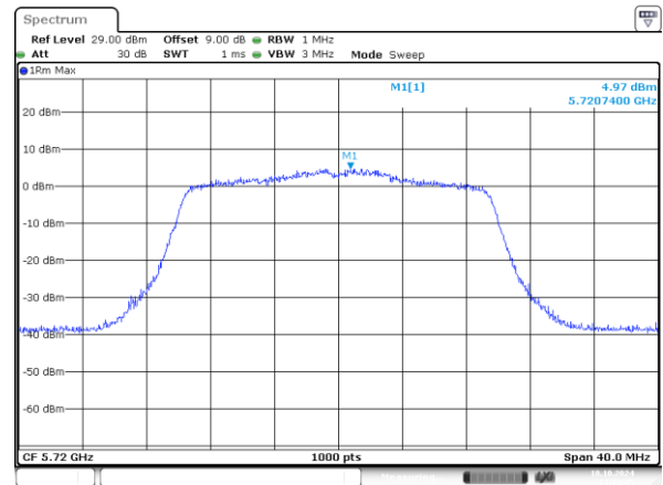
802.11ax20_5720MHz_RU_242/61_Chain 1
