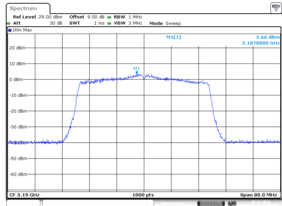
802.11ax40_5190MHz_RU_484/65_Chain 1
