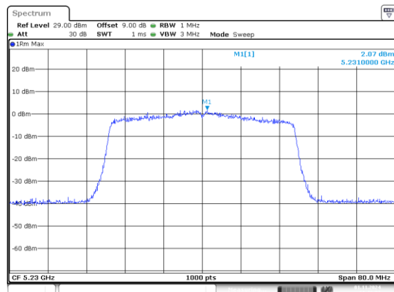
802.11ax40_5230MHz_RU_484/65_Chain 0
