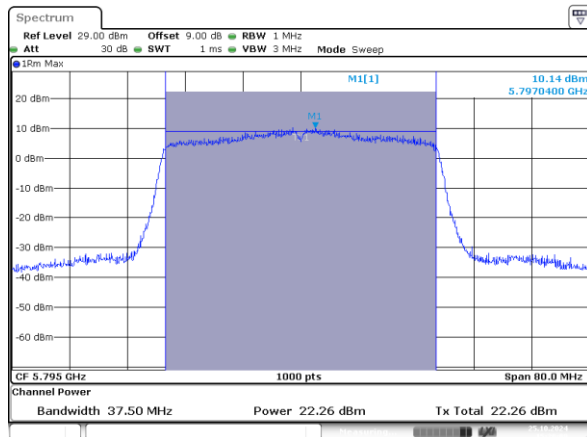
802.11ax40_5795MHz_RU_484/65_Chain 0
