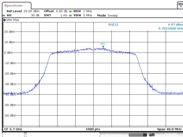
802.11ax20_5700MHz_RU_242/61_Chain 0
