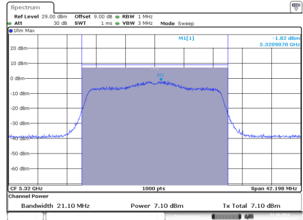
802.11ax20_5320MHz_RU_242/61_Chain 1
