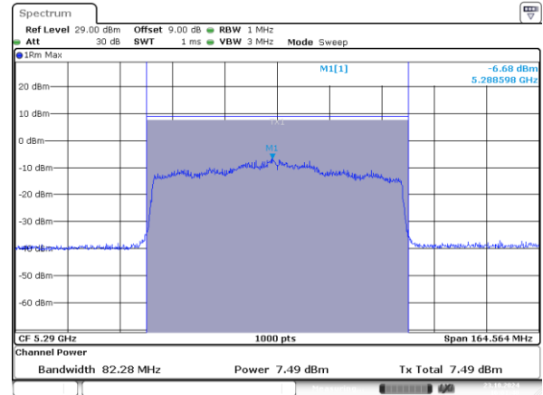
802.11ax80_5290MHz_RU_996/67_Chain 1
