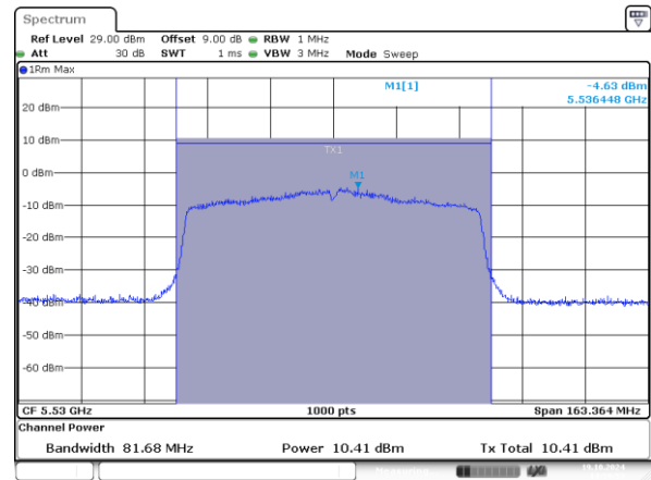
802.11ax80_5530MHz_RU_996/67_Chain 1
