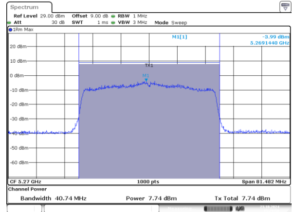
802.11ax40_5270MHz_RU_484/65_Chain 1
