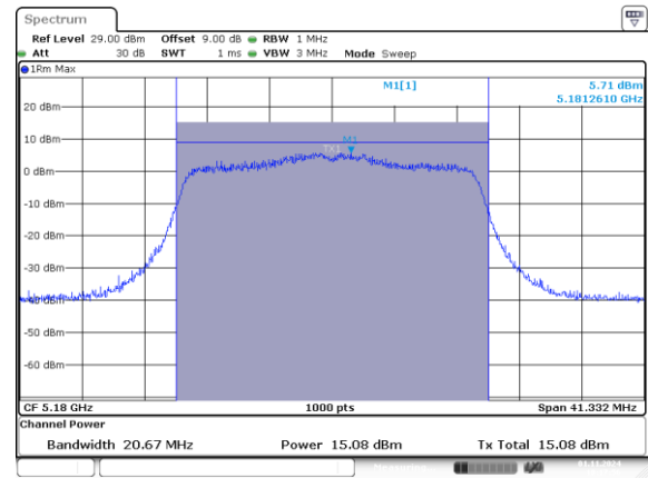
802.11ax20_5180MHz_RU_242/61_Chain 1
