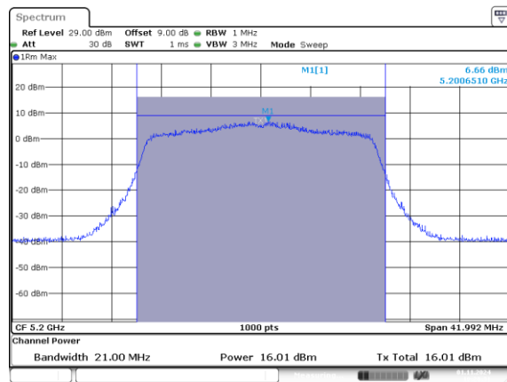
802.11ax20_5200MHz_RU_242/61_Chain 0
