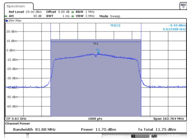
802.11ax80_5610MHz_RU_996/67_Chain 1
