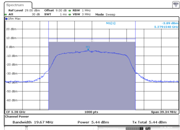
802.11a_5280MHz_Chain 1
