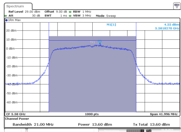
802.11ax20_5580MHz_RU_242/61_Chain 1
