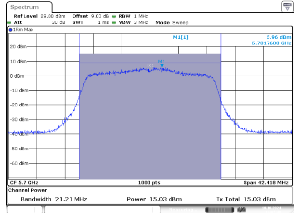
802.11ax20_5700MHz_RU_242/61_Chain 1
