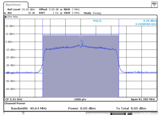
802.11ax40_5310MHz_RU_484/65_Chain 1
