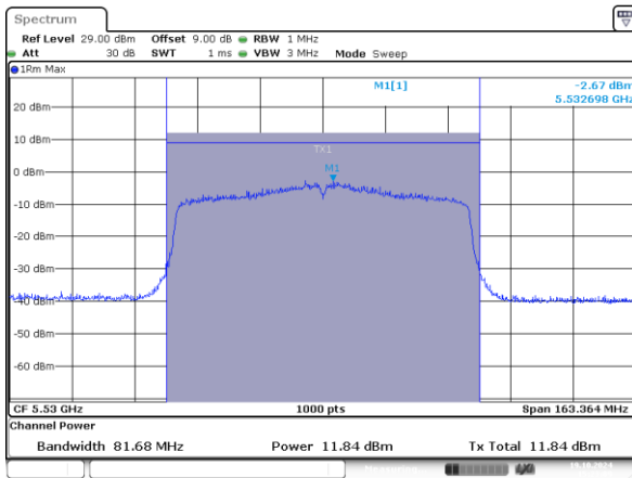
802.11ax80_5530MHz_RU_996/67_Chain 0
