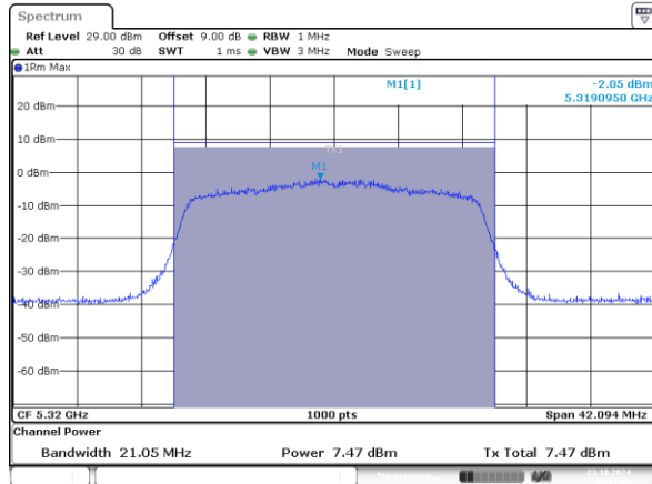
802.11ax20_5320MHz_RU_242/61_Chain 0
