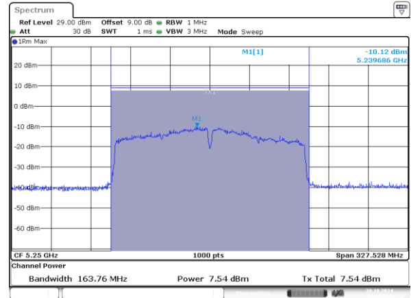
802.11ac160_5250MHz_Chain 1
