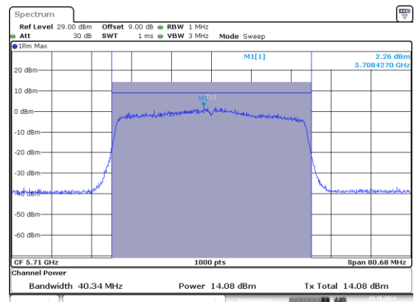
802.11ax40_5710MHz_RU_484/65_Chain 1
