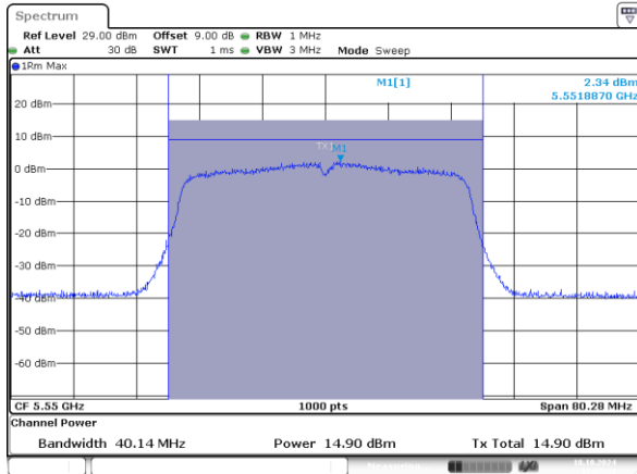
802.11n40_5550MHz_Chain 0
