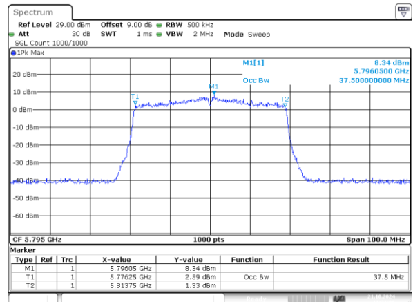
802.11ax40_5795MHz_RU_484/65_Chain 1 37.500MHz
