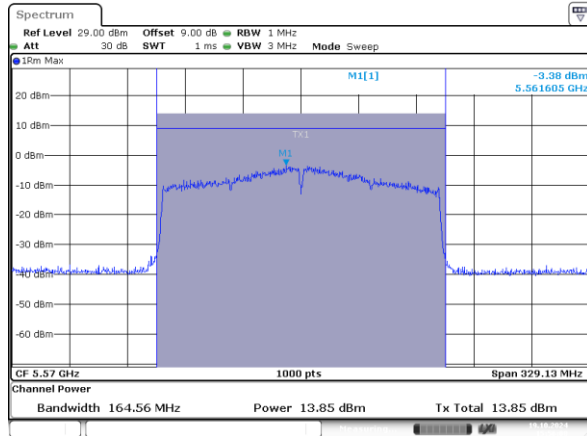
802.11ax160_5570MHz_RU_2*996_Chain 0
