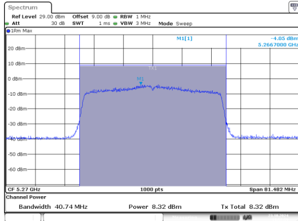
802.11ax40_5270MHz_RU_484/65_Chain 0
