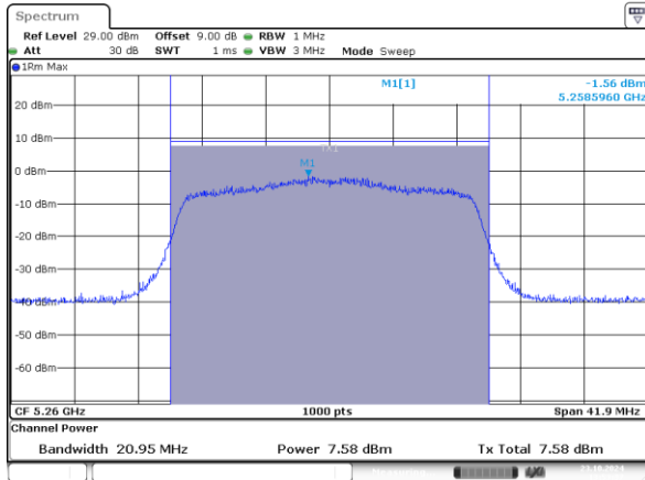
802.11ax20_5260MHz_RU_242/61_Chain 0
