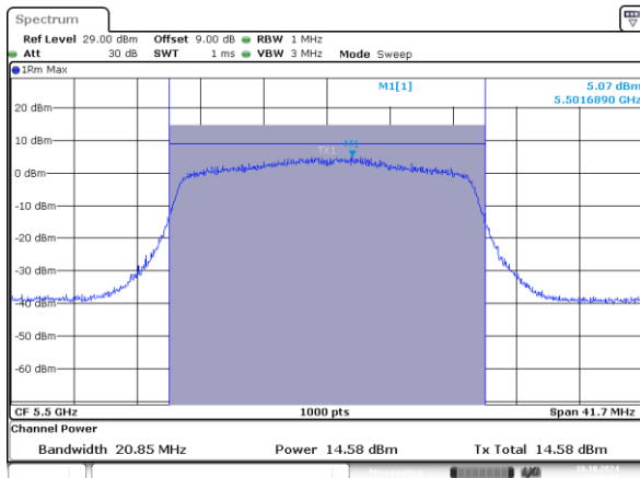
802.11ax20_5500MHz_RU_242/61_Chain 0
