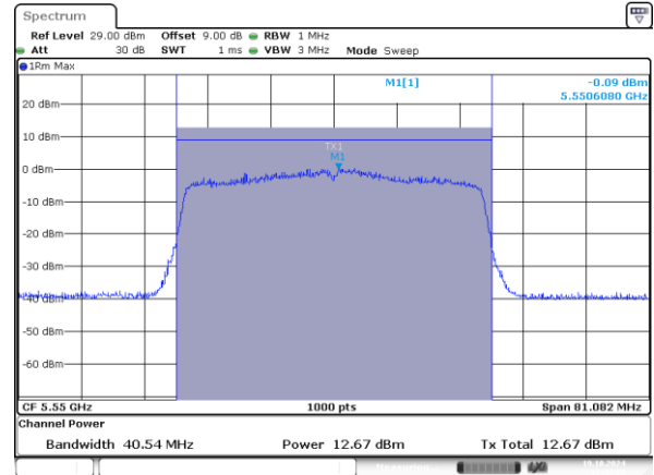
802.11ax40_5550MHz_RU_484/65_Chain 1
