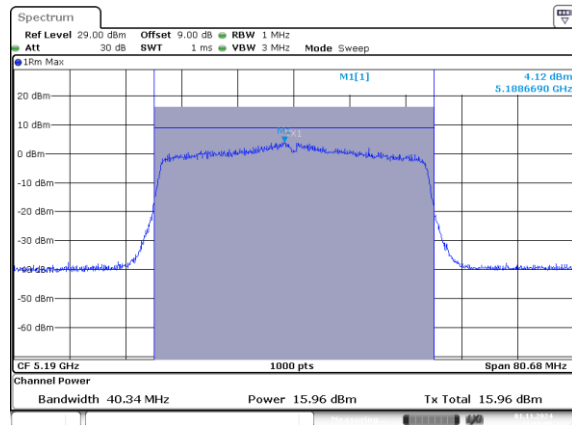
802.11ax40_5190MHz_RU_484/65_Chain 0
