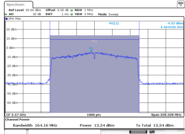
802.11ax160_5570MHz_RU_2*996_Chain 1
