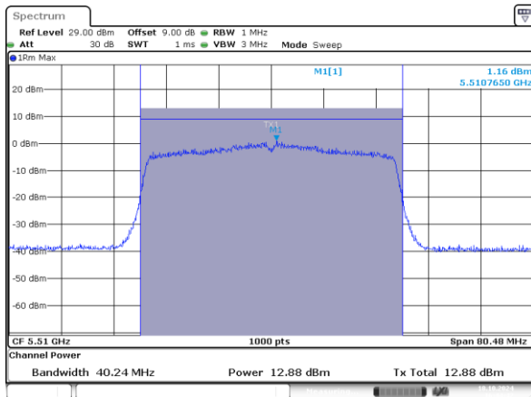
802.11ax40_5510MHz_RU_484/65_Chain 0
