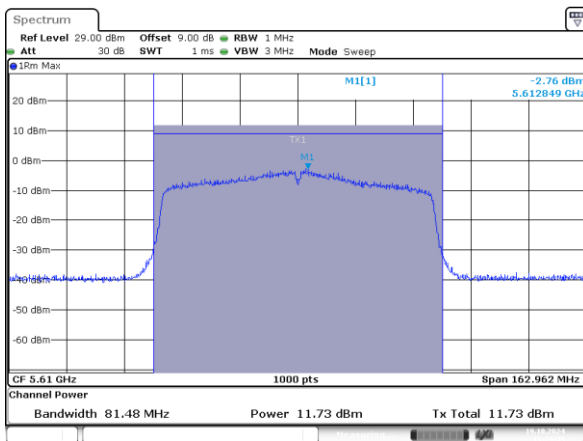
802.11ax80_5610MHz_RU_996/67_Chain 0
