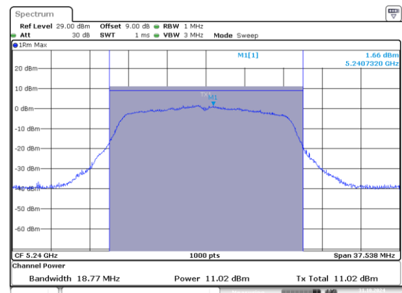
802.11a_5240MHz_Chain 1
