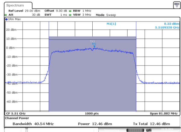
802.11ax40_5510MHz_RU_484/65_Chain 1
