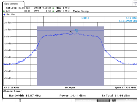
802.11a_5180MHz_Chain 0
