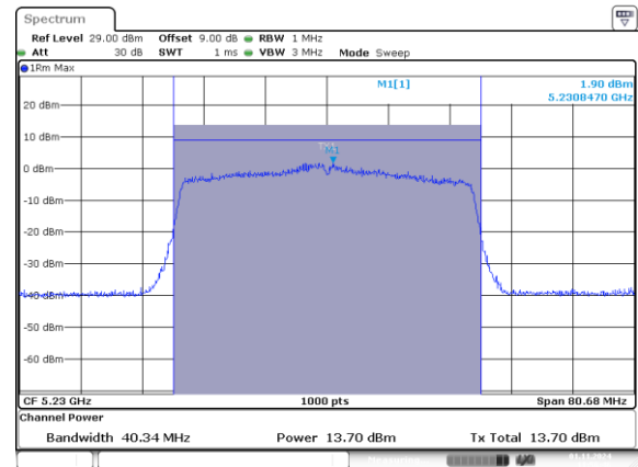
802.11ax40_5230MHz_RU_484/65_Chain 1
