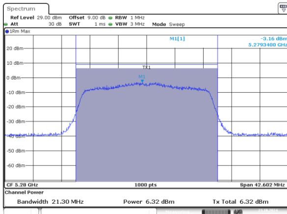
802.11ax20_5280MHz_RU_242/61_Chain 0
