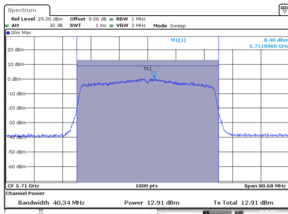
802.11ax40_5710MHz_RU_484/65_Chain 0
