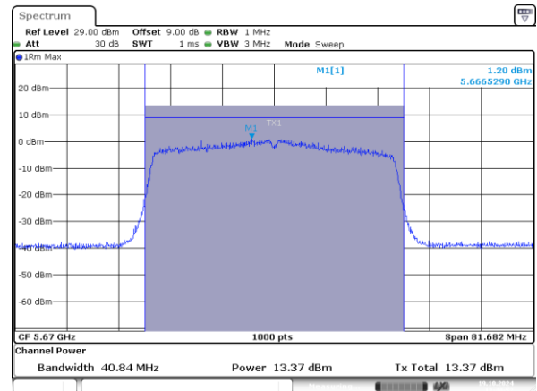
802.11ax40_5670MHz_RU_484/65_Chain 1
