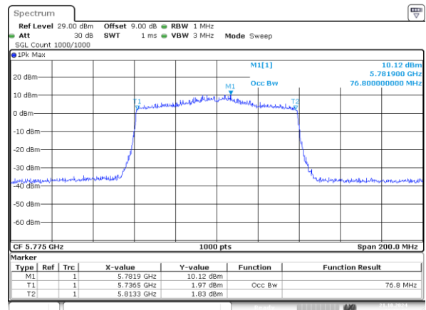
802.11ax80_5775MHz_RU_996/67_Chain 1 76.800MHz
