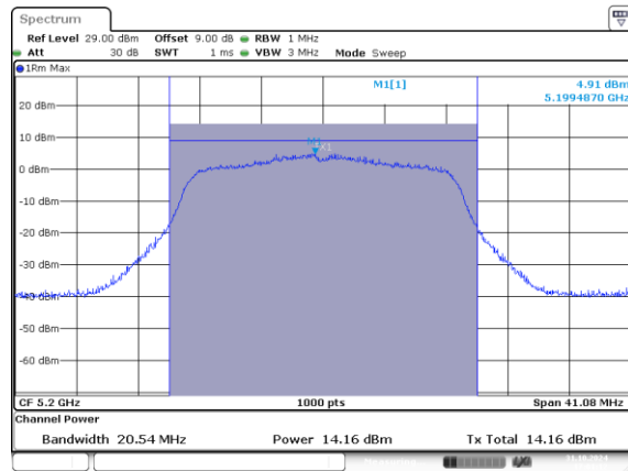
802.11n20_5200MHz_Chain 0
