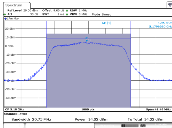
802.11n20_5180MHz_Chain 0
