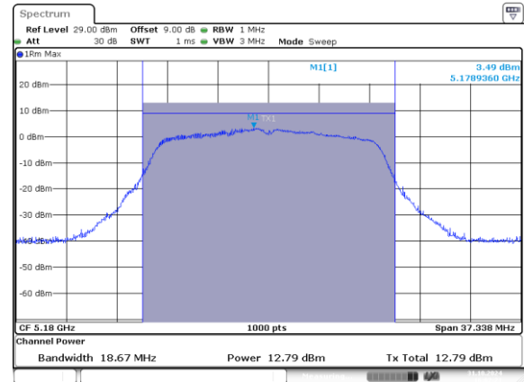
802.11a_5180MHz_Chain 1
