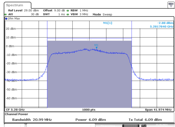
802.11ax20_5280MHz_RU_242/61_Chain 1
