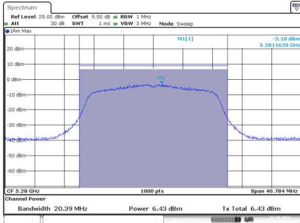
802.11n20_5280MHz_Chain 0
