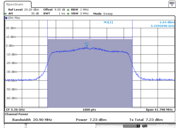
802.11ax20_5260MHz_RU_242/61_Chain 1
