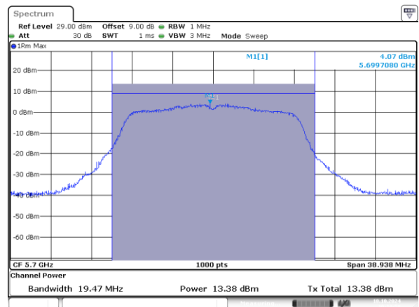
802.11a_5700MHz_Chain 1
