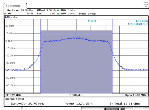
802.11ax20_5240MHz_RU_242/61_Chain 1
