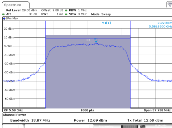
802.11a_5580MHz_Chain 0
