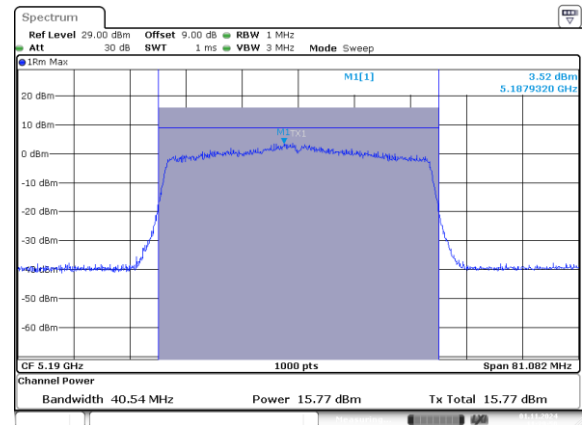
802.11ax40_5190MHz_RU_484/65_Chain 1
