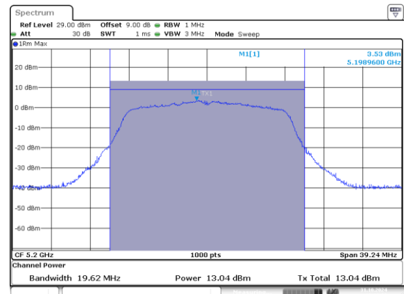
802.11a_5200MHz_Chain 1
