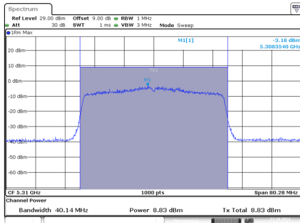
802.11ax40_5310MHz_RU_484/65_Chain 0
