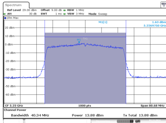
802.11ax40_5230MHz_RU_484/65_Chain 0
