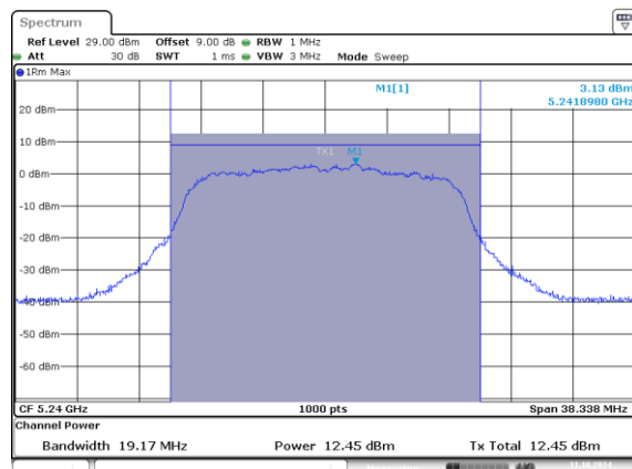
802.11a_5240MHz_Chain 0
