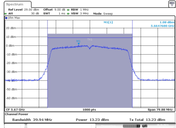
802.11n40_5670MHz_Chain 1
