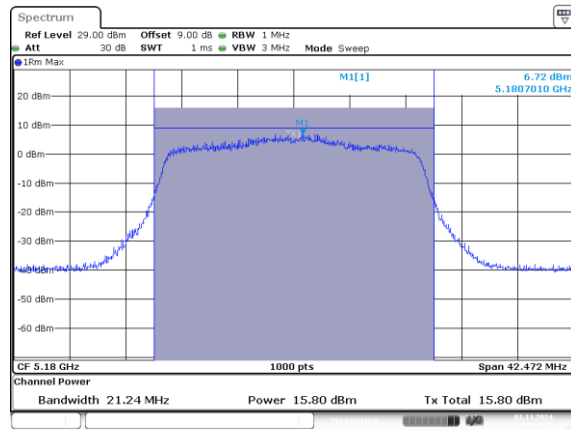
802.11ax20_5180MHz_RU_242/61_Chain 0
