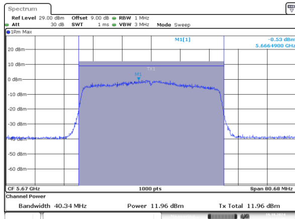
802.11ax40_5670MHz_RU_484/65_Chain 0
