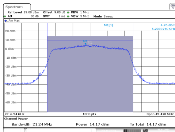
802.11ax20_5240MHz_RU_242/61_Chain 0
