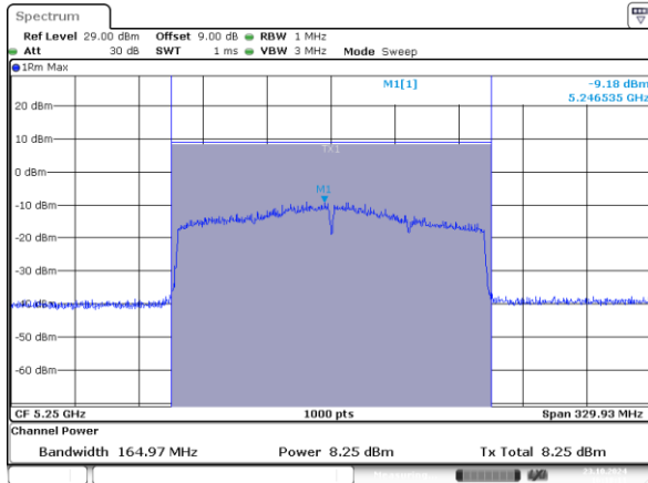
802.11ax160_5250MHz_RU_2*996_Chain 0
