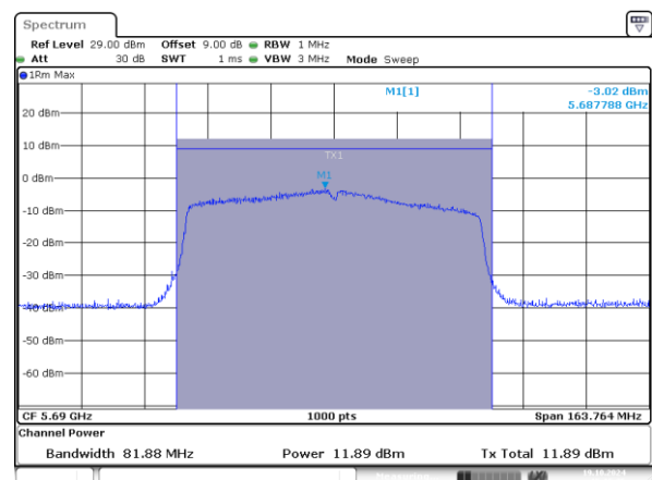
802.11ax80_5690MHz_RU_996/67_Chain 1
