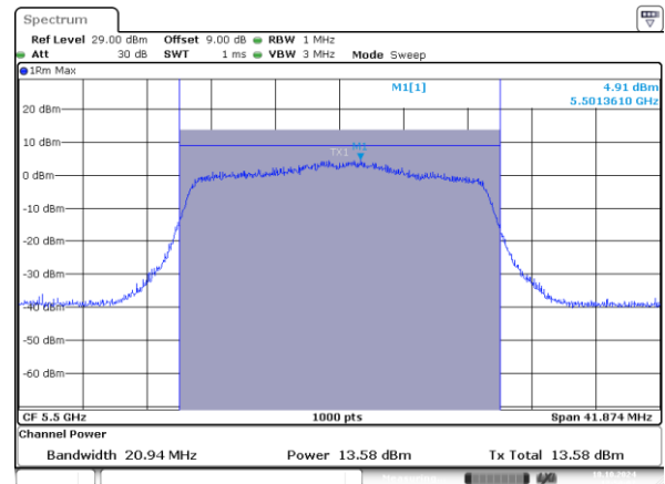
802.11ax20_5500MHz_RU_242/61_Chain 1
