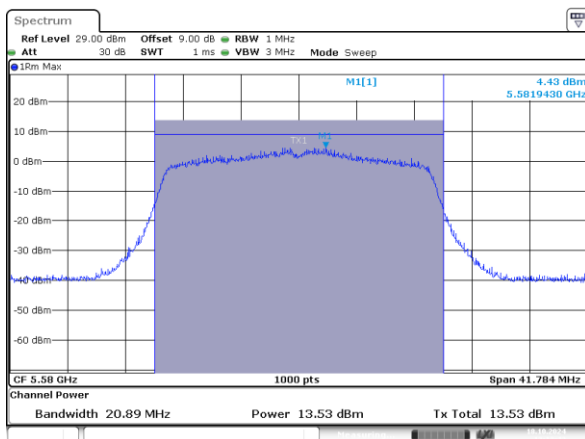
802.11ax20_5580MHz_RU_242/61_Chain 0
