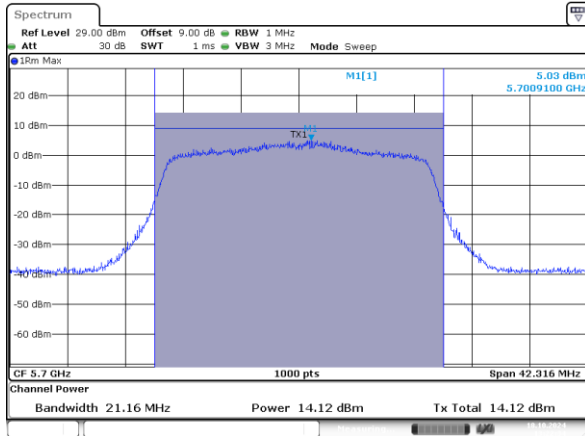
802.11ax20_5700MHz_RU_242/61_Chain 0
