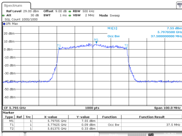
802.11ax40_5795MHz_RU_484/65_Chain 0 37.500MHz
