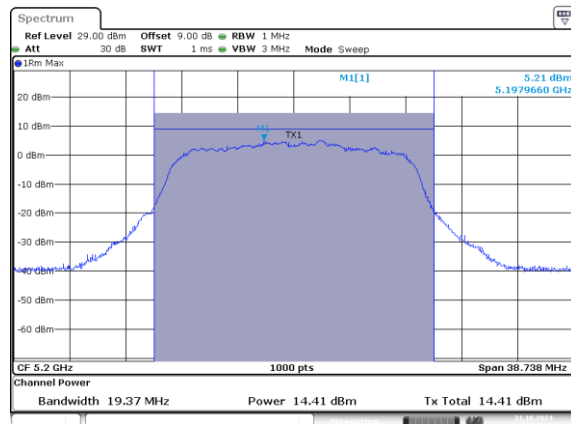
802.11a_5200MHz_Chain 0
