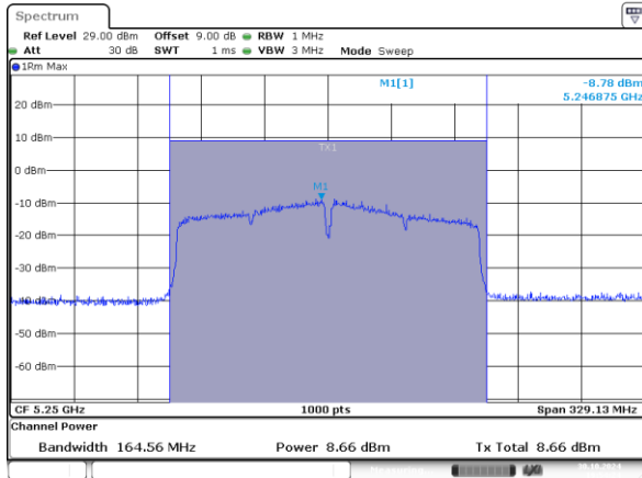
802.11ac160_5250MHz_Chain 0
