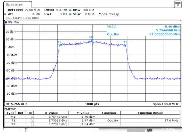
802.11ax40_5755MHz_RU_484/65_Chain 1 37.600MHz
