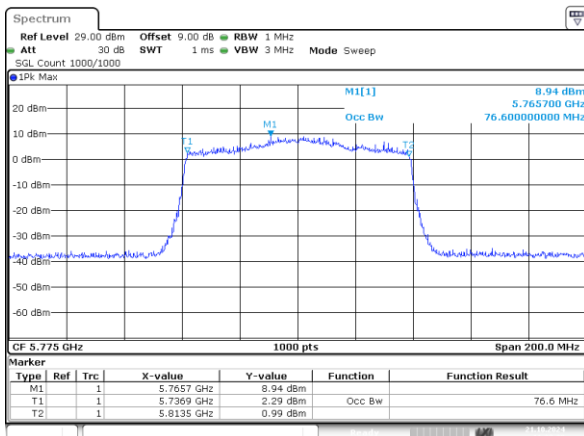
802.11ax80_5775MHz_RU_996/67_Chain 0 76.600MHz
