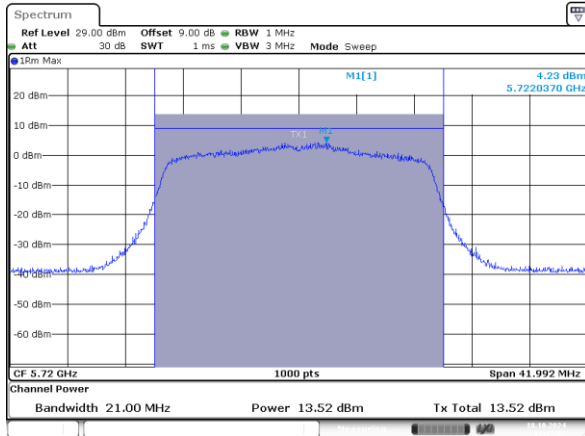
802.11ax20_5720MHz_RU_242/61_Chain 0
