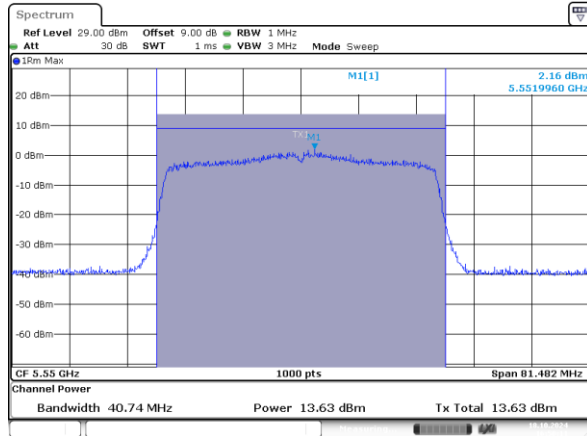
802.11ax40_5550MHz_RU_484/65_Chain 0
