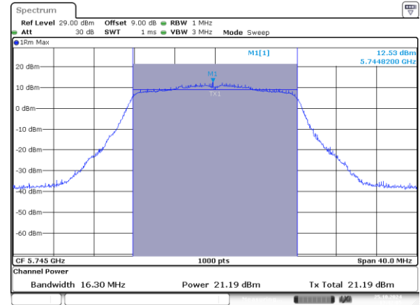
802.11a_5745MHz_Chain 1
