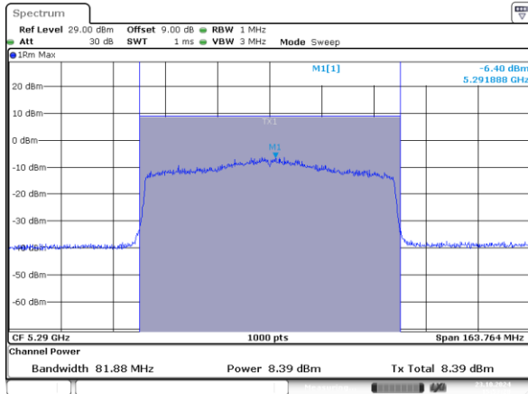
802.11ax80_5290MHz_RU_996/67_Chain 0
