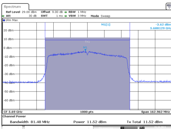
802.11ax80_5690MHz_RU_996/67_Chain 0
