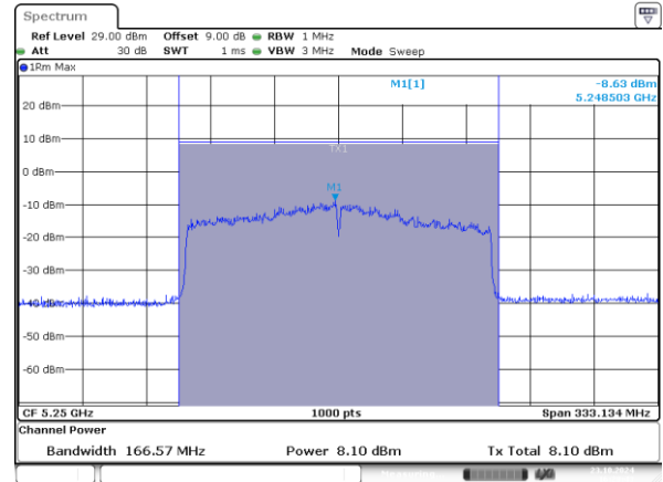
802.11ax160_5250MHz_RU_2*996_Chain 1
