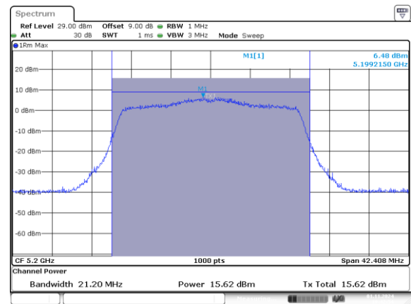
802.11ax20_5200MHz_RU_242/61_Chain 1
