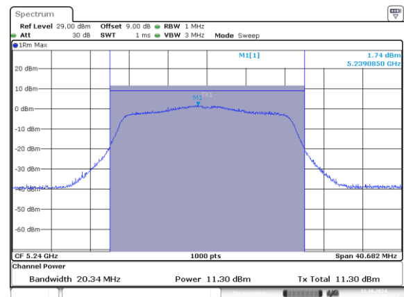
802.11n20_5240MHz_Chain 1
