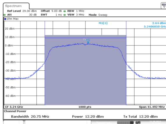
802.11n20_5240MHz_Chain 0
