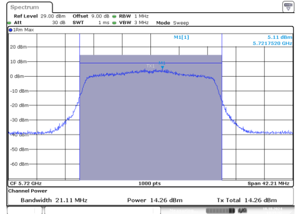
802.11ax20_5720MHz_RU_242/61_Chain 1
