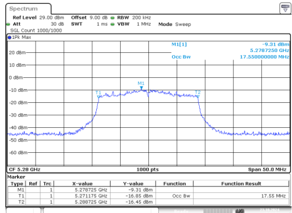
802.11n20_5280MHz_Chain 1 17.550MHz
