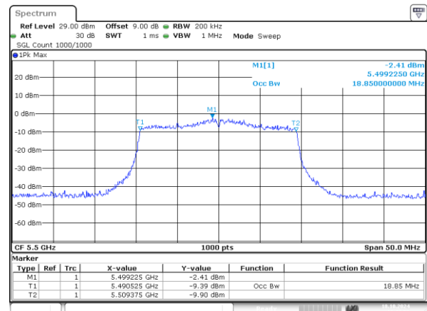
802.11ax20_5500MHz_RU_242/61_Chain 1 18.850MHz
