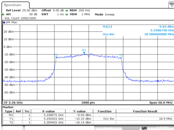
802.11ax20_5260MHz_RU_242/61_Chain 0 18.900MHz
