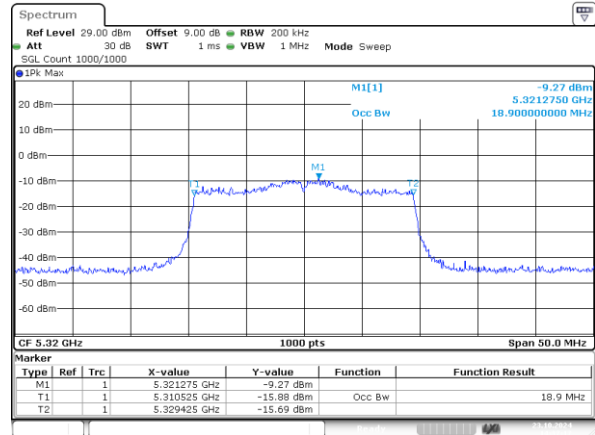
802.11ax20_5320MHz_RU_242/61_Chain 1 18.900MHz
