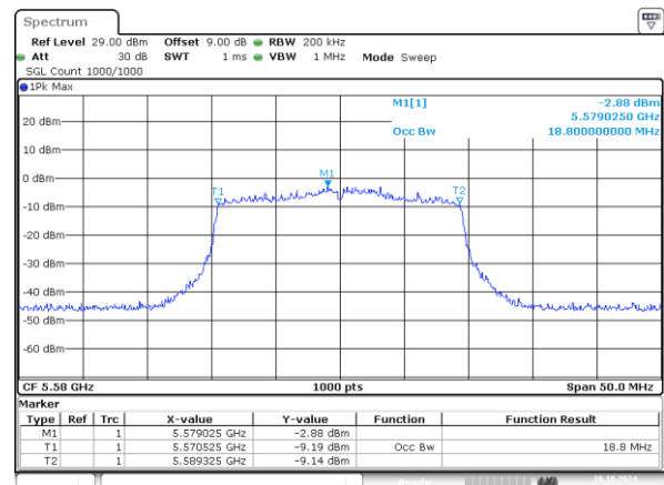
802.11ax20_5580MHz_RU_242/61_Chain 1 18.800MHz
