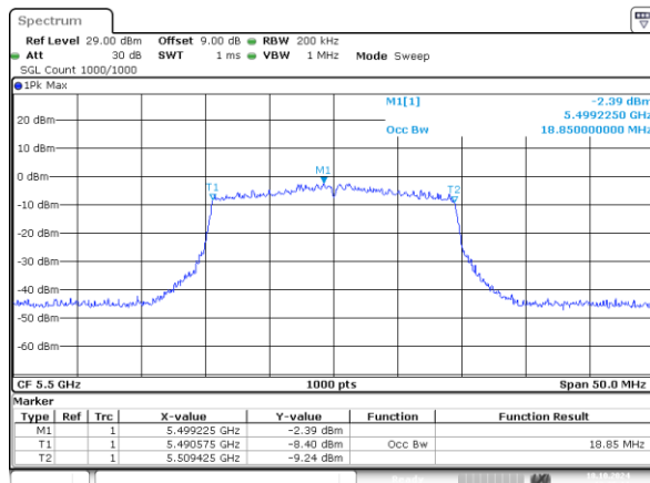
802.11ax20_5500MHz_RU_242/61_Chain 0 18.850MHz
