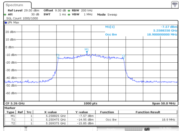
802.11ax20_5260MHz_RU_242/61_Chain 1 18.900MHz
