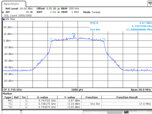
802.11n20_5745MHz_Chain 0 17.500MHz
