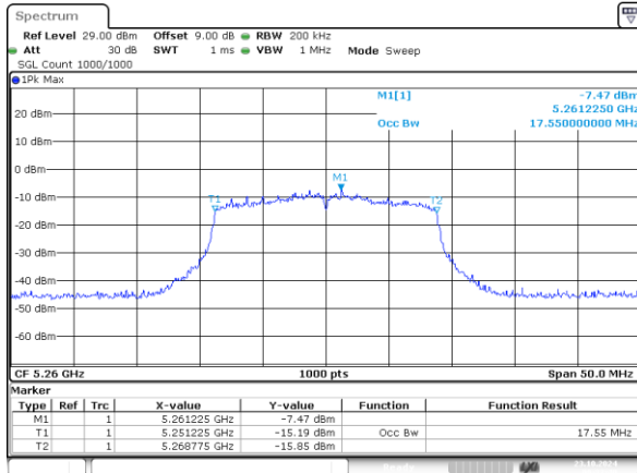
802.11n20_5260MHz_Chain 0 17.550MHz
