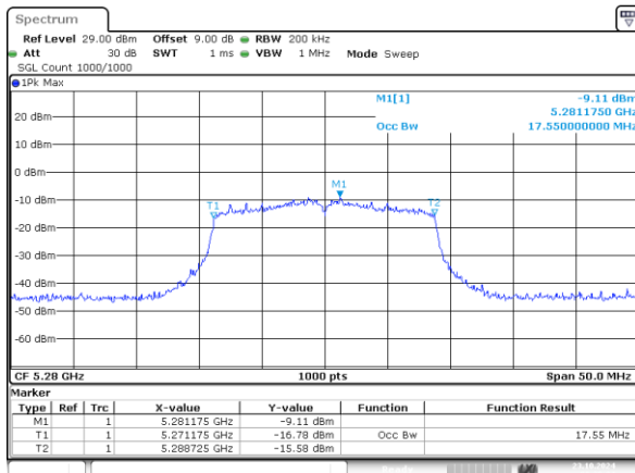
802.11n20_5280MHz_Chain 0 17.550MHz
