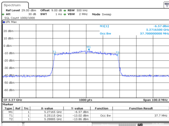
802.11ax40_5270MHz_RU_484/65_Chain 0 37.700MHz
