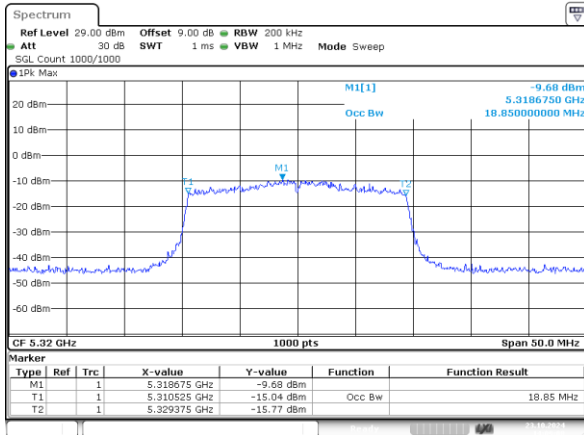
802.11ax20_5320MHz_RU_242/61_Chain 0 18.850MHz
