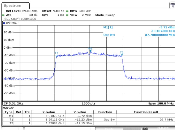
802.11ax40_5310MHz_RU_484/65_Chain 0 37.700MHz
