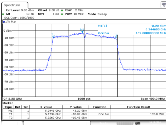
802.11ac160_5250MHz_Chain 0 152.800MHz
