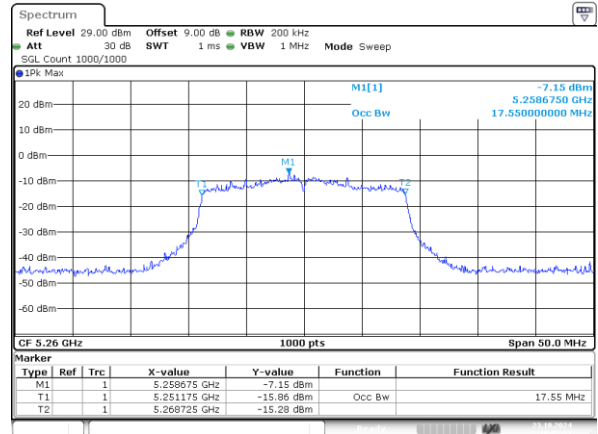
802.11n20_5260MHz_Chain 1 17.550MHz
