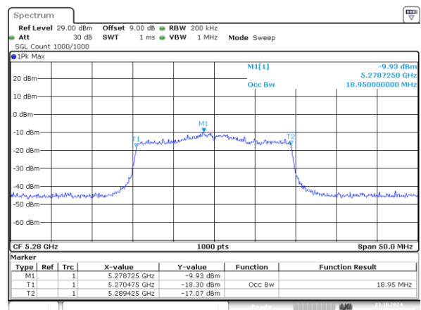
802.11ax20_5280MHz_RU_242/61_Chain 1 18.950MHz
