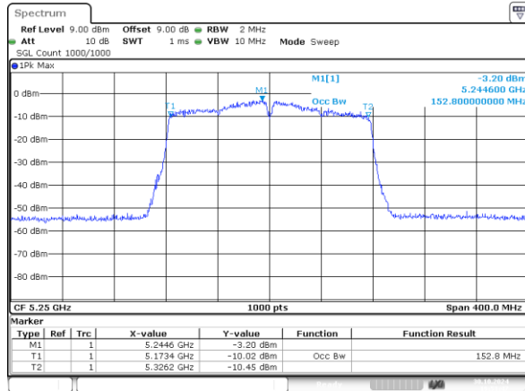
802.11ac160_5250MHz_Chain 0 152.800MHz
