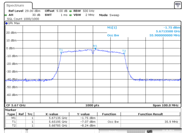
802.11n40_5670MHz_Chain 1 35.900MHz
