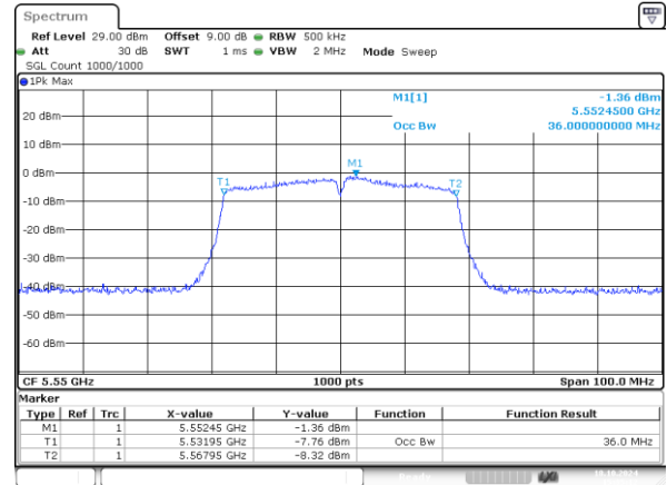
802.11n40_5550MHz_Chain 1 36MHz
