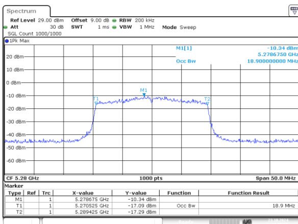
802.11ax20_5280MHz_RU_242/61_Chain 0 18.900MHz
