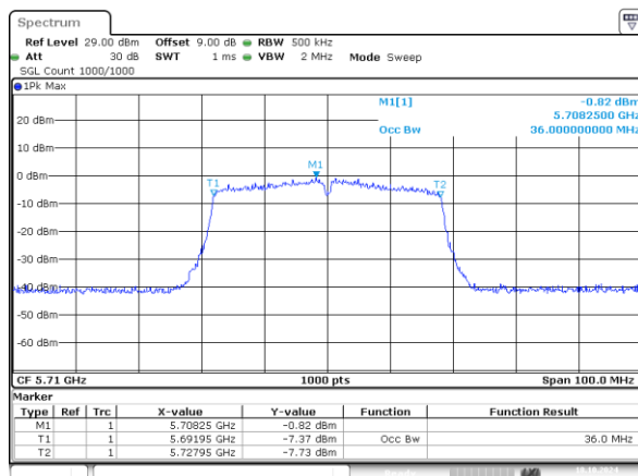
802.11n40_5710MHz_Chain 0 36MHz
