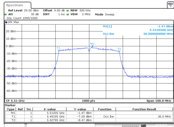
802.11n40_5510MHz_Chain 1 36MHz
