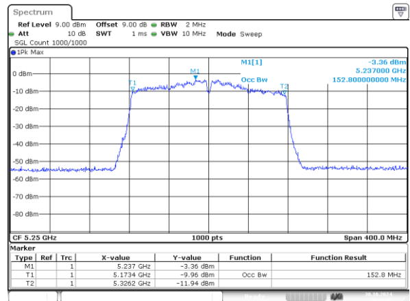
802.11ac160_5250MHz_Chain 1 152.800MHz
