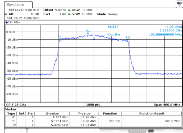
802.11ac160_5250MHz_Chain 1 152.800MHz
