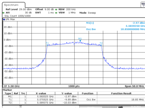
802.11ax20_5580MHz_RU_242/61_Chain 0 18.850MHz
