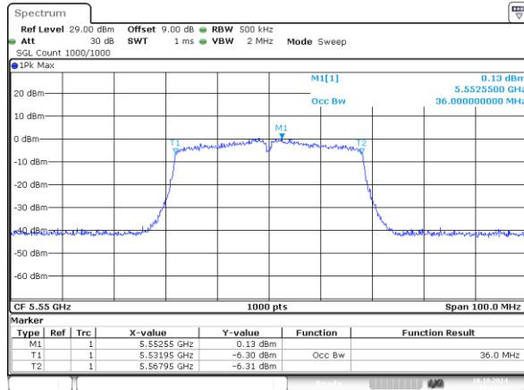
802.11n40_5550MHz_Chain 0 36MHz
