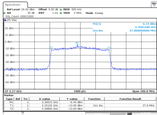
802.11ax40_5270MHz_RU_484/65_Chain 1 37.800MHz
