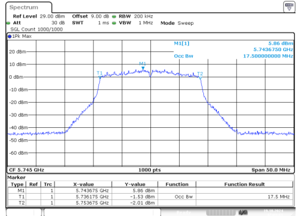
802.11n20_5745MHz_Chain 1 17.500MHz
