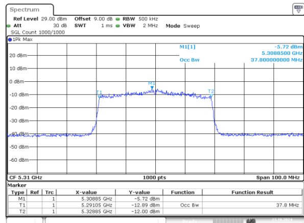
802.11ax40_5310MHz_RU_484/65_Chain 1 37.800MHz
