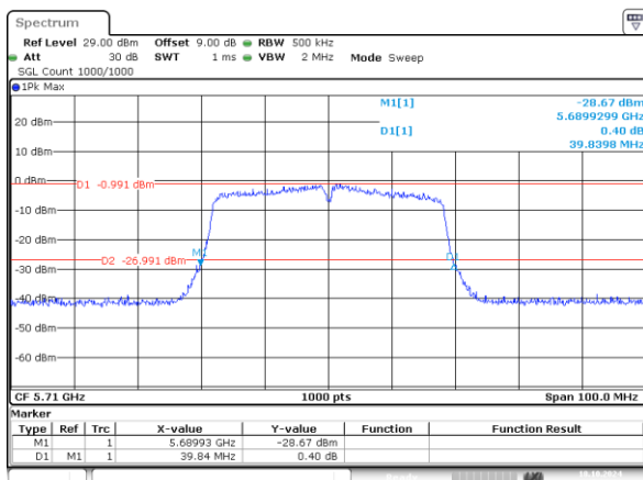
802.11n40_5710MHz_Chain 0 39.840MHz
