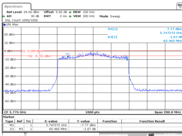
802.11ax80_5775MHz_RU_996/67_Chain 0 65.465MHz
