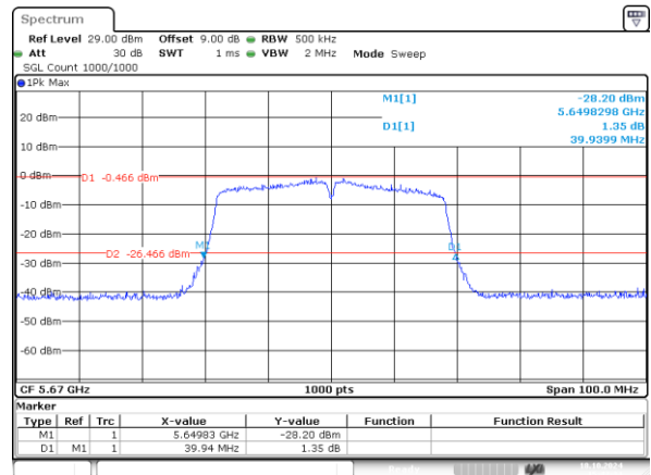
802.11n40_5670MHz_Chain 1 39.940MHz
