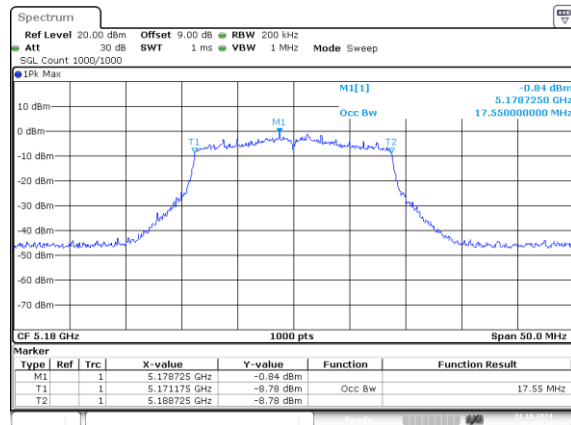
802.11n20_5180MHz_Chain 0 17.550MHz
