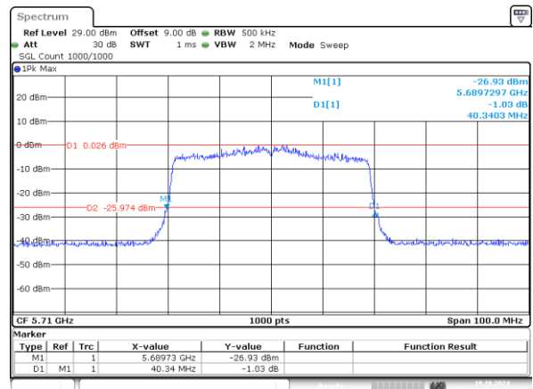
802.11ax40_5710MHz_RU_484/65_Chain 1 40.340MHz
