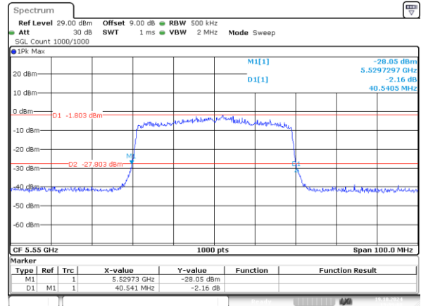
802.11ax40_5550MHz_RU_484/65_Chain 1 40.541MHz
