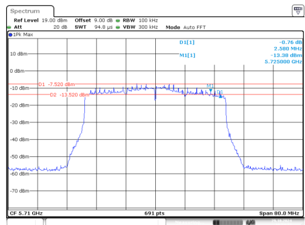
802.11ax40_5710MHz_RU_484/65_Chain 1 2.580MHz
