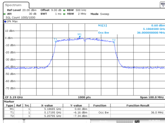
802.11n40_5190MHz_Chain 0 36MHz
