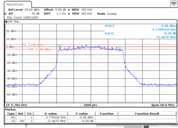
802.11ax20_5785MHz_RU_242/61_Chain 1 17.467MHz
