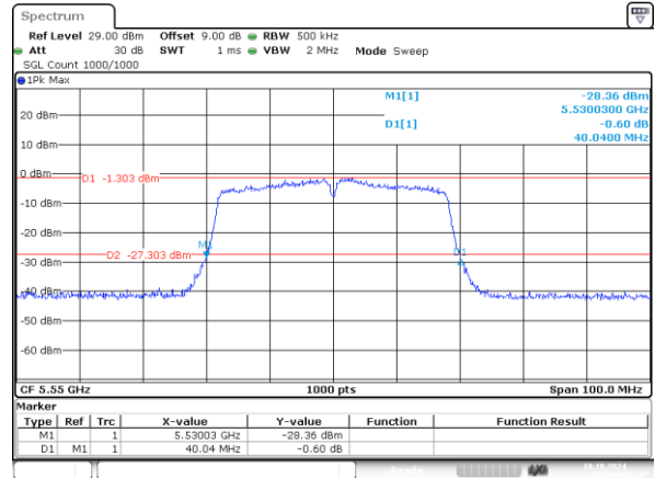
802.11n40_5550MHz_Chain 1 40.040MHz
