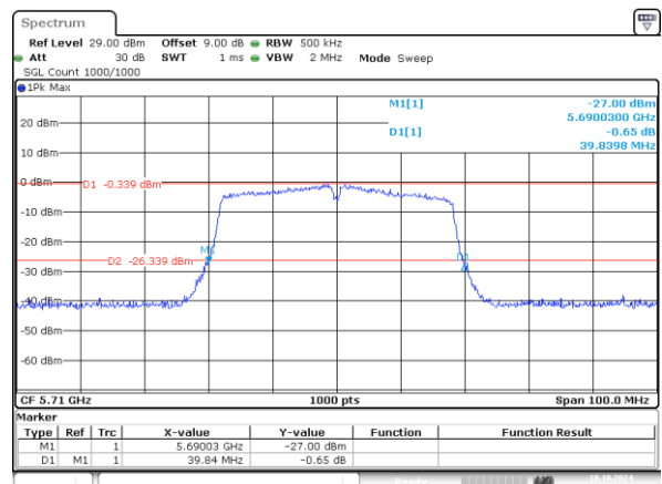
802.11n40_5710MHz_Chain 1 39.840MHz
