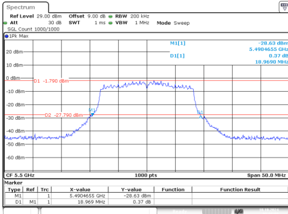
802.11a_5500MHz_Chain 0 18.969MHz
