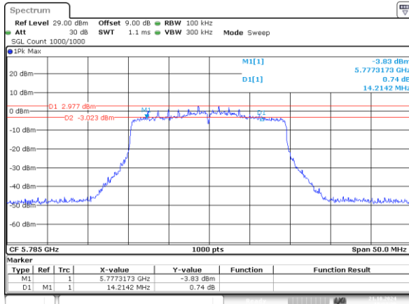
802.11ax20_5785MHz_RU_242/61_Chain 0 14.214MHz
