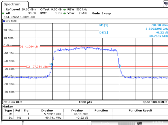
802.11ax40_5550MHz_RU_484/65_Chain 0 40.741MHz
