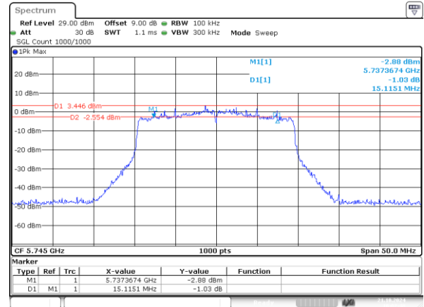
802.11ax20_5745MHz_RU_242/61_Chain 1 15.115MHz
