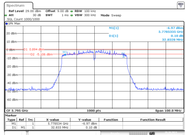
802.11n40_5795MHz_Chain 1 32.833MHz
