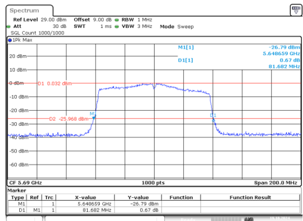
802.11ac80_5690MHz_Chain 1 81.682MHz
