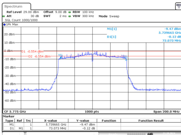
802.11ac80_5775MHz_Chain 0 73.073MHz
