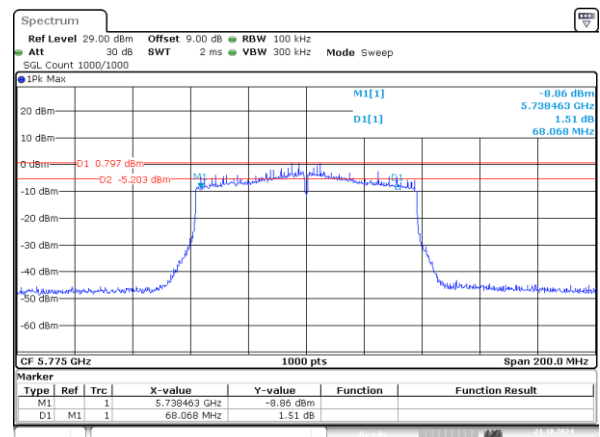
802.11ac80_5775MHz_Chain 1 68.068MHz
