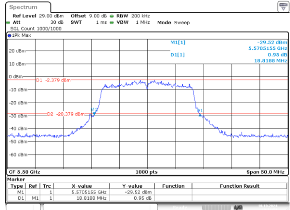
802.11a_5580MHz_Chain 1 18.819MHz
