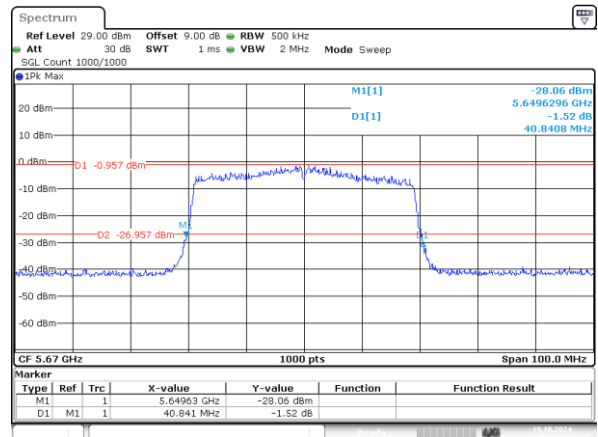
802.11ax40_5670MHz_RU_484/65_Chain 1 40.841MHz
