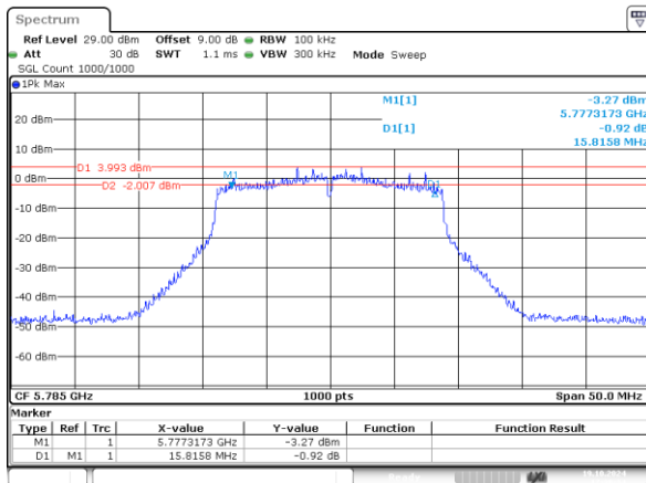
802.11n20_5785MHz_Chain 0 15.816MHz
