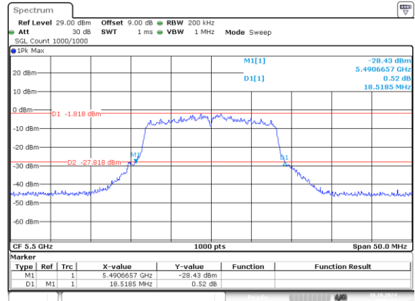
802.11a_5500MHz_Chain 1 18.519MHz
