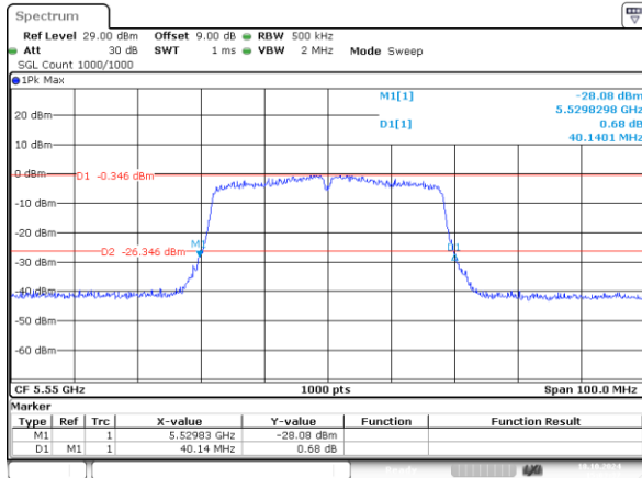
802.11n40_5550MHz_Chain 0 40.140MHz
