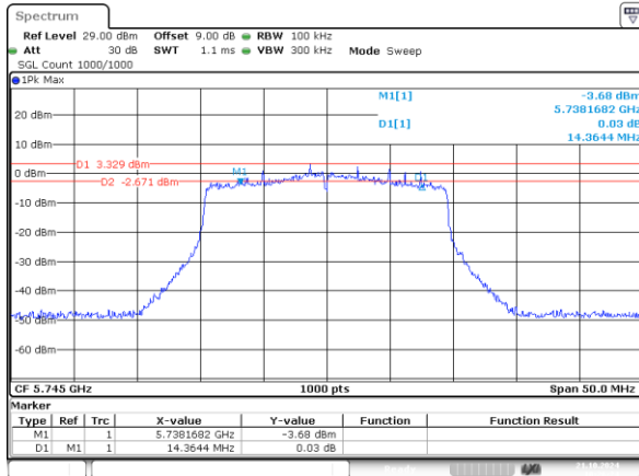
802.11ax20_5745MHz_RU_242/61_Chain 0 14.364MHz
