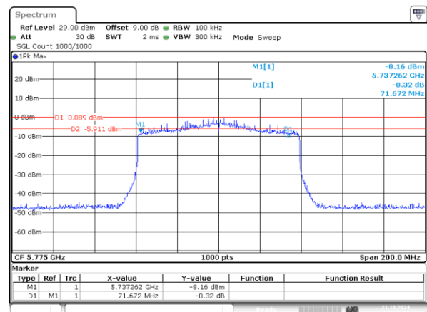
802.11ax80_5775MHz_RU_996/67_Chain 1 71.672MHz
