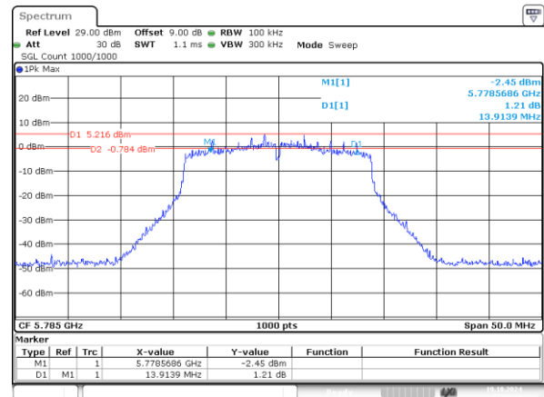
802.11n20_5785MHz_Chain 1 13.914MHz
