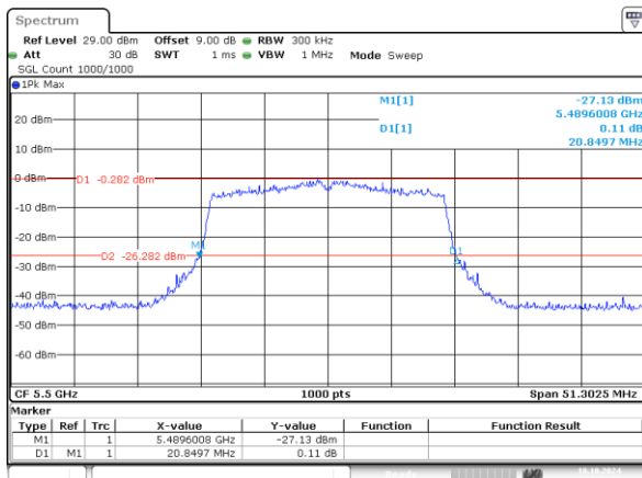
802.11ax20_5500MHz_RU_242/61_Chain 0 20.850MHz
