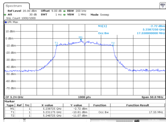
802.11n20_5240MHz_Chain 1 17.550MHz
