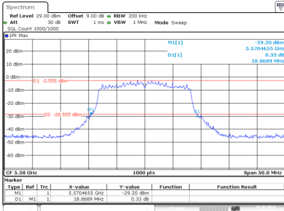
802.11a_5580MHz_Chain 0 18.869MHz
