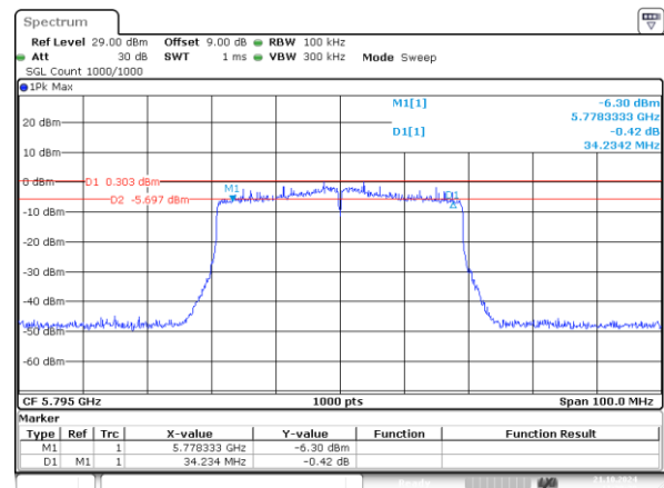
802.11ax40_5795MHz_RU_484/65_Chain 1 34.234MHz
