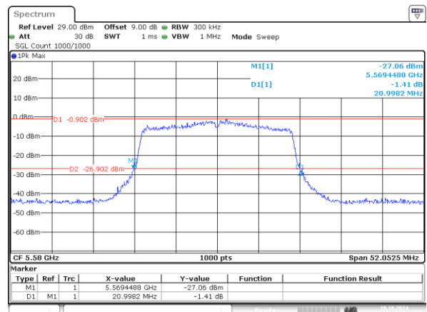
802.11ax20_5580MHz_RU_242/61_Chain 1 20.998MHz
