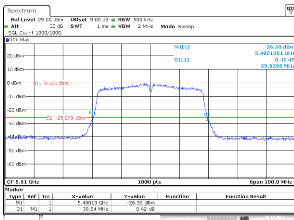
802.11n40_5510MHz_Chain 0 39.540MHz
