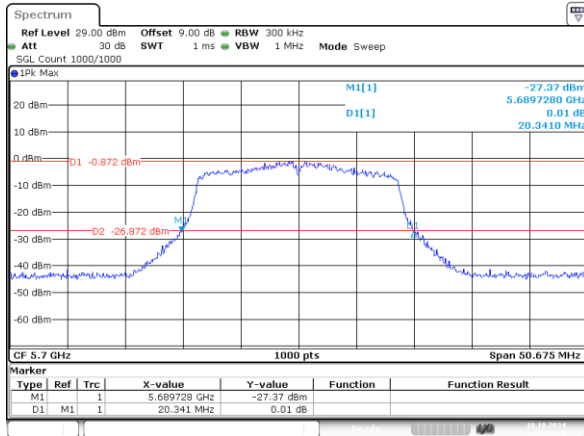
802.11n20_5700MHz_Chain 0 20.341MHz
