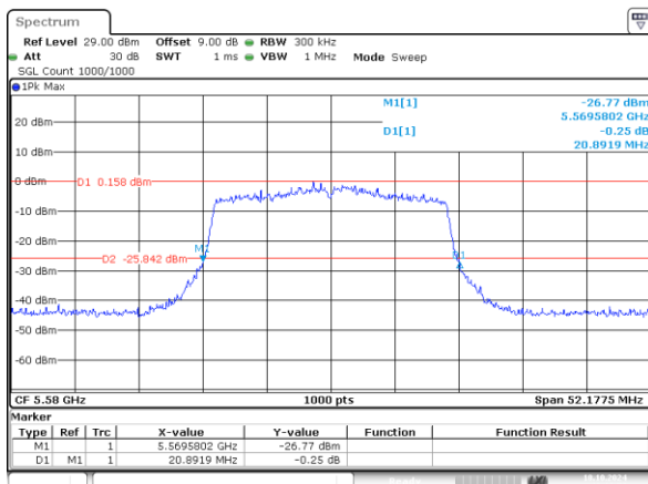
802.11ax20_5580MHz_RU_242/61_Chain 0 20.892MHz
