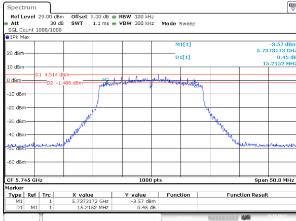
802.11n20_5745MHz_Chain 0 15.215MHz
