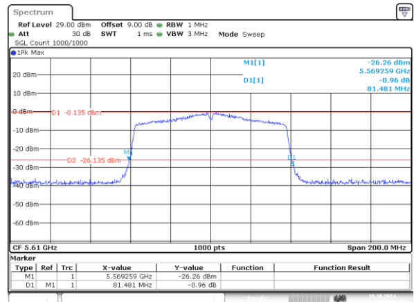
802.11ac80_5610MHz_Chain 1 81.481MHz
