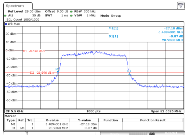
802.11ax20_5500MHz_RU_242/61_Chain 1 20.937MHz
