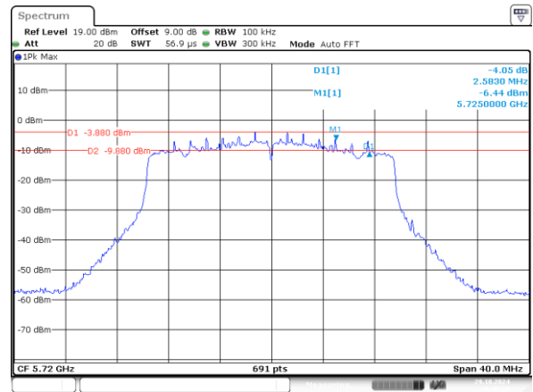
802.11ax20_5720MHz_RU_242/61_Chain 1 2.583MHz
