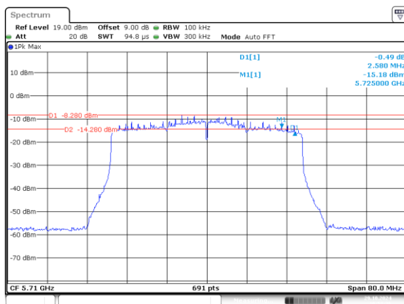
802.11ax40_5710MHz_RU_484/65_Chain 0 2.580MHz
