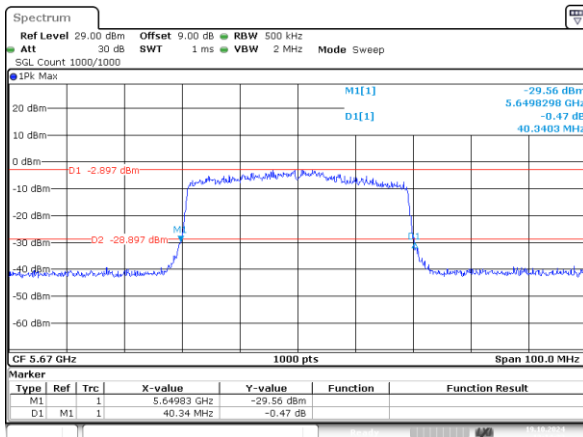
802.11ax40_5670MHz_RU_484/65_Chain 0 40.340MHz
