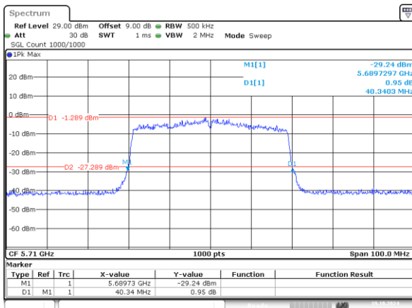
802.11ax40_5710MHz_RU_484/65_Chain 0 40.340MHz
