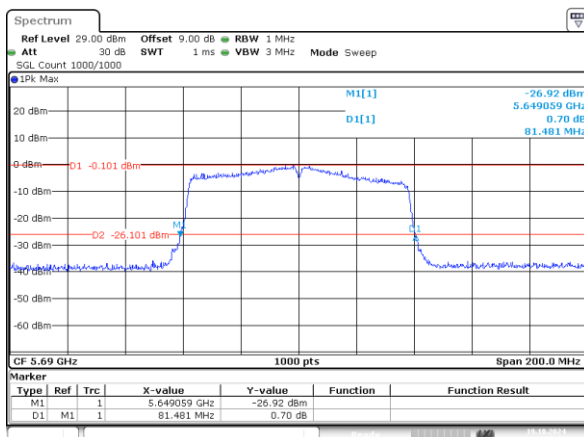
802.11ac80_5690MHz_Chain 0 81.481MHz
