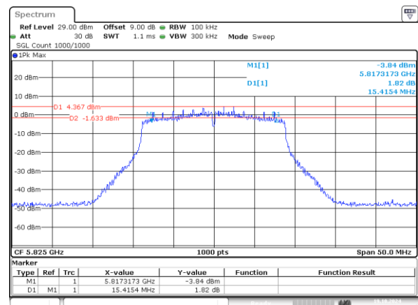
802.11n20_5825MHz_Chain 1 15.415MHz
