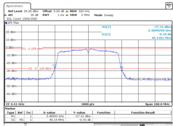
802.11n40_5510MHz_Chain 1 40.140MHz
