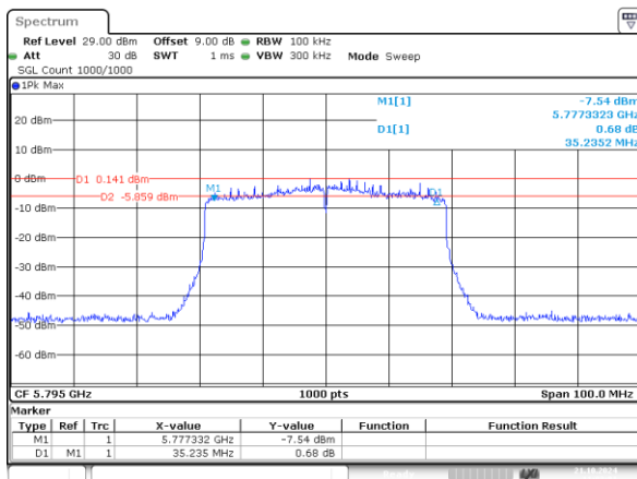
802.11ax40_5795MHz_RU_484/65_Chain 0 35.235MHz
