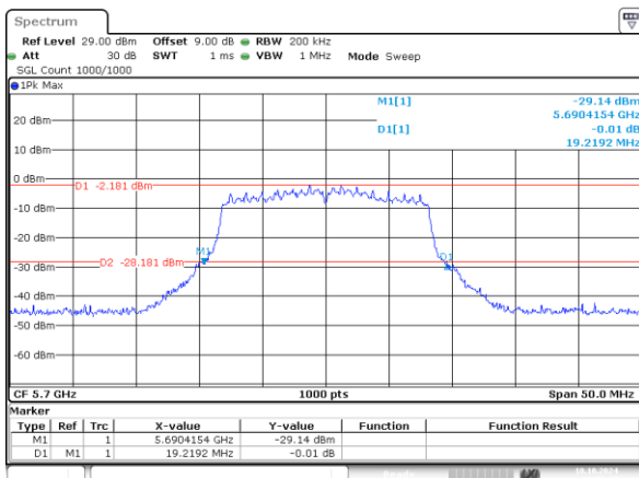
802.11a_5700MHz_Chain 0 19.219MHz
