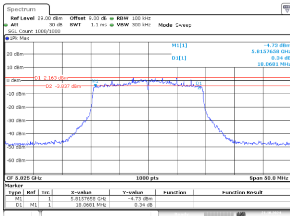
802.11ax20_5825MHz_RU_242/61_Chain 0 18.068MHz
