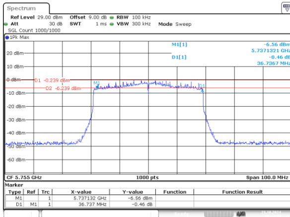
802.11ax40_5755MHz_RU_484/65_Chain 0 36.737MHz
