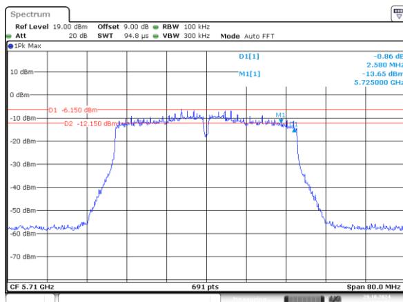
802.11n40_5710MHz_Chain 0 2.580MHz
