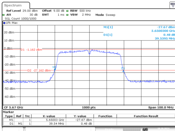
802.11n40_5670MHz_Chain 0 39.540MHz
