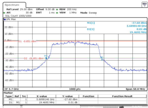
802.11a_5700MHz_Chain 1 19.469MHz
