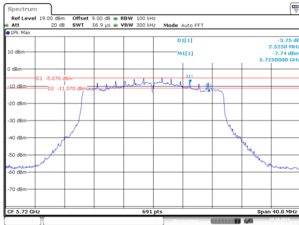
802.11ax20_5720MHz_RU_242/61_Chain 0 2.525MHz
