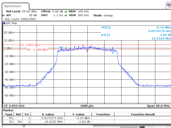
802.11n20_5825MHz_Chain 0 15.215MHz
