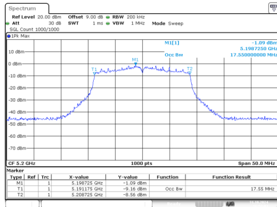
802.11n20_5200MHz_Chain 0 17.550MHz
