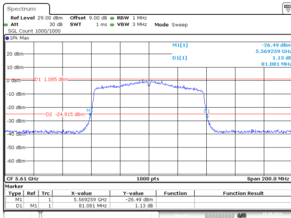
802.11ac80_5610MHz_Chain 0 81.081MHz
