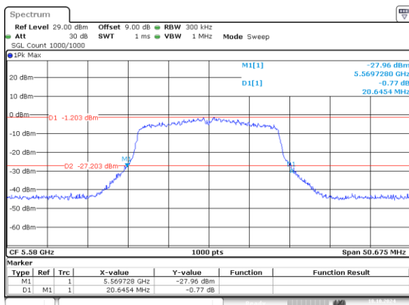
802.11n20_5580MHz_Chain 0 20.645MHz
