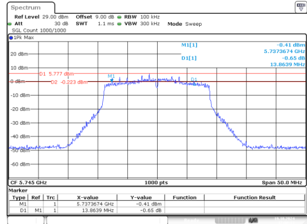
802.11n20_5745MHz_Chain 1 13.864MHz
