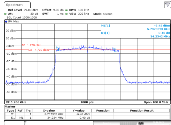
802.11ax40_5755MHz_RU_484/65_Chain 1 34.234MHz
