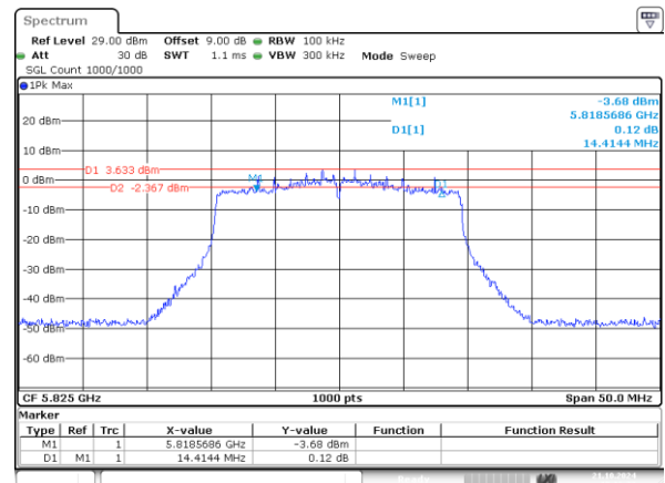
802.11ax20_5825MHz_RU_242/61_Chain 1 14.414MHz
