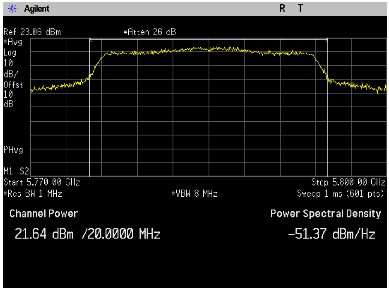
Figure 35: U-NII-3_5785MHz_Mid Ch_157_20MHz BW_n-mode_Output Power_Port 2.
