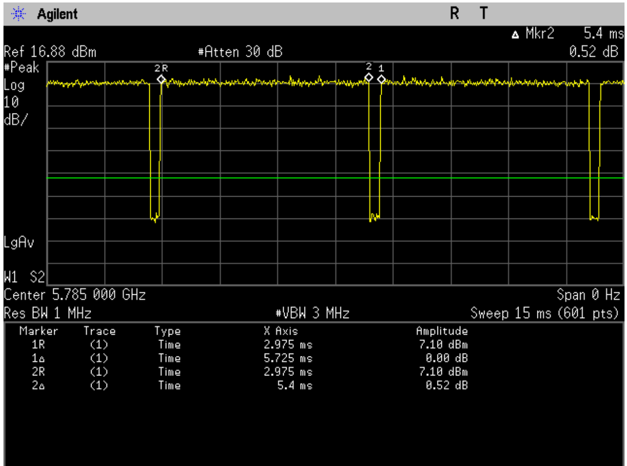
Figure 4: U-NII-3_5785MHz_Mid Ch_157_20MHz BW_ac-mode_Duty Cycle_Port 1.
