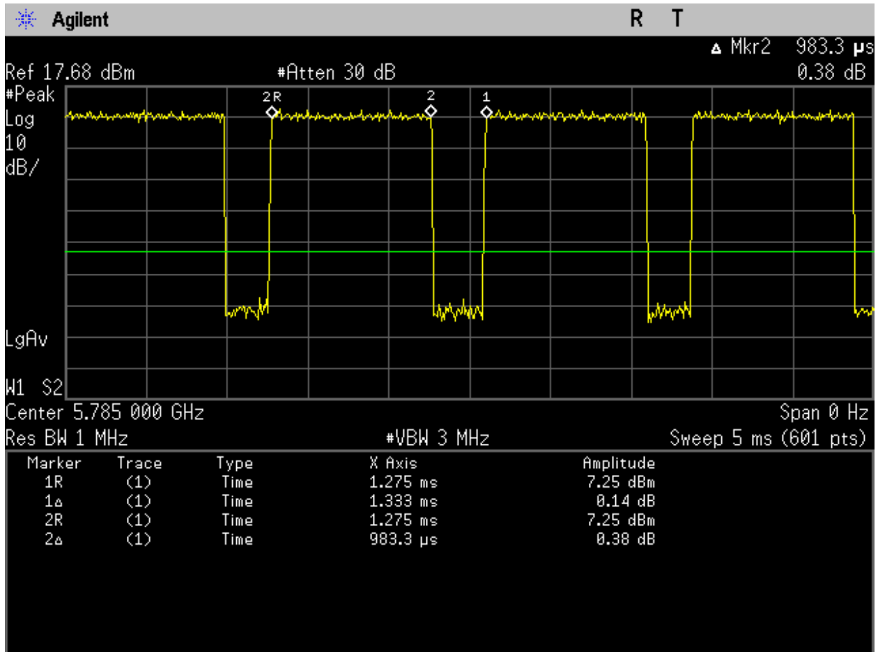
Figure 3: U-NII-3_5785MHz_Mid Ch_157_20MHz BW_a-mode_Duty Cycle_Port 1.
