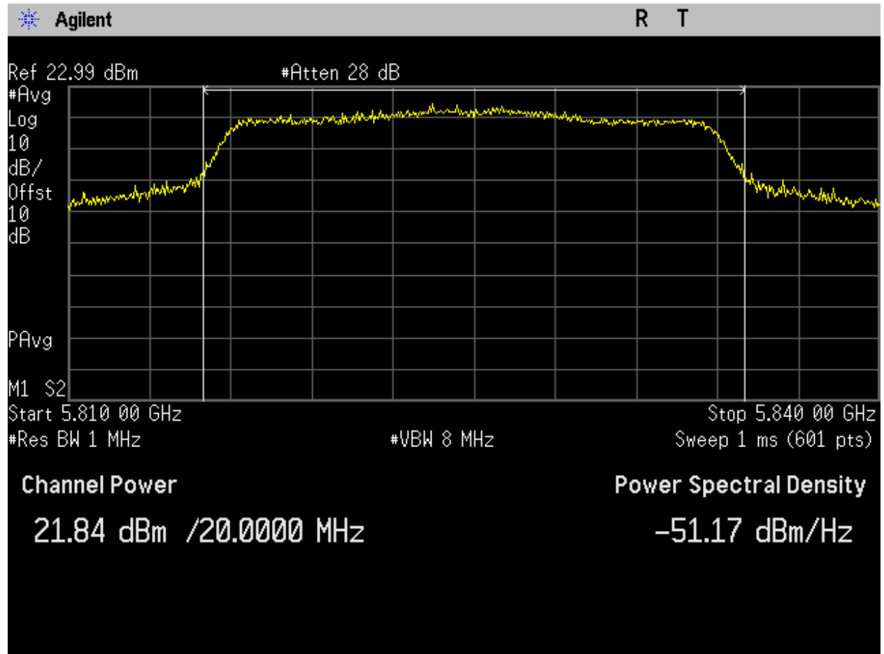
Figure 45: U-NII-3_5825MHz_High Ch_165_20MHz BW_ac-mode_Output Power_Port 2.
