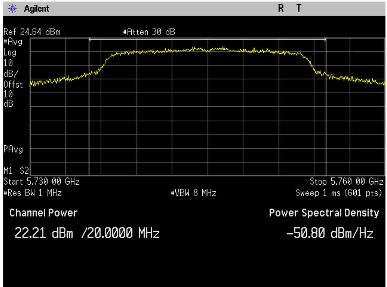
Figure 11: U-NII-3_5745MHz_Low Ch_149_20MHz BW_a-mode_Output Power_Port 2.
