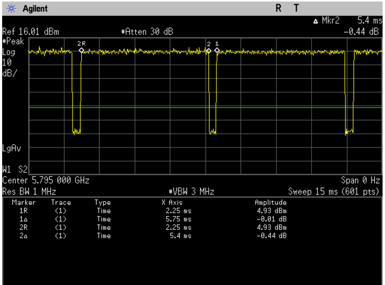
Figure 8: U-NII-3_5795MHz_High_Mid Ch_159_40MHz BW_ax-mode_Duty Cycle_Port 1.
