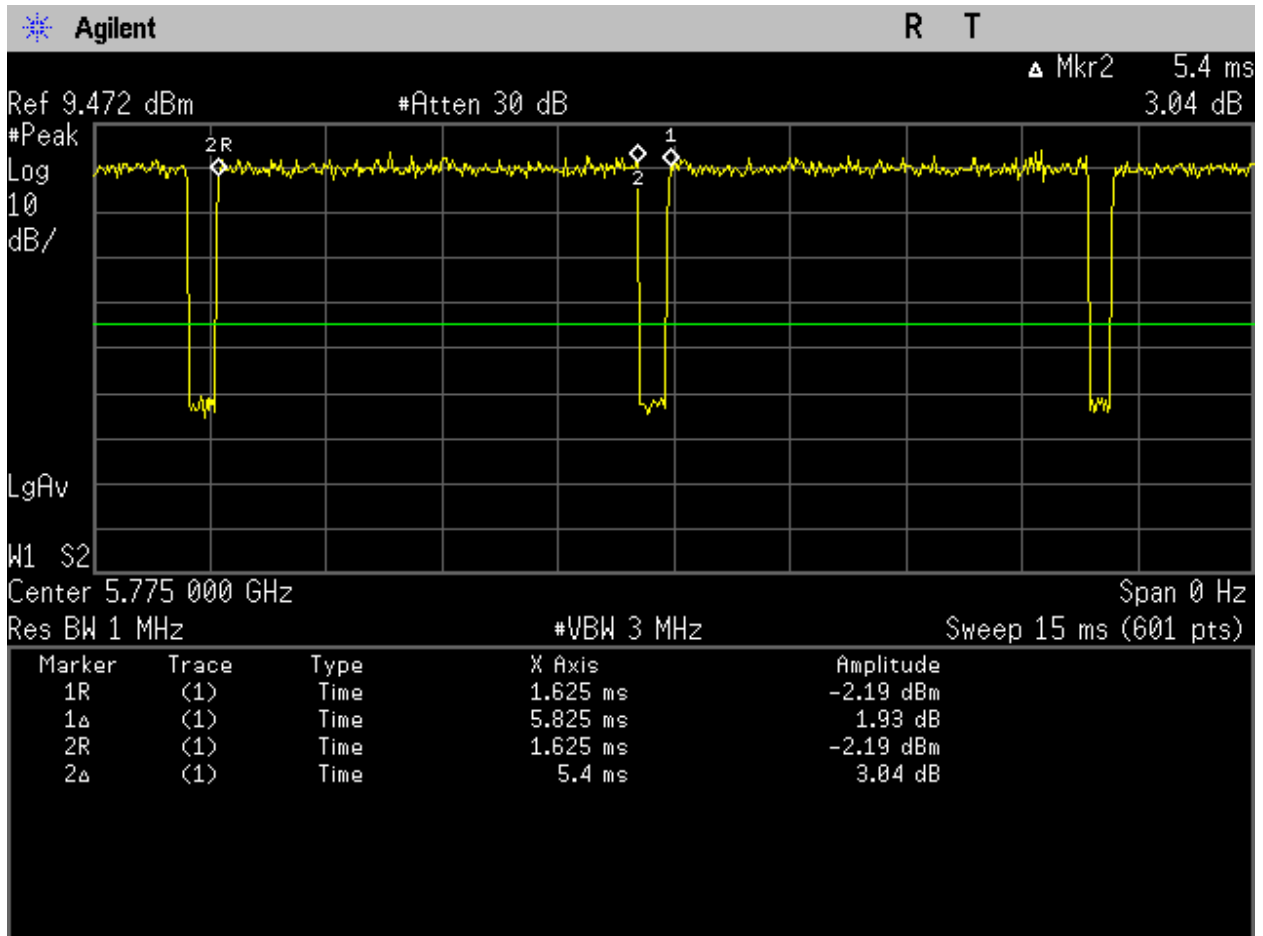
Figure 2: U-NII-3_5775MHz_High_Mid Ch_155_80MHz BW_ax-mode_Duty Cycle_Port 1.
