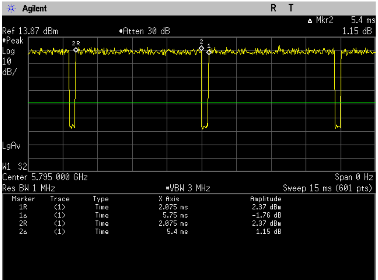
Figure 7: U-NII-3_5795MHz_High_Mid Ch_159_40MHz BW_ac-mode_Duty Cycle_Port 1.
