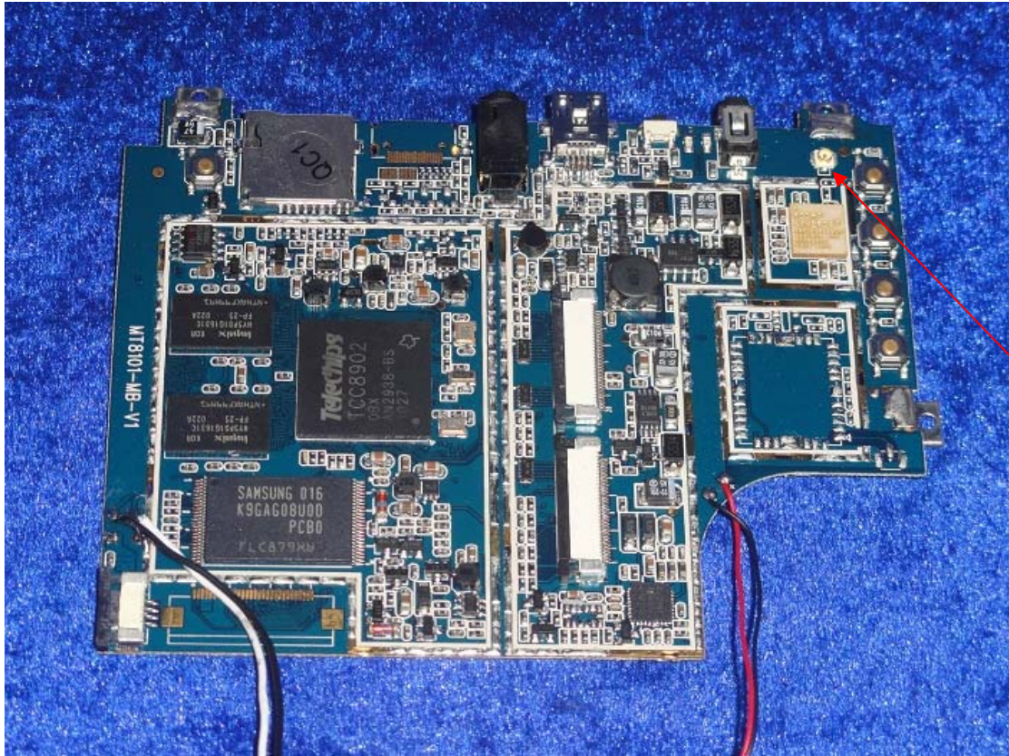
Antenna Connector
