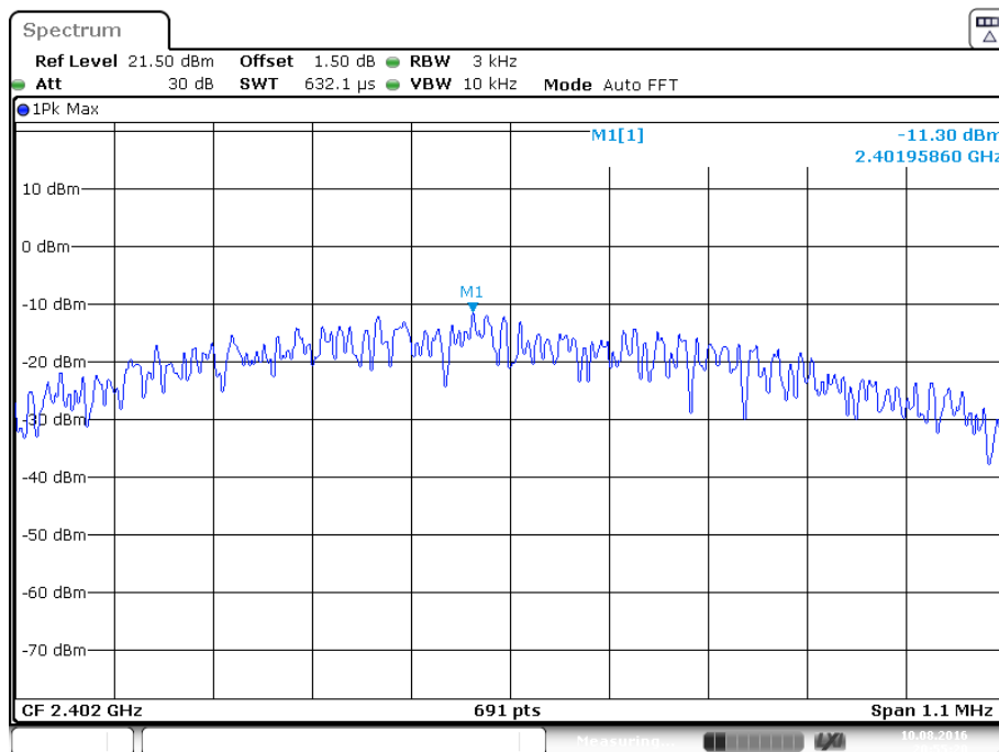
Power Spectral Density, BLE Low Channel
