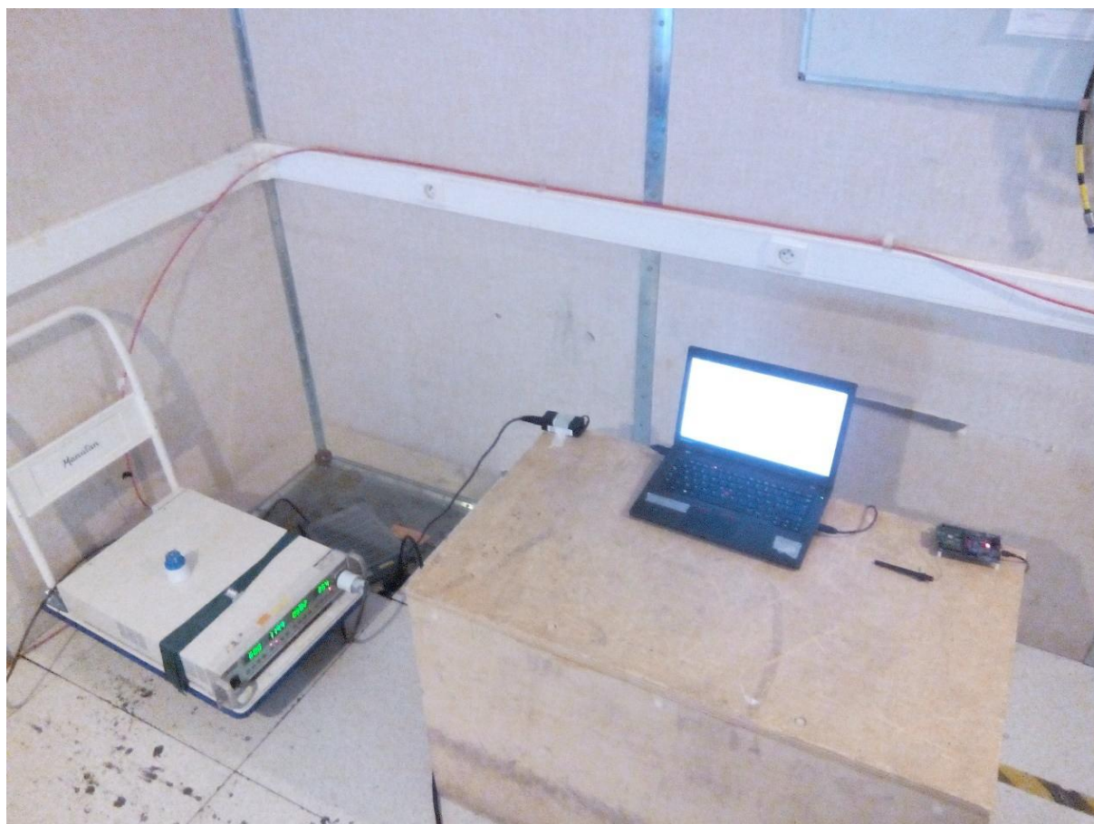
Conducted emission measurement setup
