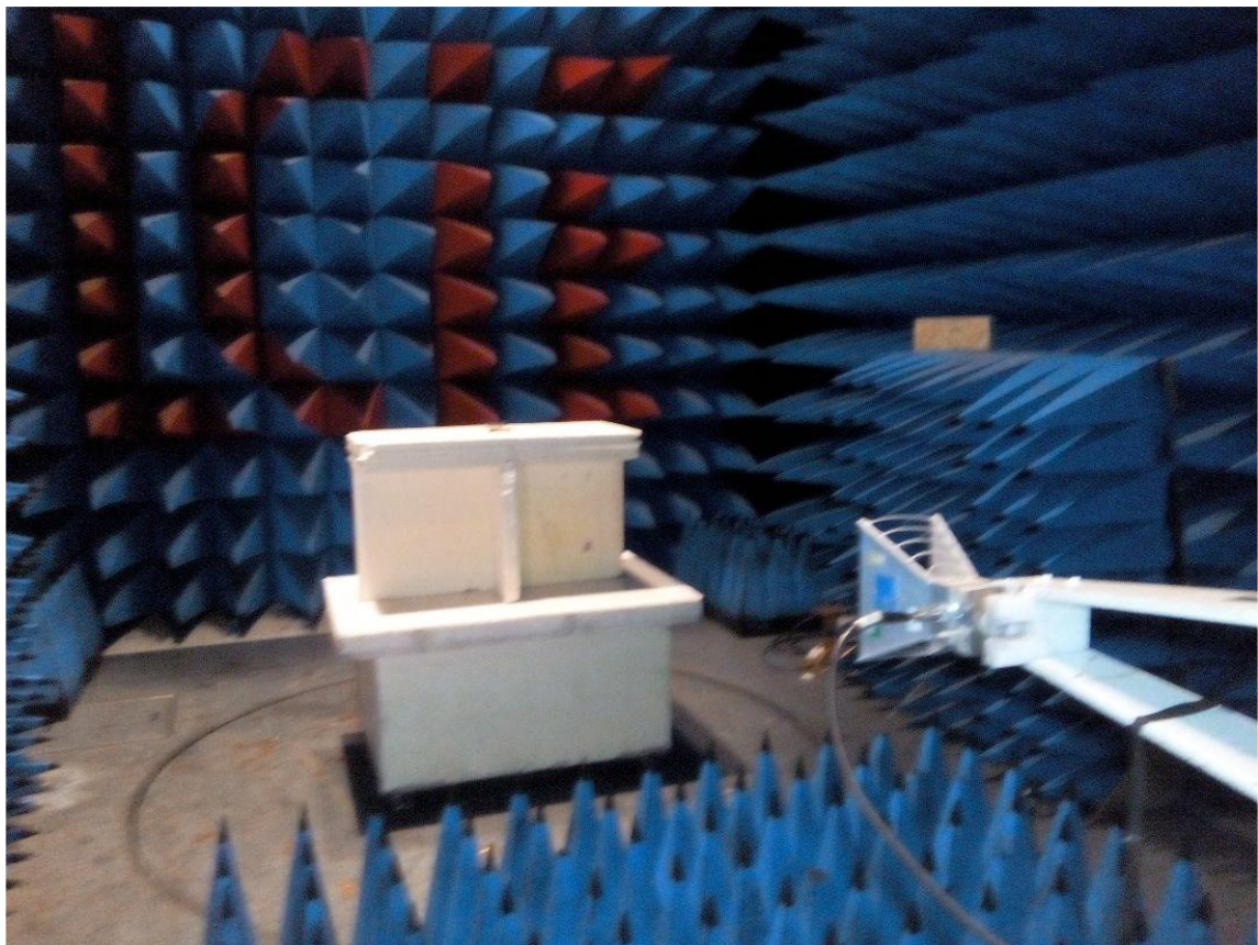
Radiated emissions measurements setup
